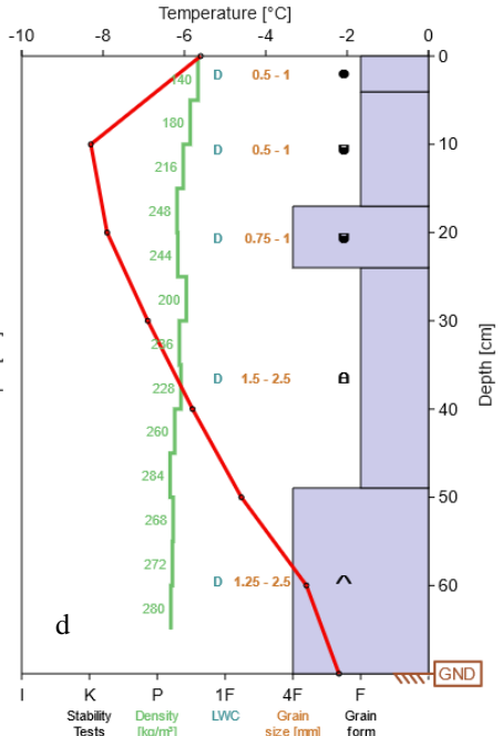
Figure 6. Examples of measured snow profiles in a forest clearing site during NoSREx missions: (a) M00 (17 March 2011) and in the winter of 2011-2012; b: M01 19 December 2011; c: M04 February 8, 2012; d: M09 March 8, 2012. Profiles include density (green line), temperature (red line), grain size (minimum-maximum ranges), grain type and hand hardness (vertical bars; K=knife, P=pencil, 1F=one finger, 4F=four fingers and F = fist). Hand hardness was not estimated on 17 March 2011.
