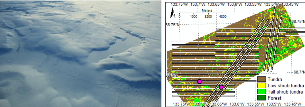
Figure 17. Aerial photograph (left) and land cover map of the Trail Valley Creek (TVC) research basin, overlaid by SnowSAR flight transects. Location of weather stations indicated by purple dots. Photograph courtesy of A. Coccia, Metasensing.
