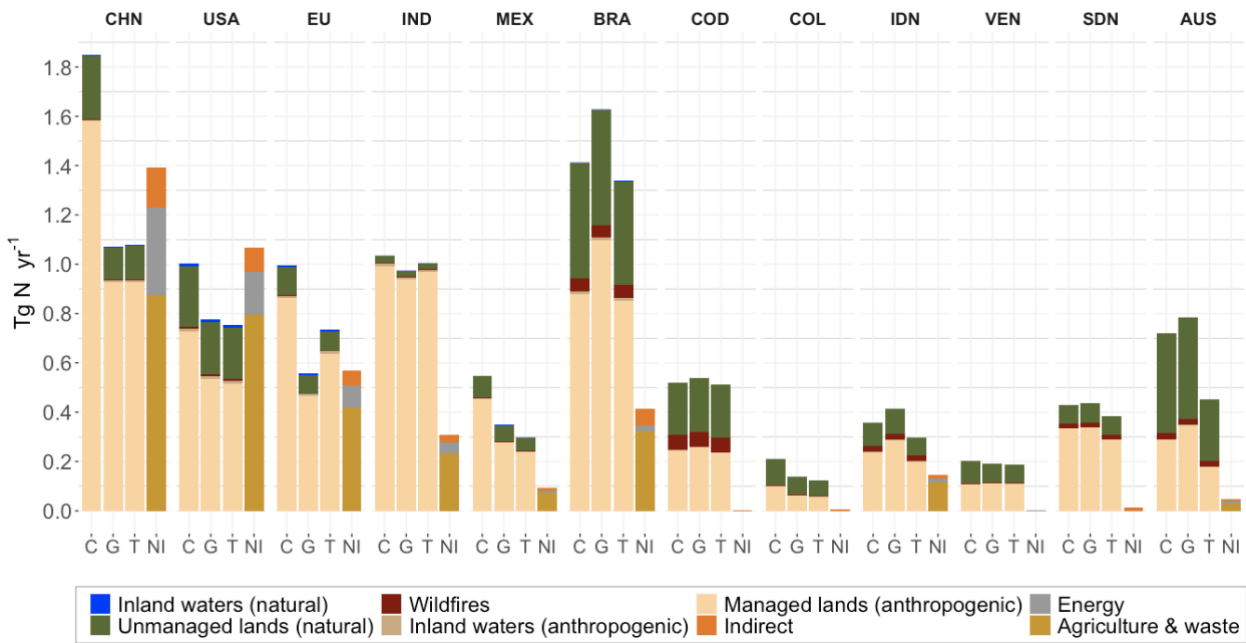
Figure 11: N 2 O emission fluxes in TgN yr -1 for CAMS (C), GEOS-Chem (G) and INVICAT (T) inversions compared to NGHGI (NI) data for 2010-2016. C, G, and T data correspond to the mean of fluxes from 2010 to 2016. NGHGI values represent the mean of available data for the same period. Anthropogenic rivers emissions are from Yao et al. (2019) and they are represented for information as part of managed land emissions, as they are captured by inversions (section 1). Natural river emissions are considered as the average of 1900-1910 (section 1) which are removed from total emissions of inversions. Data of wildfires correspond to GFEDv4 reported values for the period of interest (van der
