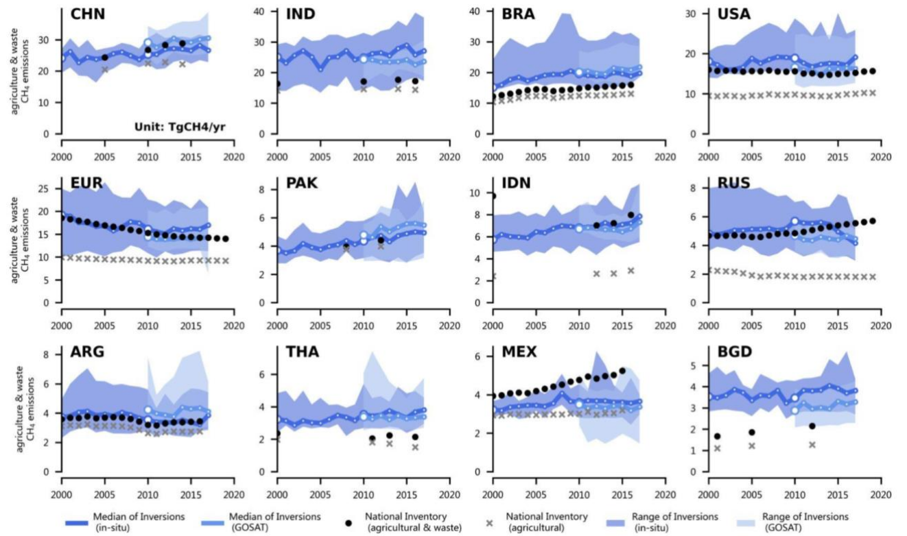
Figure 6: CH 4 emissions from agriculture and waste for the 12 largest emitters in this sector, China (CHN), India (IND), Brazil (BRA), United States (USA), EU27 & UK (EUR), Pakistan (PAK), Indonesia (IDN), Russia (RUS), Argentina (ARG), Thailand (THA), Mexico (MEX), and Bangladesh (BGD). The black dots denote the reported estimates from NGHGs from the agriculture and waste sector and the grey crosses denote NGHGs emissions from the agriculture sector only; the difference being the waste sector. Other lines, colors and symbols as Fig 4.
