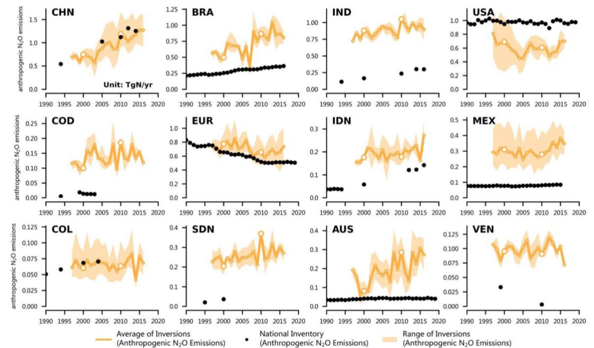
Figure 7: Anthropogenic N 2 O fluxes of the top 12 emitters: China (CHN), Brazil (BRA), India (IND), United States (USA), Democratic Republic of the Congo (COD), EU27 & UK (EUR), Indonesia (IDN), Mexico (MEX), Colombia (COL), Sudan (SDN), Australia (AUS), and Venezuela (VEN). The black dots denote the anthropogenic emissions from the UNFCCC national inventories. The thick orange lines denote the median of anthropogenic fluxes among N 2 O inversions (thick) and the light orange areas denote the maximum-minimum ranges of all inversions. COD NC3 report 2000-2010 but total emissions are inconsistent with sectoral emissions
