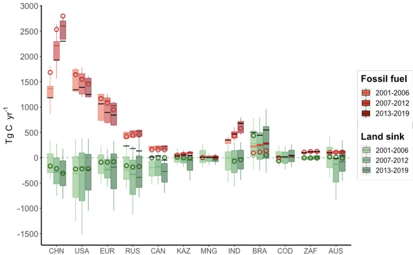
Figure 8: CO 2 fluxes for land sink, and fossil emissions. Box plots represent inversions for different time periods. Horizontal lines inside box plots denote median values for inversions. Vertical lines of box plots denote minimum and maximum values for selected time periods. Black horizontal lines symbolize net CO 2 fluxes (fossil fuel and cement emissions + land flux) for inversions. Circumferences represent the mean of UNFCCC NGHGI data available for each time period.
