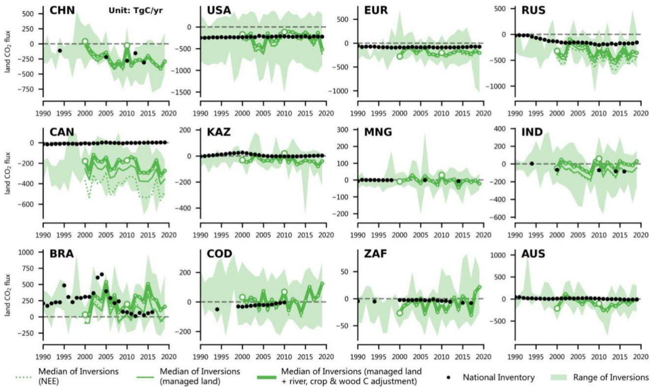
Figure 3: Net Ecosystem Exchange (NEE) CO 2 fluxes (TgC yr -1 ) from China (CHN), United States (USA), EU27 & UK (EUR), Russia (RUS), Canada (CAN), Kazakhstan (KAZ), Mongolia (MNG), India (IND), Brazil (BRA), Democratic
