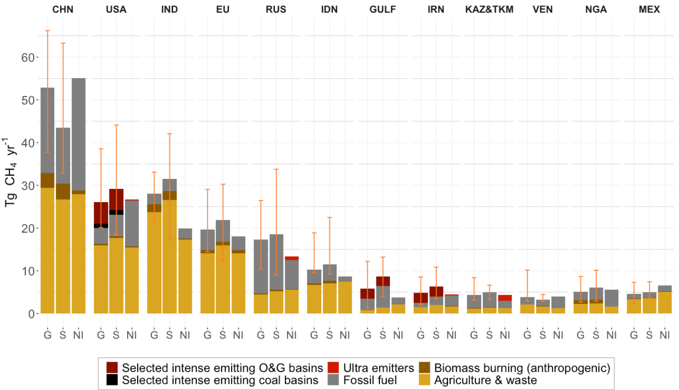
Figure 10: Total Anthropogenic CH 4 emissions from in-situ (S) and GOSAT (G) inversions compared to NGHGI (NI). S and G data correspond to the mean of inversion medians from the last 5 years of the available inversion data (2013 to 2017). Error bars denote minimum and maximum values for S and G inversions. NGHGI values represent the mean
