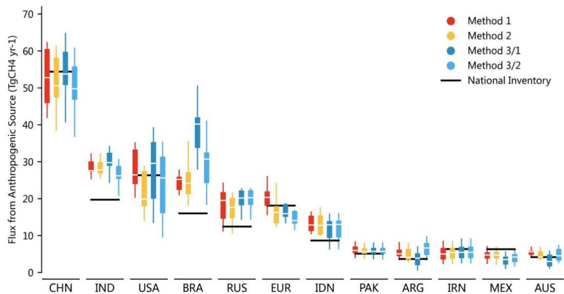
Figure 9: Interquartile and min, max of Total Anthropogenic CH 4 emissions separated using different methods based on GOSAT inversions in the 2010s and the total anthropogenic CH 4 emissions from NGHGs. For each region, vertical boxes show median, interquartile range, and min/ max of the GOSAT inversions. Each color represents a different separation approach, as defined in section 1.4. Black lines denote the average of Total Anthropogenic CH 4 emissions from national inventories in the 2010s with available reported years.
