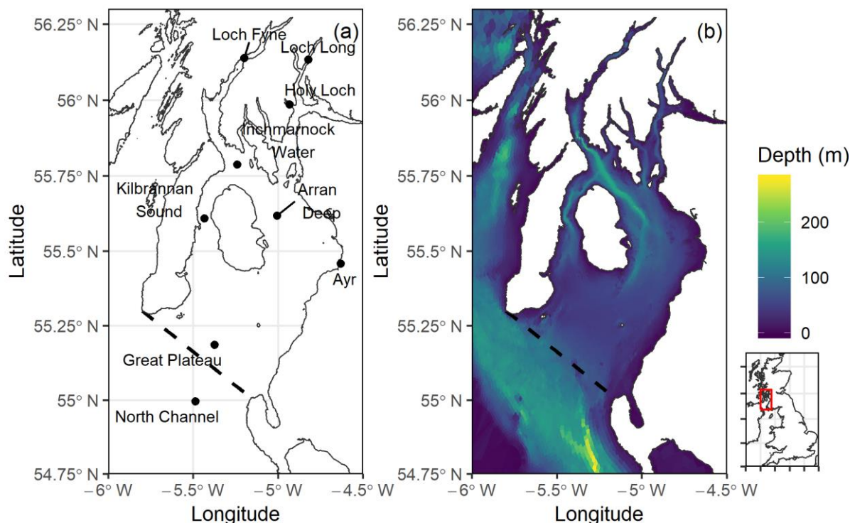
105 Figure 1 Maps of the Firth of Clyde showing (a) locations referred to in text and, (b) bathymetry mapped over an unstructured grid. Seabed depth is shown in metres and the dashed line shoes the outer geographical limits of the Firth of Clyde. The location of the Firth of Clyde on the west coast of Scotland is shown inset. Bathymetry data source: Sabatino et al. (2016).
