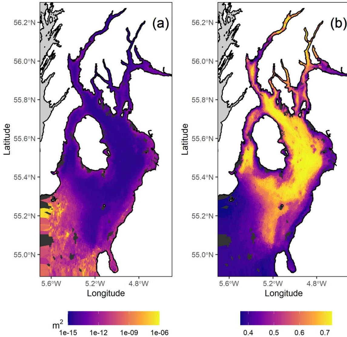
465 Figure 13 Mapped predictions of (a) sediment permeability and (b) sediment porosity in the Firth of Clyde. Seabed consisting of hard substrate or sediments with a predicted permeability greater than 1 \times 10^{-6} \text{ m}^2 are shown as black areas. Permeability predictions were generated from the map of percentage mud content in seabed sediments. Porosity was predicted from the map of median grain size in the Firth of Clyde.
