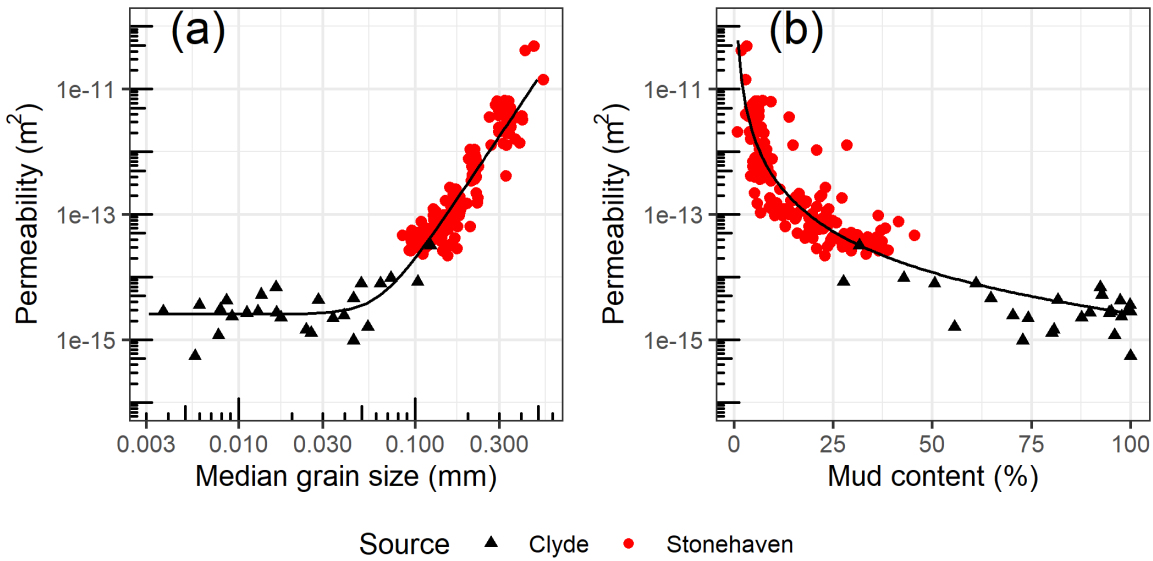
440 Figure 11 Relationship between sediment permeability ( m^2 ) and (a) median grain size (mm) and (b) % mud content for measurements from the Firth of Clyde (black triangles) and samples from the North Sea analysed by Serpetti et al. (2016) (red points). Fitted relationships for the combined data are shown by a solid line. Note \log_{10} scale.
