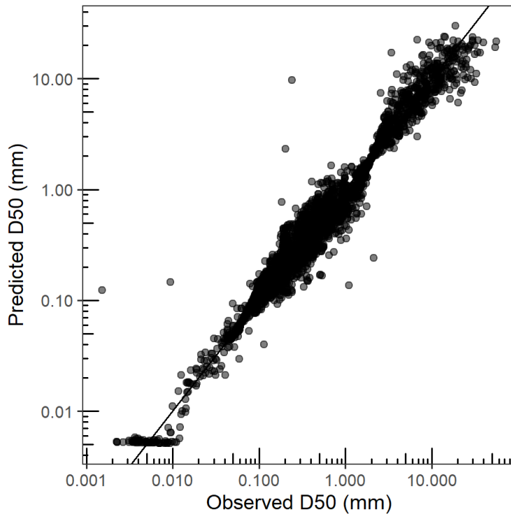
425 Figure 9 Leave-one-out cross-validation results showing predicted and measured values of median grain size for a dataset comprising samples collected from cruises in the Firth of Clyde in April and October 2017 and supplemented with data from the North Sea, Celtic Sea and English channel collected by CEFAS and MSS (n = 3244). Note \log_{10} scale.
