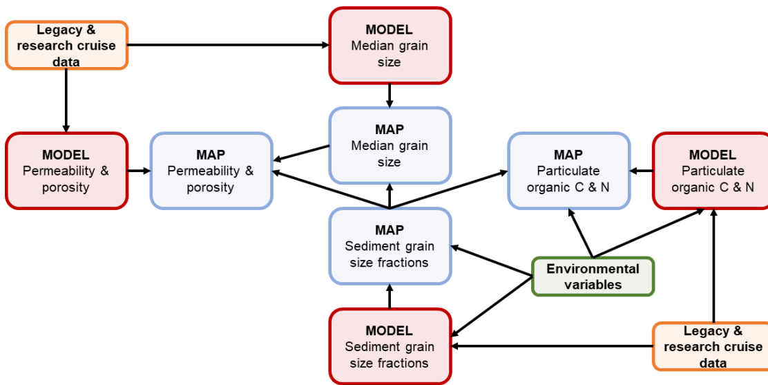
295 Figure 5 Illustration of the workflow described in this chapter. Legacy and research cruise data (orange boxes) were used in conjunction with mapped environmental variables (green boxes) to fit models of seabed sediment grain size and geotechnical properties and organic carbon and nitrogen content. Full-coverage quantitative maps of these properties (blue boxes) were generated by using mapped environmental variables and sedimentary maps created earlier in the workflow as the substrate from which to generate predictions from the fitted models.
