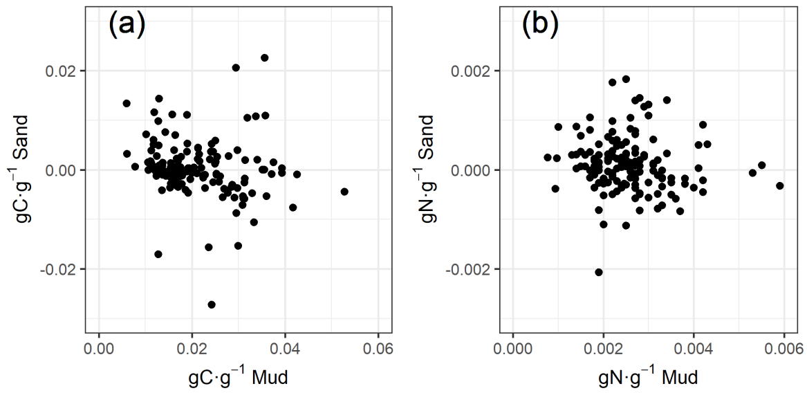
615 Figure A.1 Relationship between (a) the mass fraction of organic carbon in mud ( \text{gC g}^{-1} \text{ mud} ) and in sand ( \text{gC g}^{-1} \text{ sand} ) and (b) the mass fraction of organic nitrogen in mud ( \text{gN g}^{-1} \text{ mud} ) and in sand ( \text{gN g}^{-1} \text{ sand} ) for sediment collected from the North Sea by CEFAS and the Clyde Sea.
