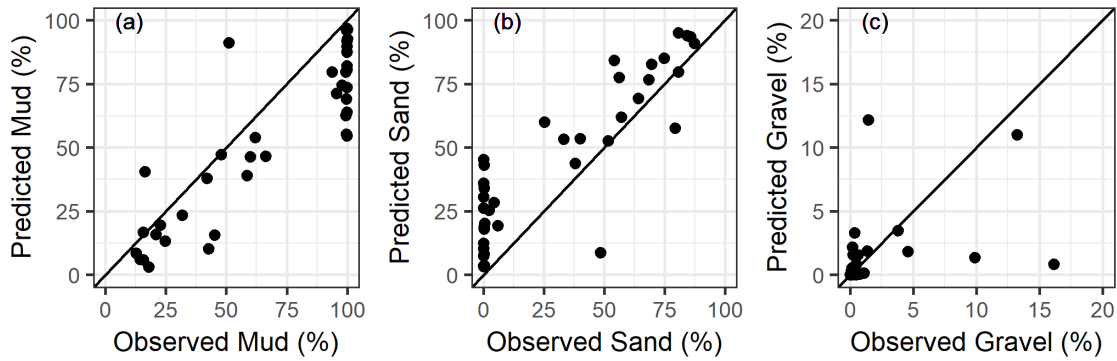
Figure 8 Comparison of predicted and observed percentages of (a) mud, (b) sand and (c) gravel in Firth of Clyde seabed sediments. Observation data are recent measurements carried out in 2017 that were not used during model fitting. Predictions were generated from the sediment maps presented in Fig. 7. This is therefore an independent test of model and map predictive performance.
