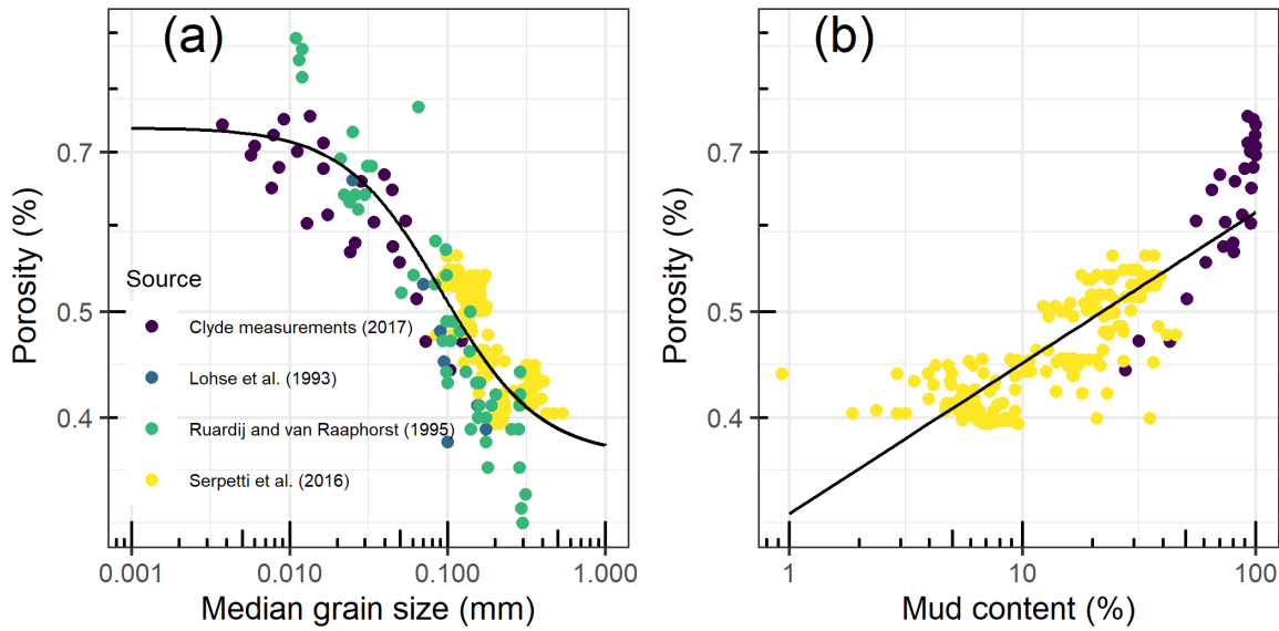
Figure 12 Relationship between sediment porosity (%) and (a) median grain size (mm) and (b) % mud content for measurements for the top 10 cm seabed sediment on a log 10 scale.
