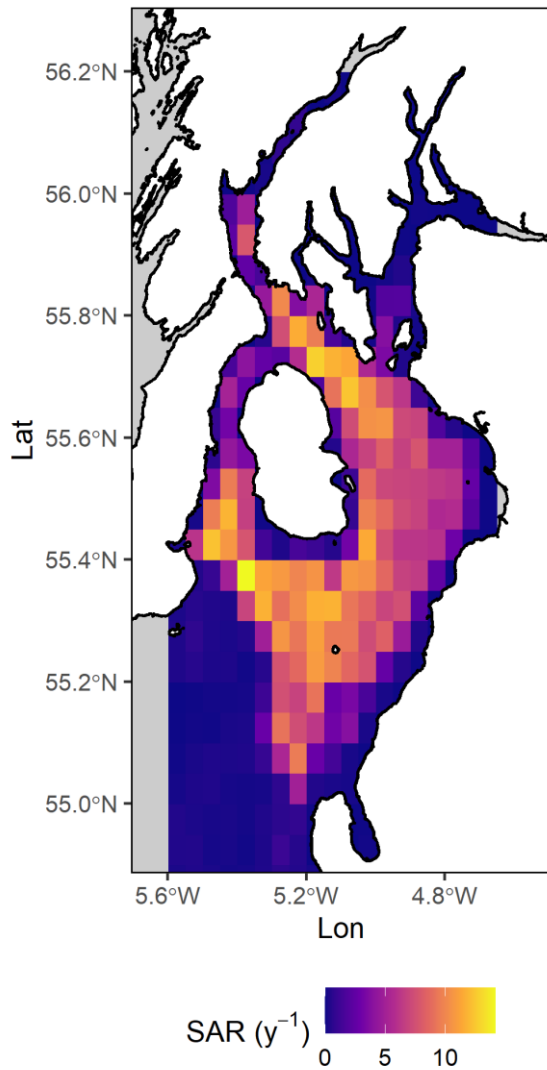
190 Figure 4 Mean annual swept area ratio (SAR) for the years 2009 - 2016. Spatial distribution of seabed abrasion pressure from fishing vessels with an overall length greater than 12 m. Areas where no data is available are shown in grey.
