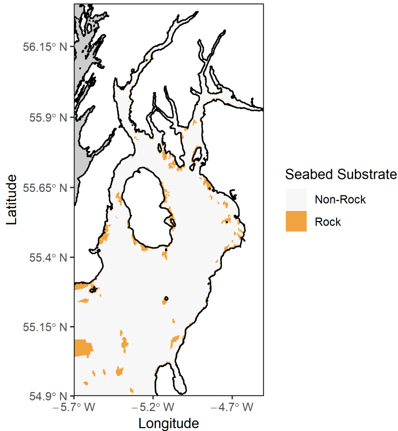
400 Figure 6 Distribution of hard substrate in the Firth of Clyde according to BGS data layers and Random Forest model predictions generated for areas lacking data - the inner Firth of Clyde and sea lochs.
