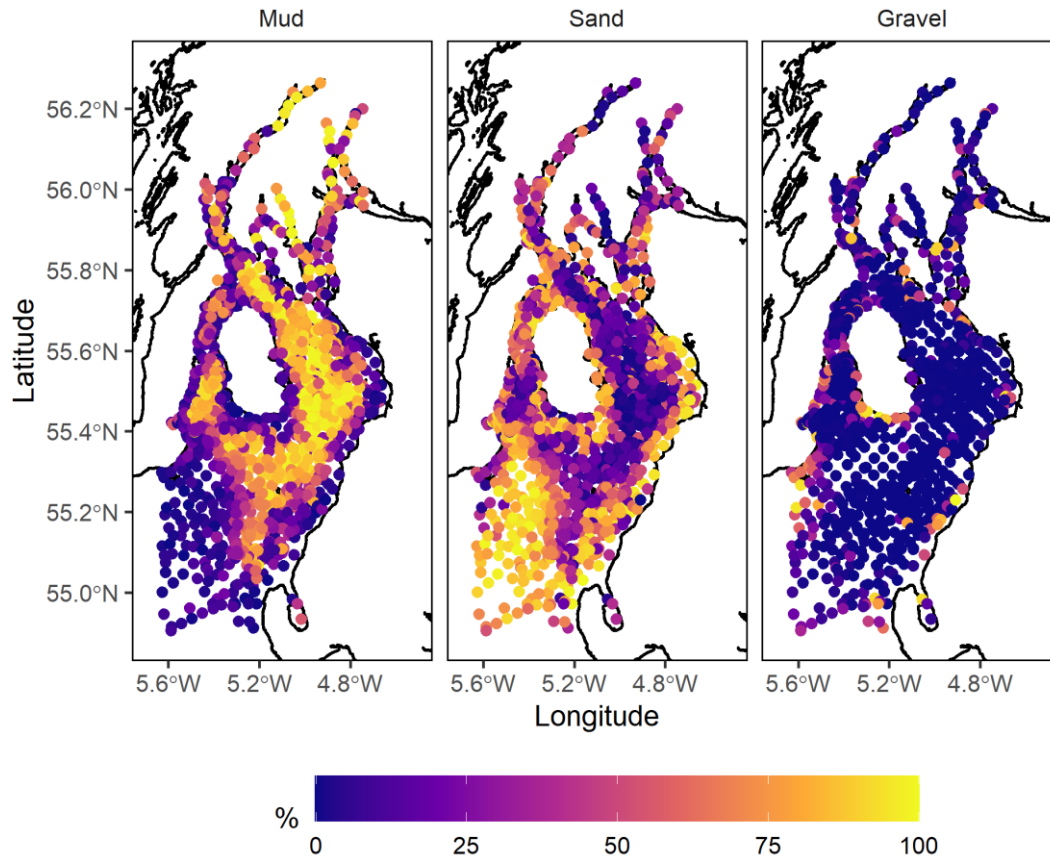
135 Figure 2 Locations sampled by BGS, MSS and SEPA for the measurement of percentage mud, sand and gravel in seabed sediments in the Firth of Clyde.
