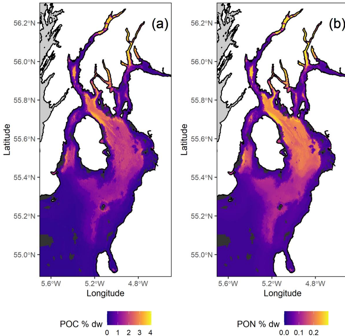
Figure 15 Maps of predicted % dry weight sediment (a) organic carbon and (b) organic nitrogen content within the top 10 cm of seabed in the Firth of Clyde.
