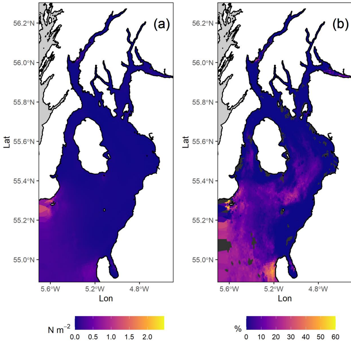
470 Figure 14 Mapped predictions of (a) annual mean bed shear stress and (b) sediment mobility in terms of the annual percentage of 475 time that sediment motion occurs in the Firth of Clyde.
