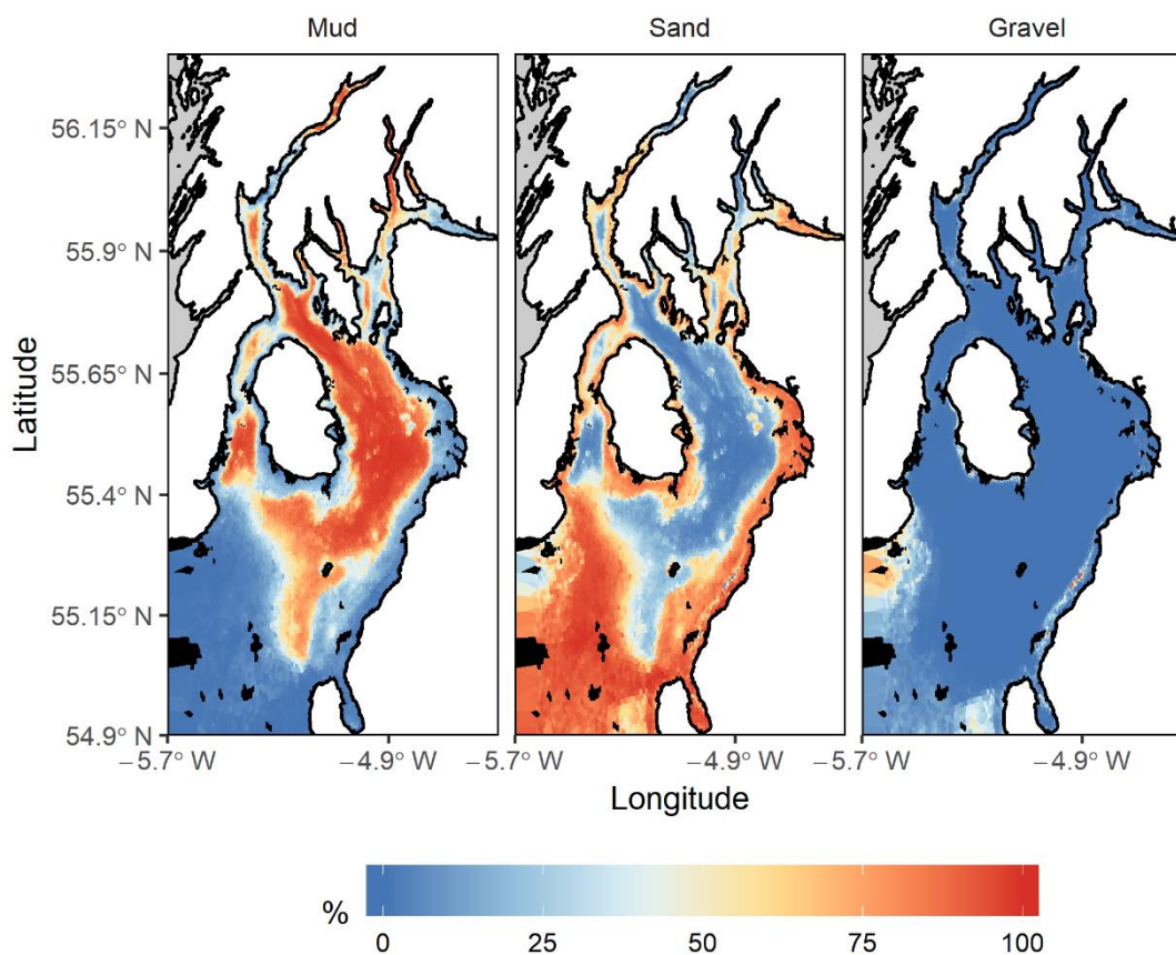
Figure 6 Mapped percentages of mud, sand and gravel within Firth of Clyde sediments predicted from Random Forest models.
