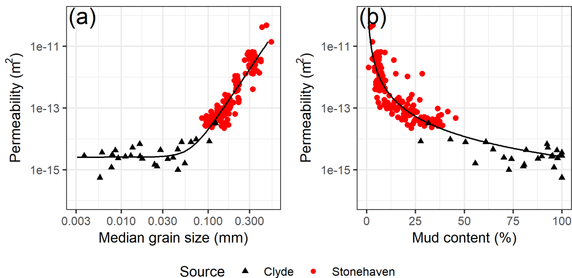
370 Figure 10 Relationship between sediment permeability ( m^2 ) and (a) median grain size (mm) and (b) % mud content for measurements from the Firth of Clyde (black triangles) and samples from the North Sea analysed by Serpetti et al. (2016) (red points). Fitted relationships for the combined data are shown by a solid line. Note \log_{10} scale.
