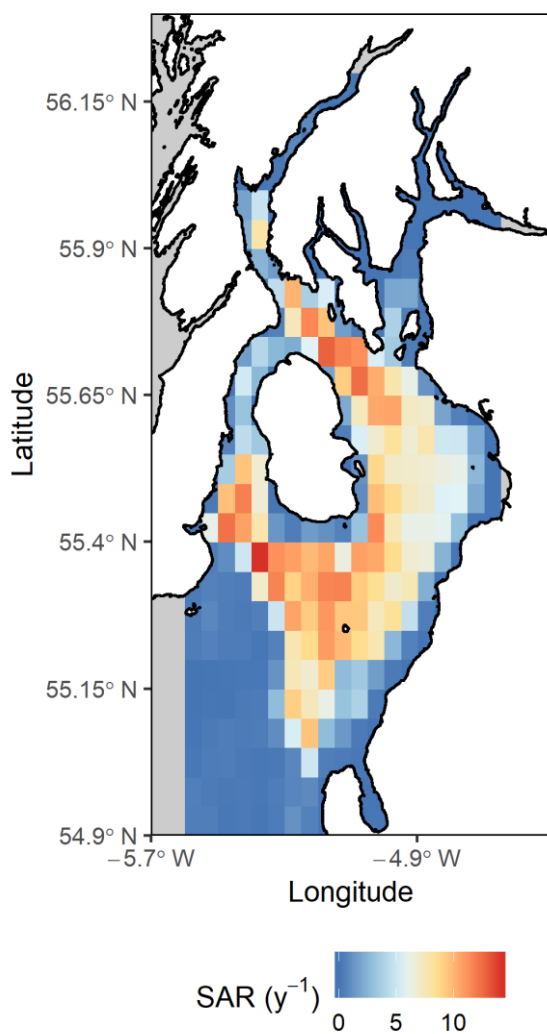
175 Figure 4 Mean annual swept area ratio (SAR) for the years 2009 - 2016. Spatial distribution of seabed abrasion pressure from fishing vessels with an overall length greater than 12 m. Areas where no data is available are shown in grey.
