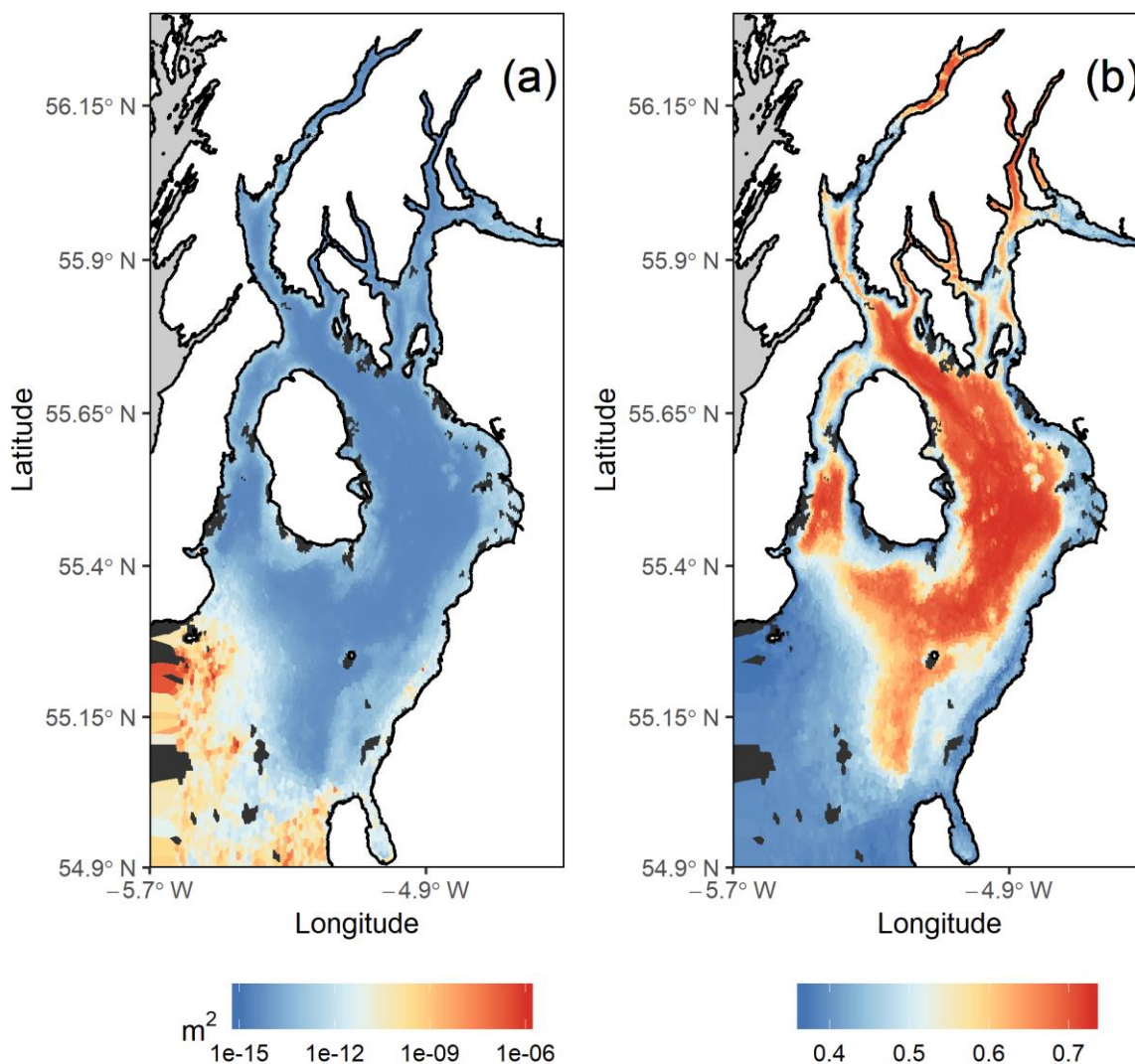
390 Figure 12 Mapped predictions of (a) sediment permeability and (b) sediment porosity in the Firth of Clyde. Seabed consisting of hard substrate or sediments with a predicted permeability greater than 1 \times 10^{-6} \text{ m}^2 are shown as black areas. Permeability predictions were generated from the map of percentage mud content in seabed sediments. Porosity was predicted from the map of median grain size in the Firth of Clyde.
