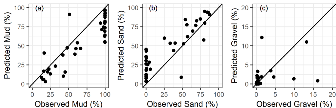
Figure 7 Comparison of predicted and observed percentages of (a) mud, (b) sand and (c) gravel in Firth of Clyde seabed sediments.
