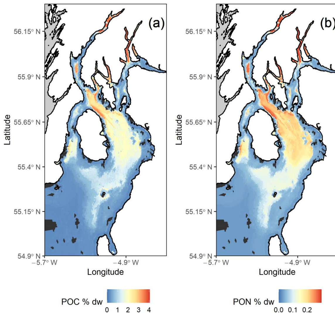
Figure 14 Maps of predicted % dry weight sediment (a) organic carbon and (b) organic nitrogen content within the top 10 cm of seabed in the Firth of Clyde.
