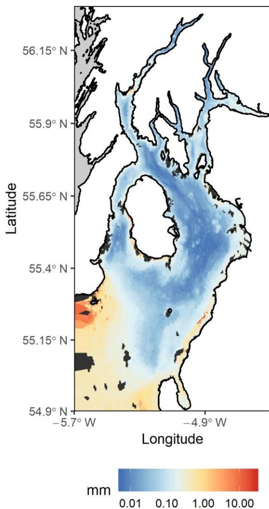
Figure 9 Mapped predictions of median grainsize for seabed sediments in the Firth of Clyde.
