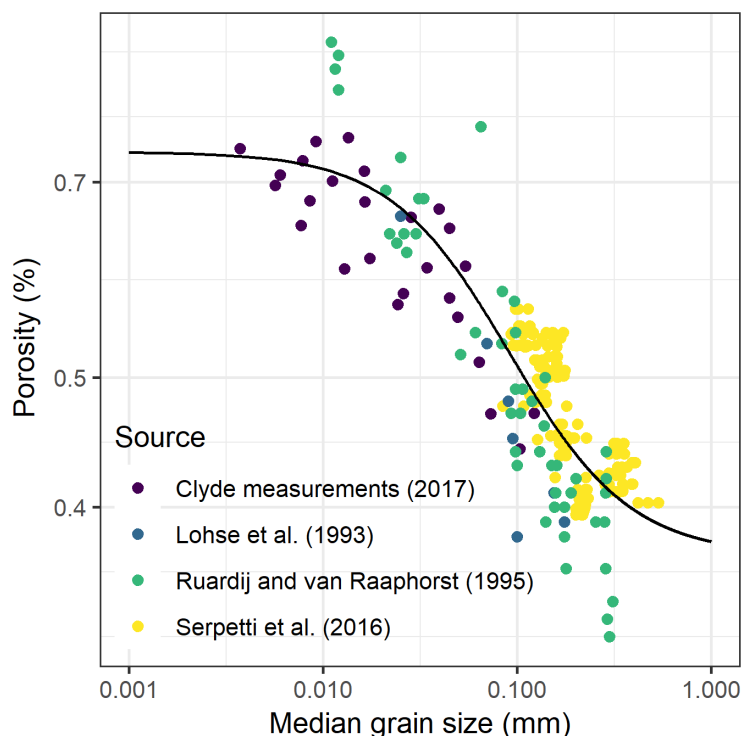
380 Figure 11 Relationship between sediment porosity (%) and median grain size (mm) for the top 10 cm seabed sediment on a log 10 scale.
