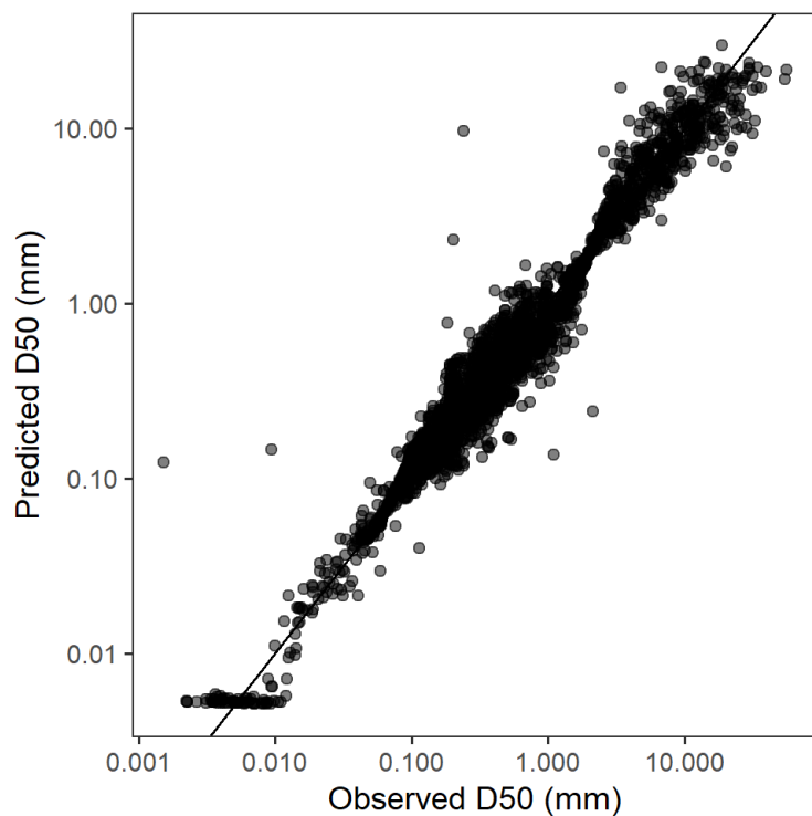
Figure 8 Leave-one-out cross-validation results showing predicted and measured values of median grain size for a dataset comprising samples collected from cruises in the Firth of Clyde in April and October 2017 and supplemented with data from the North Sea, Celtic Sea and English channel collected by CEFAS and MSS (n = 3244). Note \log_{10} scale.
