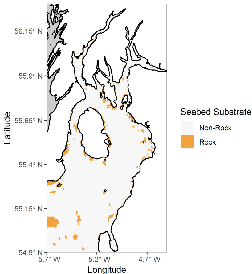
335 Figure 5 Distribution of hard substrate in the Firth of Clyde according to BGS data layers and Random Forest model predictions generated for areas lacking data - the inner Firth of Clyde and sea lochs.
