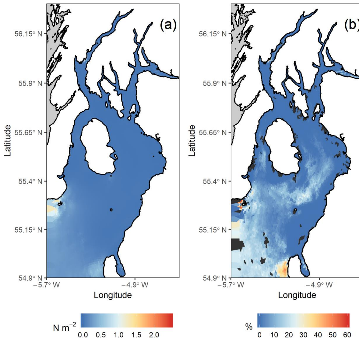
Figure 13 Mapped predictions of (a) annual mean bed shear stress and (b) sediment mobility in terms of the annual percentage of time that sediment motion occurs in the Firth of Clyde.
