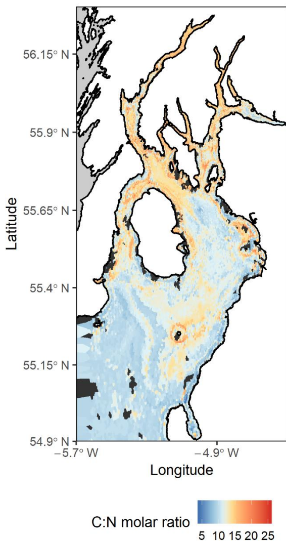
Figure 15 Variation in the predicted organic carbon-nitrogen molar ratio.
