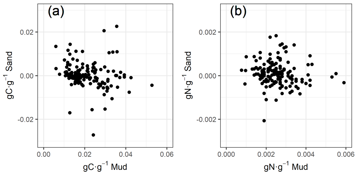
Figure A.1 Relationship between (a) the mass fraction of organic carbon in mud ( \text{gC g}^{-1}\text{ mud} ) and in sand ( \text{gC g}^{-1}\text{ sand} ) and (b) the mass fraction of organic nitrogen in mud ( \text{gN g}^{-1}\text{ mud} ) and in sand ( \text{gN g}^{-1}\text{ sand} ) for sediment collected from the North Sea by CEFAS and the Clyde Sea.
