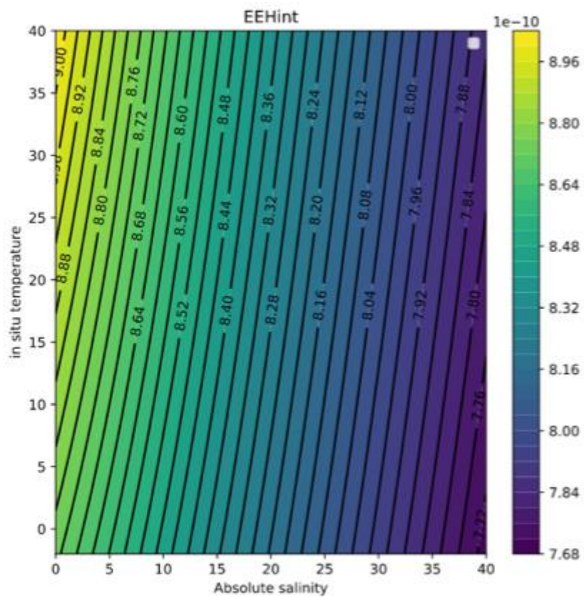
Figure B1: Integrated expansion efficiency of heat (IEEH) dependence on in situ temperature and absolute salinity at 1 atm in mm/J-1.
