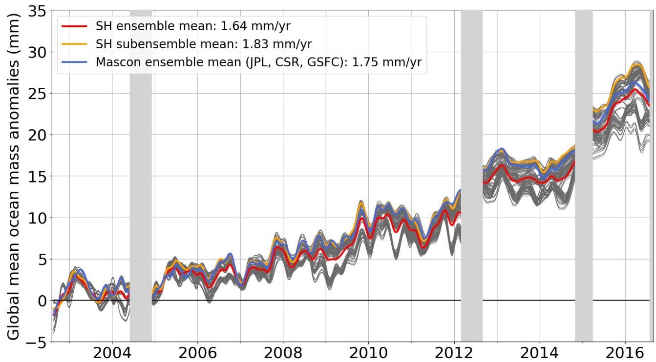
555 Figure A1: Comparison of global mean ocean mass changes from satellite gravimetry based on spherical harmonics solutions (LEGOS ensemble V1.4, in grey) and mascon solutions over August 2002-August 2016 for the global ocean. The mean of the full spherical harmonic ensemble is shown in red. The mean of the spherical harmonic ensemble subset consistent with mascons is shown in orange. The mean of the three mascon solutions considered in this study is shown in blue.
