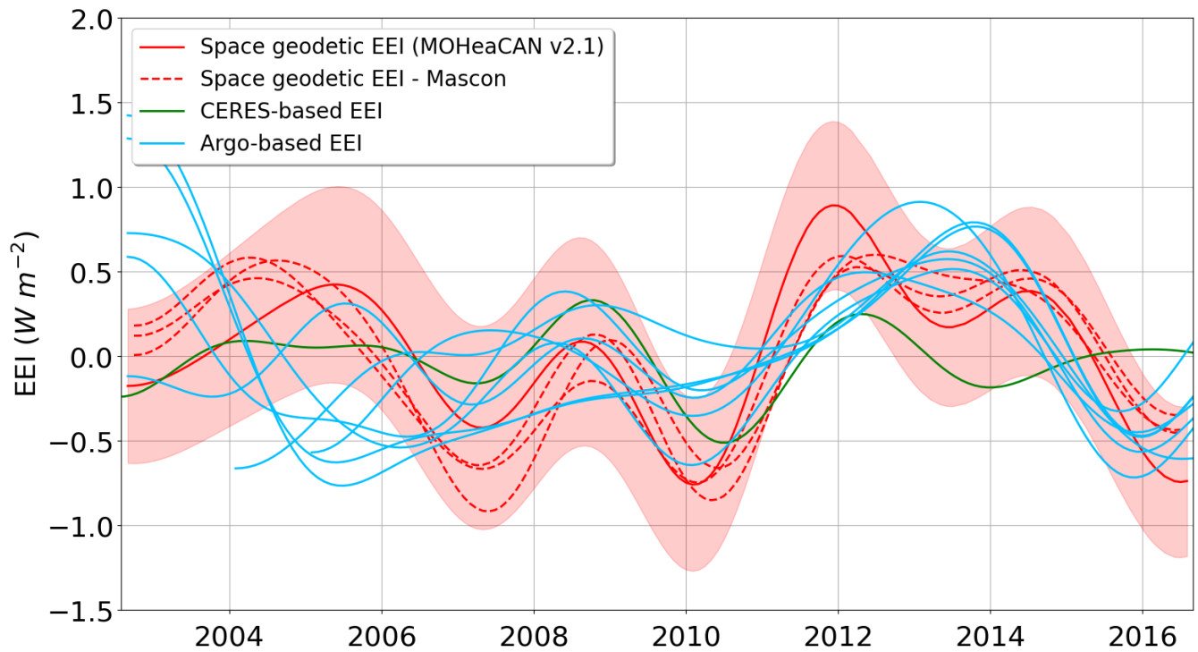
875 Figure 7: Interannual variations of Earth energy imbalance (EEI) time series. Mean and trend values have been removed for each time series and a filter has been applied to remove signals lower than 3 years. Red lines correspond to space geodetic estimates where estimates based on mascon ocean mass are represented in dash lines and MOHeaCAN v2.1 is represented by mean value (solid red) and the uncertainty at 1-sigma (shaded areas). Green line corresponds to CERES-based estimates and blue lines to the Argo-based estimates.
