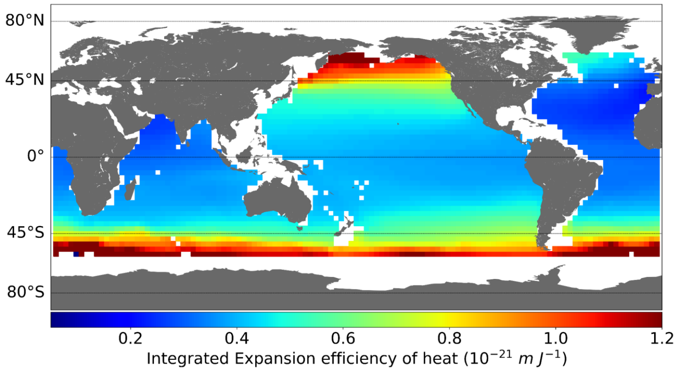
850 Figure 1: Integrated Expansion Efficiency of Heat (EEH) coefficients ( m J^{-1} ) at regional scale (3x3 degrees). See text.
