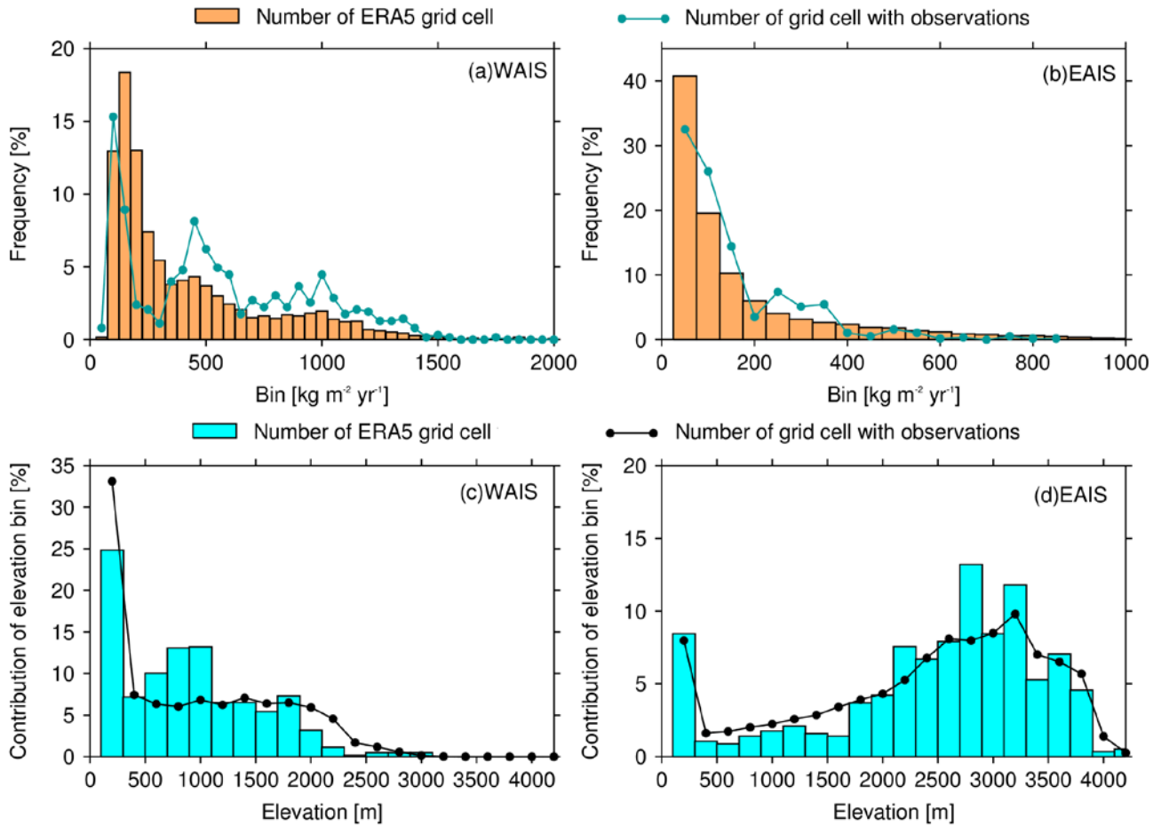
810 Figure 6 Relative frequency of ERA5 P-E field data and gridded averaged records from the multi-year averaged SMB subdatabase, with a bin range of 50 \text{ kg m}^{-2} \text{ yr}^{-1} on (a) the West Antarctic Ice Sheet (WAIS) and (b) the East Antarctic Ice Sheet (EAIS). ERA5 field data are bilinearly interpolated over a 30\text{km} Cartesian grid. We average SMB for each 30\times 30 \text{ km} grid cell (values from points located in the same grid cell are averaged), and then number of grid cells in each bin are calculated. The contribution of the area of elevation bin for ERA5 grid cells containing measurements, and entire elevation range to (c) the WAIS and (d) the EAIS. The 200\text{m} elevation bins are used.
