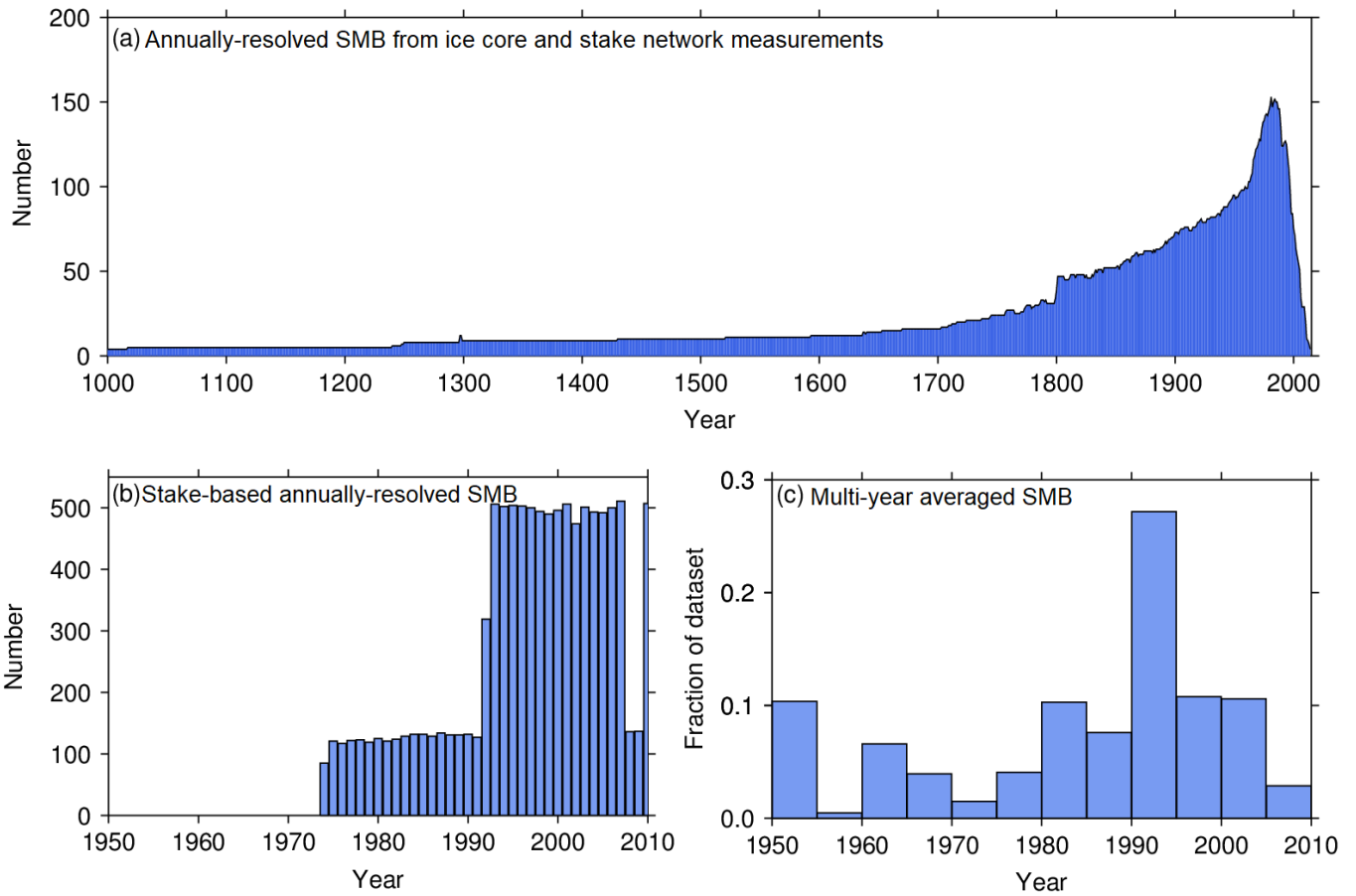
765 Figure 3: (a) Availability of records excluding the stake measurements along the traverse from Syowa Station to Dome F in the annual resolved SMB sub-database over time during the past 1000 years. (b) Time coverage of the stake measurements along the traverse from Syowa Station to Dome F. (c) Histograms indicating the date taken of the multi-year averaged SMB subdataset only including ice core and stake measurements.
