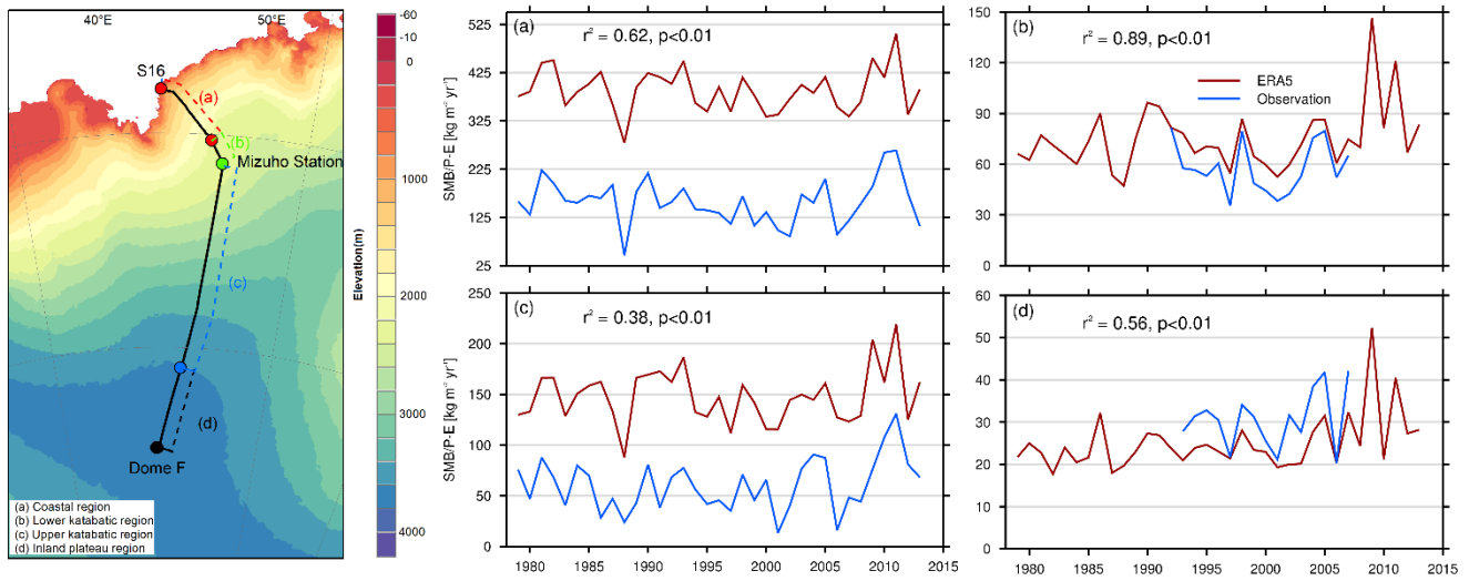
835 Figure 9: The left map showing the locations of stake measurements along the traverse between Syowa Station and Dome F, and the regional boundaries. The right four charts showing the comparison of the inter-annual variability in spatially-averaged stake measurements and snow accumulation simulated by ERA5 for (a) the coastal region, (b) lower katabatic region, (c) upper katabatic region, and (d) inland plateau region.
