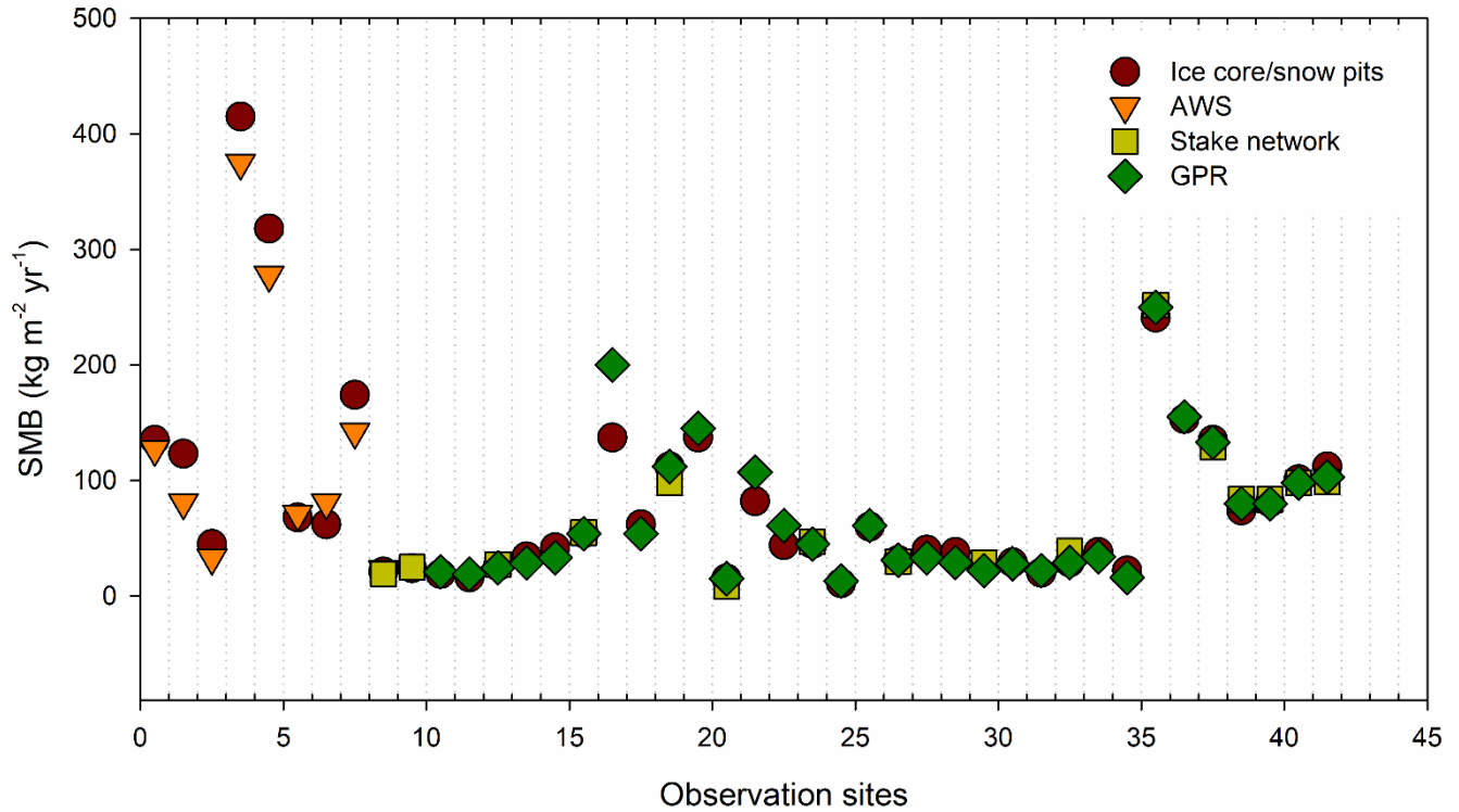
Figure 4: Inter-comparison between different types of SMB measurements including AWS, snow pit/ice core and GPR at 42 locations. They are mainly distributed near Talos Dome, along a transect from Terra Nova Bay to Dome C, on the western Dronning Maud Land, and at Dome F and Dome A.
