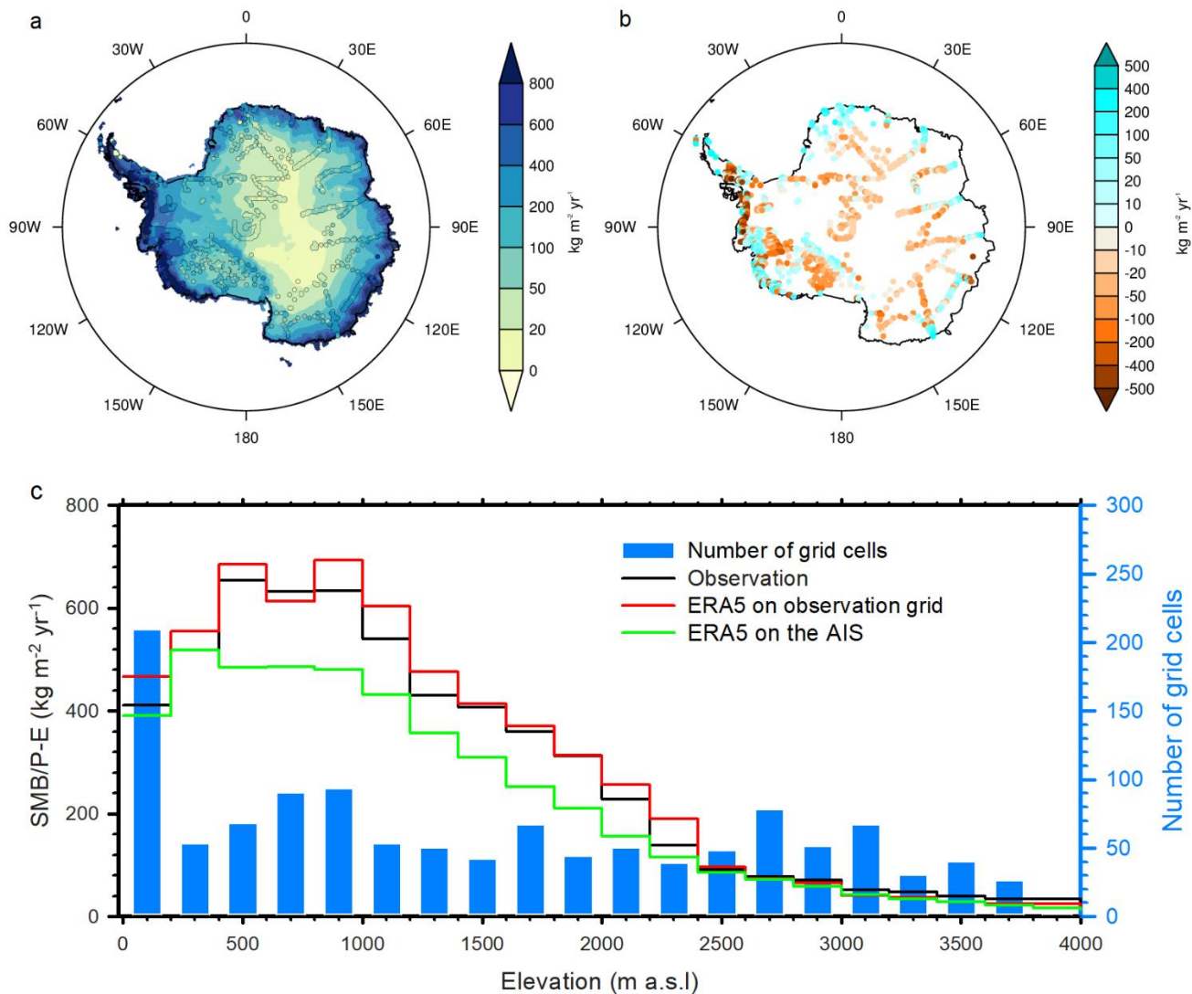
Figure 7: (a) Spatial distribution of ERA5 mean precipitation minus evaporation (approximated as SMB) for the period 1979–2018, and multi-year mean SMB measurements averaged on ERA5 grid cells (30km×30km). (b) ERA5 minus observed SMB averaged on the ERA5 grid cells, (c) Multi-year averaged observations and ERA5 simulations, binned in 200 m elevation intervals. The number of ERA5 grid cells with in situ measurements in each elevation bin is shown by the blue line (right axis). Red lines denote SMB averaged by ERA5 for grid cells including observations within each elevation bin. Green lines denote SMB averaged by ERA5 over each whole bin of elevations.
