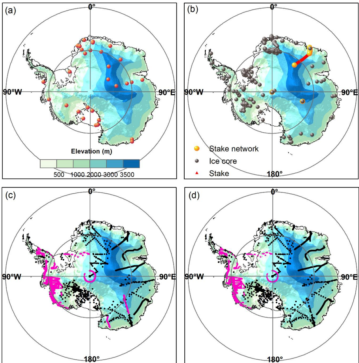
755 Figure 1: The comprehensive dataset of Antarctic SMB observations. (a) Spatial distribution of available AWS observations; (b) Locations of available annual resolved SMB observations. (c) Locations of available multi-year averaged SMB field data. Purple five-pointed stars standard for GPR measurements. Black points represent reliable SMB determined by stake/stake farms, ice cores/snow pits. (d) Location of multi-year averaged SMB data only during the second half 20th century selected for model validation.
