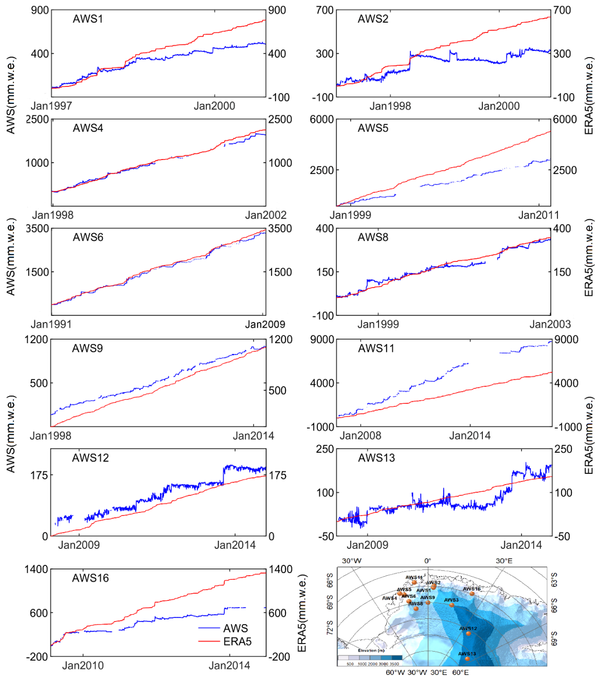
825 Figure 8: Cumulative daily snow accumulation and snowfall over time for each station over the Dronning Maud Land (a-k). (l) Spatial distribution of the AWS stations (Notice that AWS3 station records are not included due to a number of missing data)
