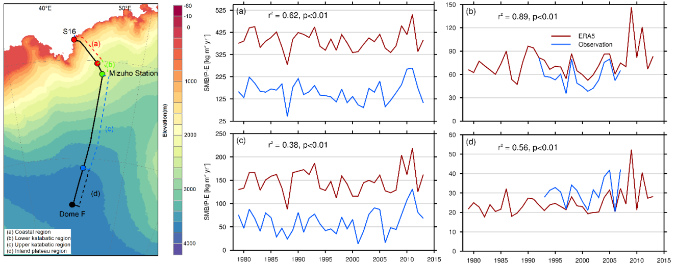
Figure 9: The left map showing the locations of stake measurements along the traverse between Syowa Station and Dome F, and the regional boundaries. The right four charts showing the comparison of the inter-annual variability in spatially-averaged stake measurements and snow accumulation simulated by ERA5 for (a) the coastal region, (b) lower katabatic region, (c) upper katabatic region, and (d) inland plateau region.
