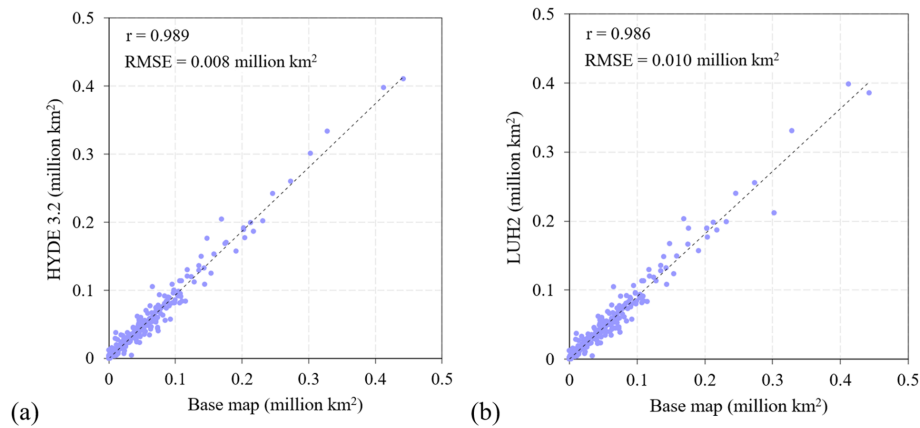
Figure 12. Comparison of cropland area at the downscaling region level between the base map and (a) HYDE 3.2 in 2010 CE and (b) LUH2 in 2010 CE. The black lines are the linear regression lines.
