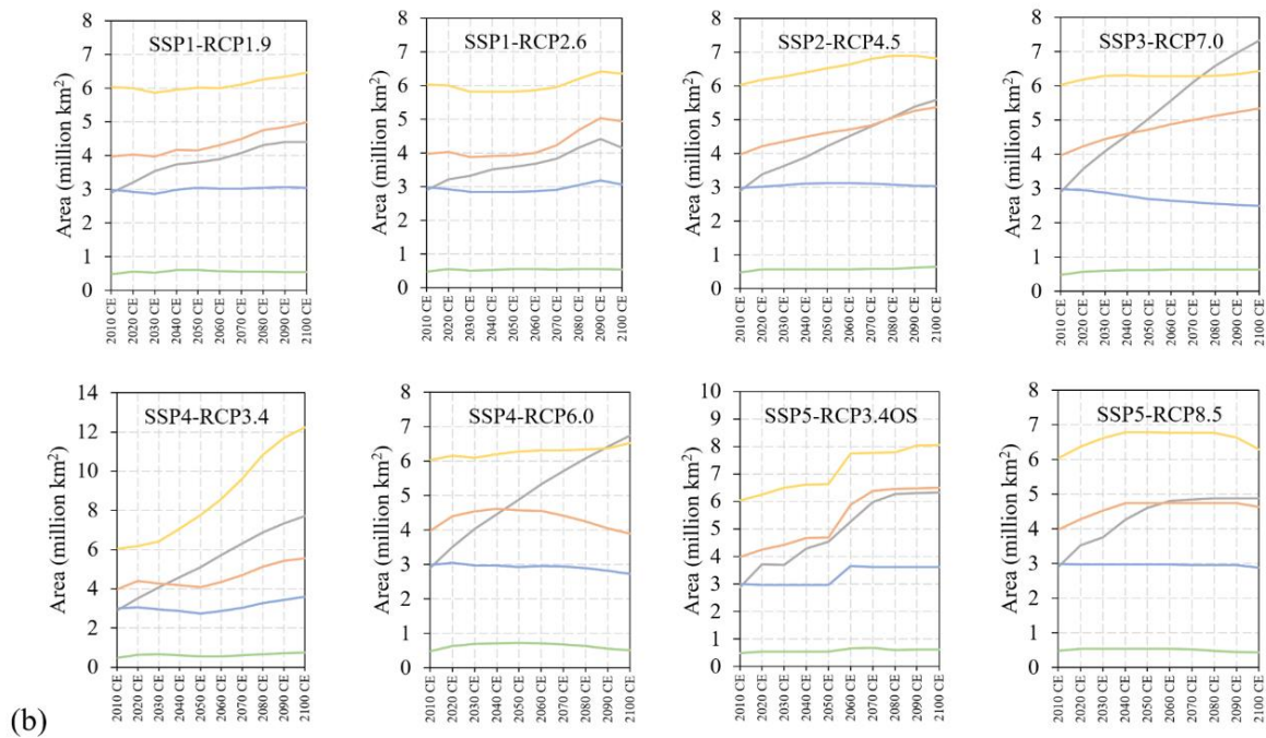
Figure 10: Cropland area of different continents for (a) 10000 BCE-2010 CE and (b) 2010 CE-2100 CE under eight future scenarios. The division of continents is based on countries and identical with FAO statistics.
