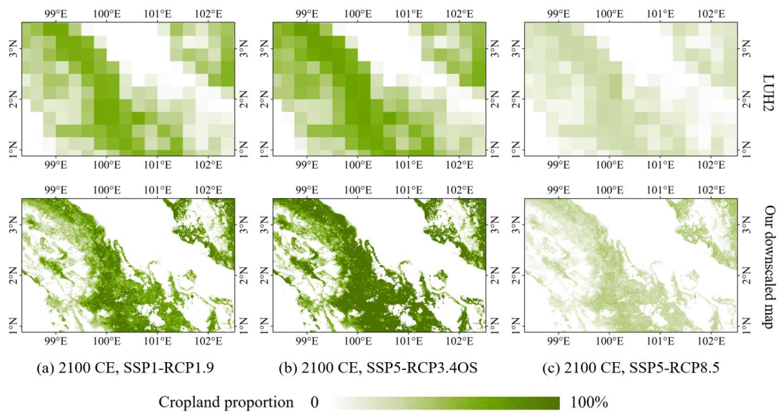
665 Figure 6: Cropland distribution of the region shown in Fig. 4f for different scenarios: (a)-(c). The location of image center points is Riau, Indonesia (2.199°N, 100.425°E).
