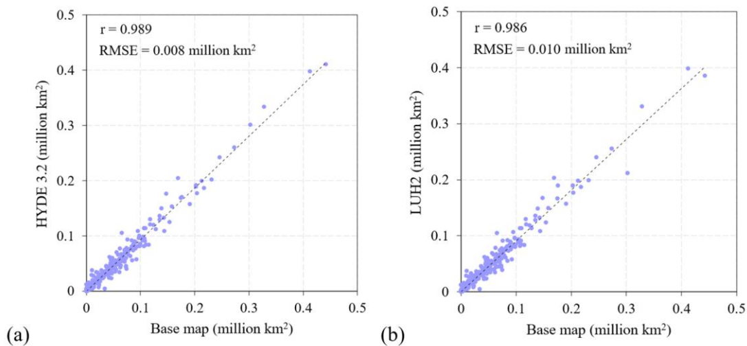
Figure 12: Comparison of cropland area at the downscaling region-level between the base map and (a) HYDE 3.2 in 2010 CE, (b) LUH2 in 2010 CE. The black lines are the linear regression lines.
