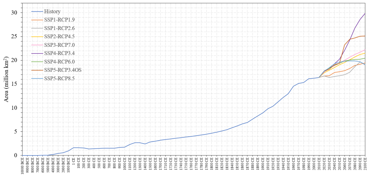
680 Figure 9: Global cropland area from 10000 BCE to 2100 CE.
