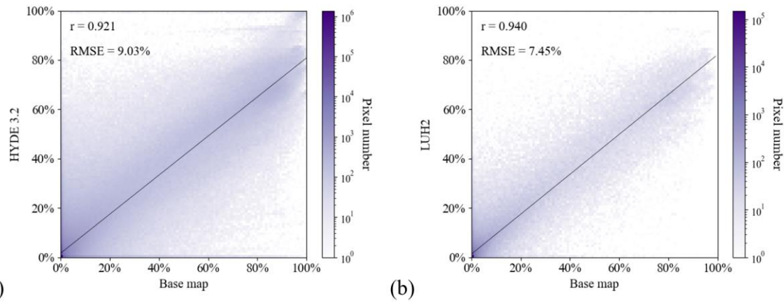
Figure 8: Comparison of cropland proportion in the corresponding pixels between the base map and (a) HYDE 3.2 in 2010 CE, (b) LUH2 in 2010 CE. Our downscaled maps were aggregated into 10 km and 0.25^\circ resolution for the two comparisons, respectively. The cell value represents the pixel numbers in the corresponding cropland proportion range. The black lines are the linear regression lines.
