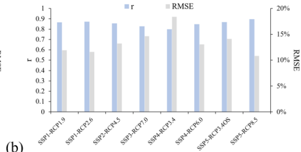
Figure 7: Comparison of cropland proportion in the corresponding pixels between our downscaled map and (a) HYDE 3.2 in the selected eight years, (b) LUH2 in 2100 CE under eight future scenarios. Our downscaled maps were aggregated into 10 km and 0.25° resolution for the two comparisons, respectively.
