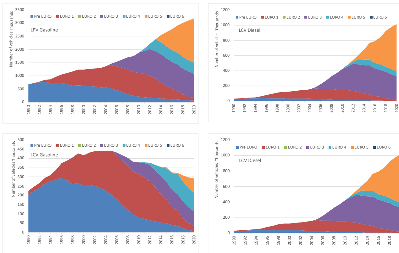
50 Figure 3. Emission standards and vehicle fleet in Chile, 1990-2020, for light passenger vehicles (LPV) and light commercial vehicles (LCV), using gasoline and diesel respectively
