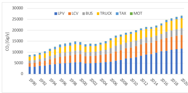
(a) CO 2
