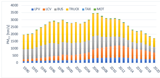
(c) PM 2.5
