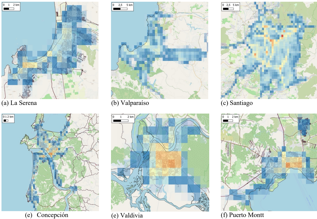
70 Figure 7. Spatial disaggregation of NO x exhaust emissions for six cities in Chile, 2020, as a fraction of Gg/y. Colour legend same as Figure 6.
