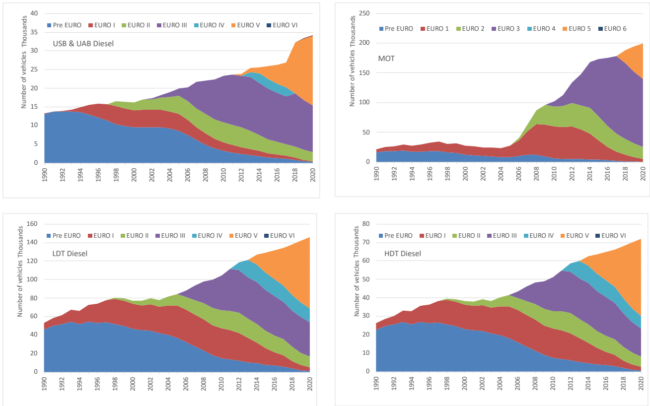
Figure 4. Emission standards and vehicle fleet in Chile, 1990-2020, for urban standard buses (USB), urban articulated buses (UAB), 2-wheelers (MOT), light-duty trucks (LDT) and heavy-duty trucks (HDT)
