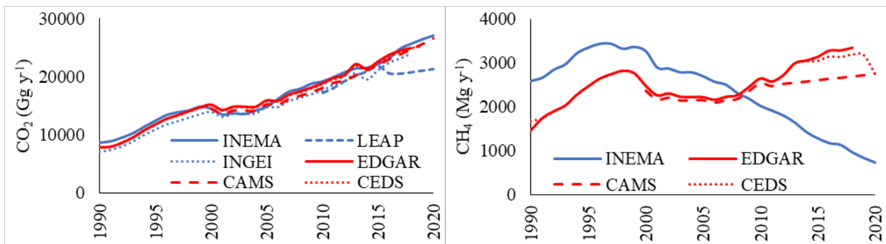
Figure 8. Comparison between CO 2 (left) and CH 4 (right) between this work (INEMA) and other local and global emission inventories.
