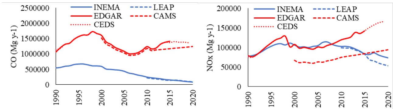
Figure 10. Comparison between CO (left) and NOx (right) between this work (INEMA) and other local and global emission inventories.
