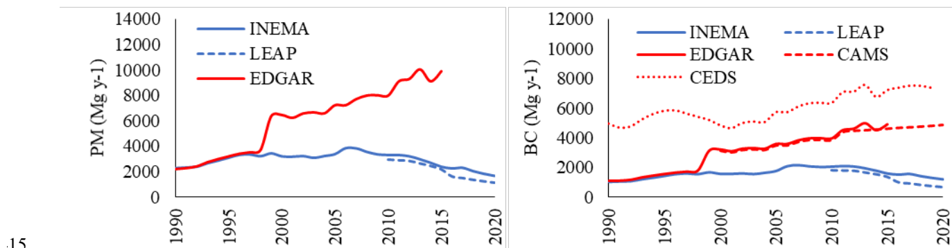
Figure 9. Comparison of PM 2.5 (left) and BC (right) emissions between this work (INEMA) and other local and global inventories.
