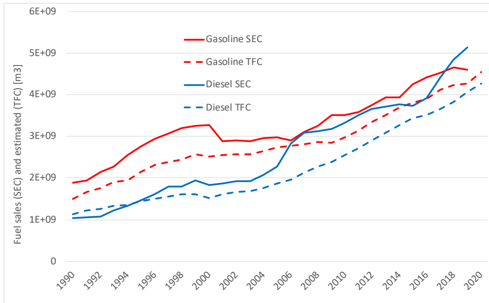
65 Figure 2. National fuel sales and estimated total fuel consumption for gasoline and diesel in Chile
