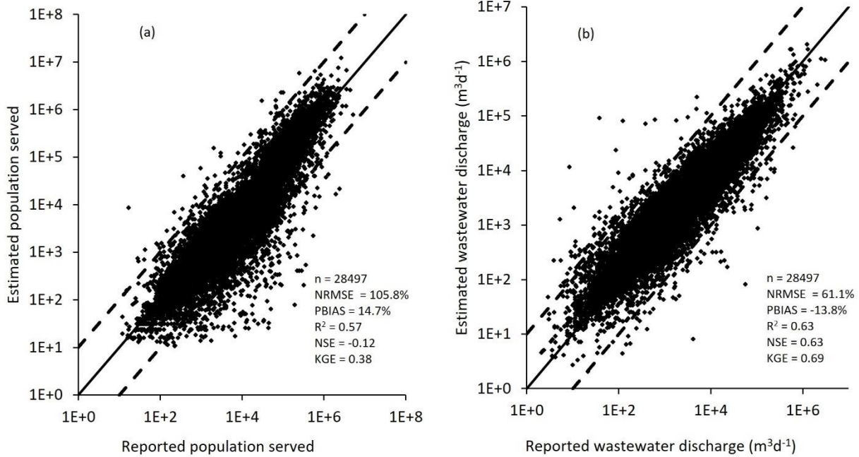
780 Figure 4. Evaluation of the method used to estimate missing attributes (see text for more explanations): population served (a) and treated wastewater discharge (b). n is the number of records, NRMSE is the normalized root mean square error, PBIAS is the percent bias, NSE is the Nash-Sutcliffe efficiency and KGE is the Kling-Gupta efficiency. The solid line represents the 1:1 line and the dashed lines represents the error line of one order of magnitude.
