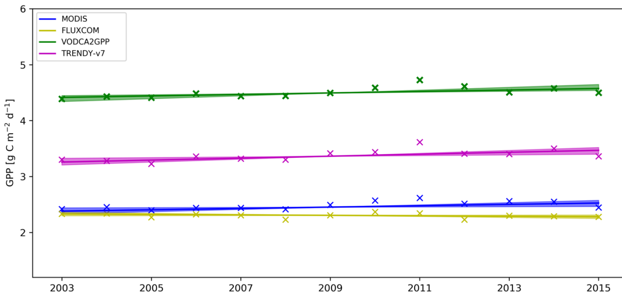
385 Figure 7: Time-series of yearly median GPP with the regression lines as obtained by the Theil-Sen estimator. Areas around the regression lines indicate the 90%-confidence intervals.
