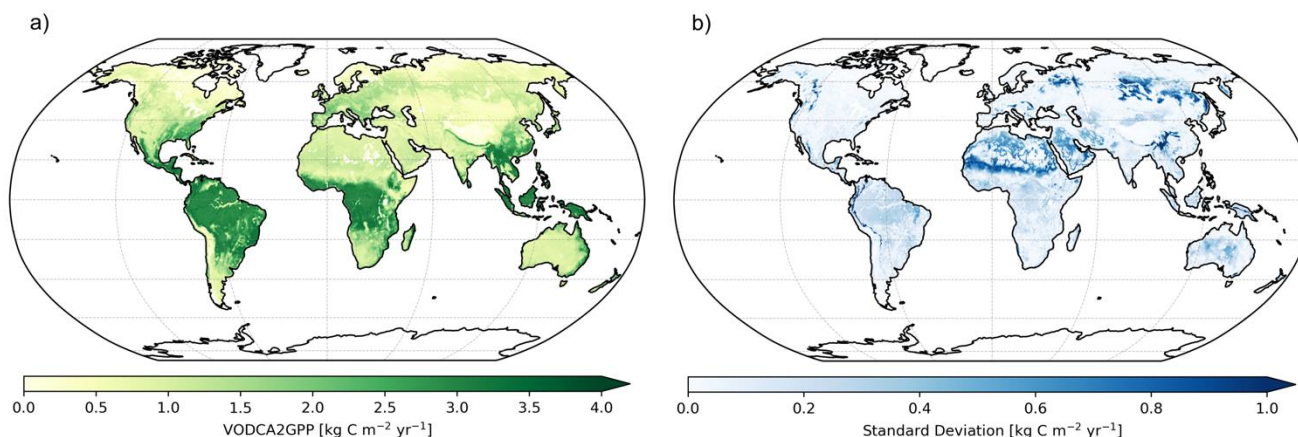
295 Figure 2: a) Mean annual GPP as derived from VODCA2GPP for the period 1988-2019. b) Standard deviation of mean annual GPP (1988-2019) as obtained by the uncertainty analysis based on site-level cross-validation.
