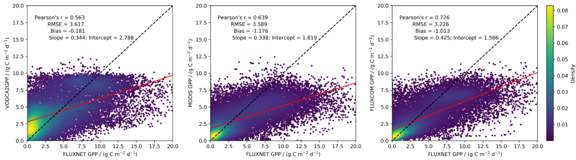
Figure 4: GPP from FLUXNET plotted against GPP from VODCA2GPP, MODIS and FLUXCOM for the period 2002-2016 with 8-daily sampling.
