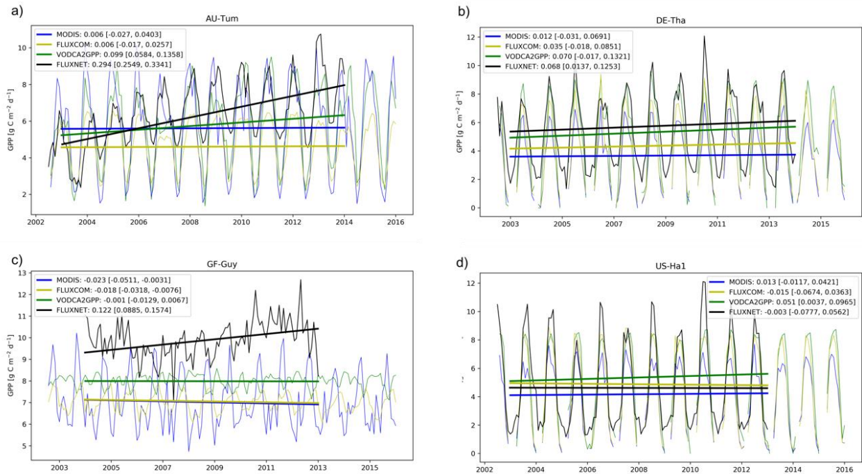
550 Figure A6: Exemplary collection of time series of in-situ FLUXNET GPP together with extracted time series from MODIS, FLUXCOM and VODCA2GPP. The stations were selected because of their high data availability for the respective landcover. The lines indicate the regression lines as obtained from the Theil-Sen slope estimation for yearly median GPP. The trends are computed for the common observation period with FLUXNET. The slope [ \text{g C m}^{-2} \text{yr}^{-1} ] is depicted in the legend together with the respective 90% lower/upper confidence intervals. The depicted stations are:
