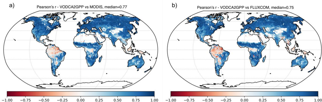
Figure 3: Pearson's r between VODCA2GPP and MODIS GPP (a) and VODCA2GPP and FLUXCOM GPP (b). The correlations are based on the common observation period between 2002 and 2016 with 0.25^\circ spatial and 8-daily temporal resolution.
