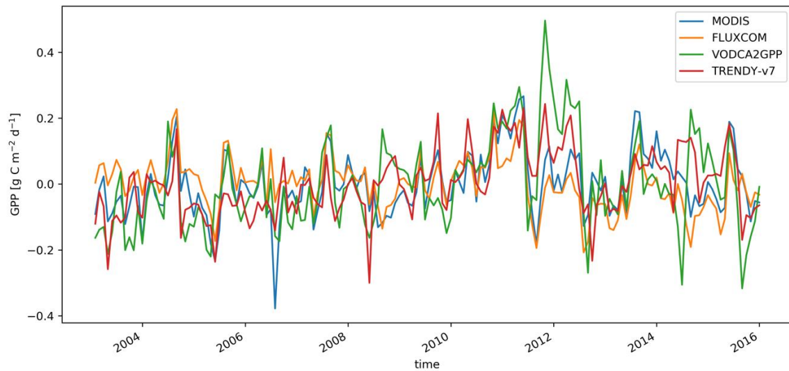
350 Figure 6: Time-series of mean global monthly GPP anomalies.
