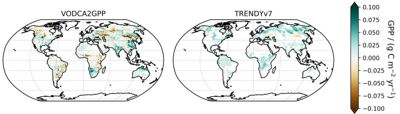
545 Figure A5: Global maps of yearly median GPP trends for the period 1988-2016 for VODCA2GPP and TRENDY-v7. White indicates non-significant trends.
