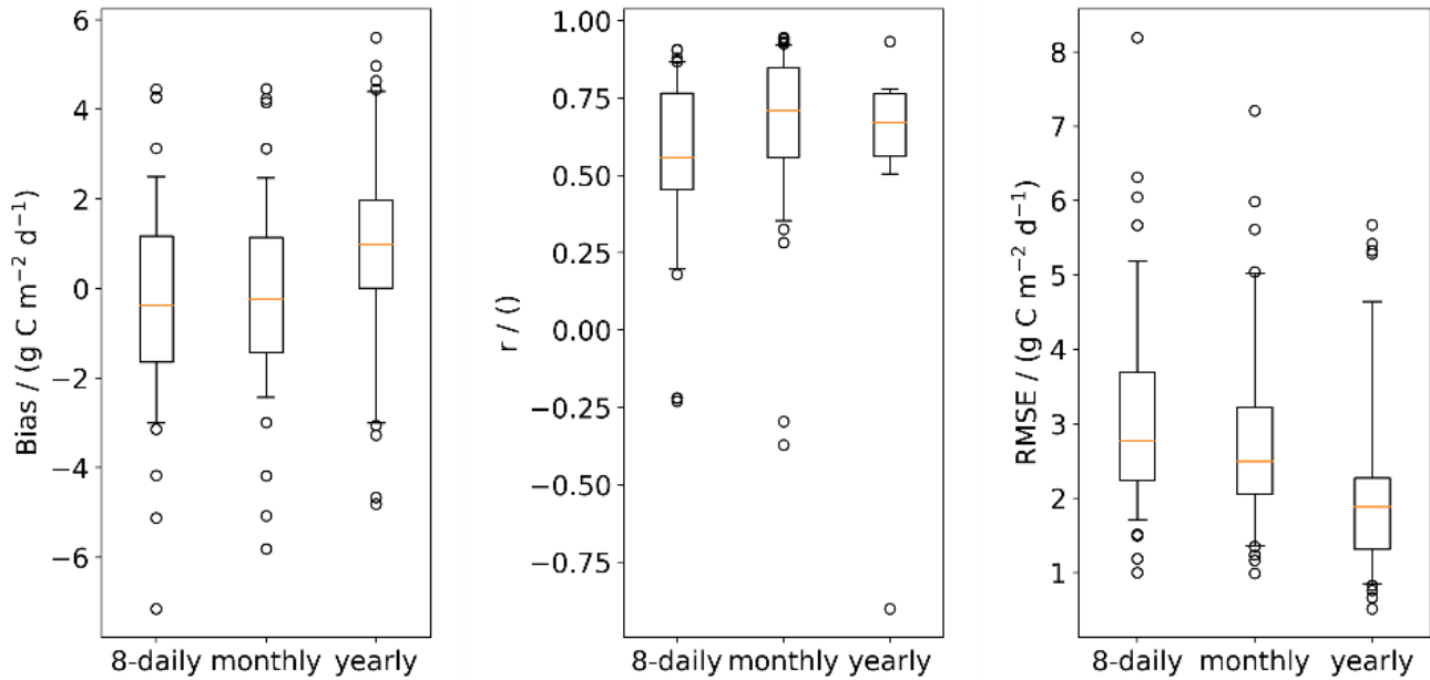
Figure 5: Site-based cross-validation for 8-daily, monthly, and yearly sampling of GPP from VODCA2GPP and FLUXNET. RMSE, Bias and Pearson's r were computed at each of the 10% of FLUXNET sites that were omitted during the respective training run. Non-significant Pearson correlation ( p -value < 0.1 ) were ignored. The boxplots for Pearson's r are based on the 71 (8-daily), 66 (monthly) and 8 (yearly sampling) significant values for Pearson's r values. The whiskers of the boxplots extend to the 0.05/0.95 percentiles.
