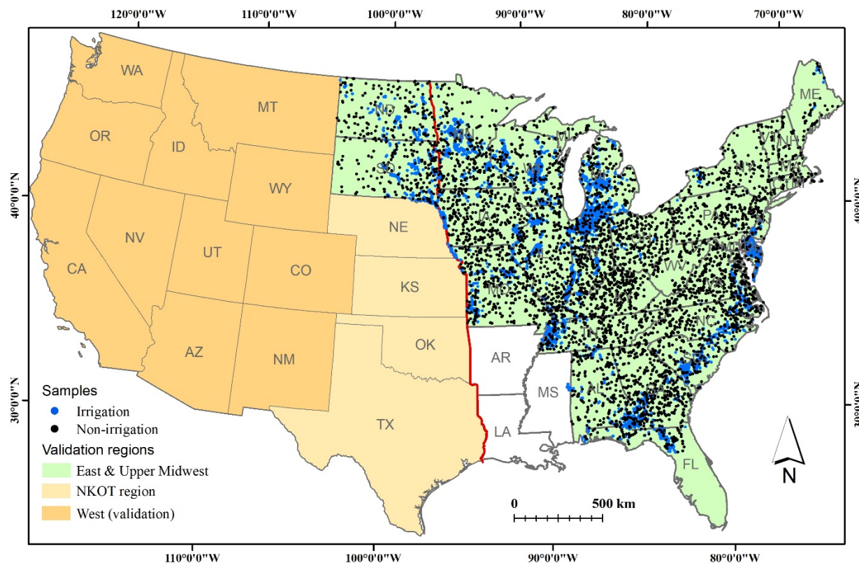
125 Figure 2: Map evaluation and comparison design and the distribution of test sample locations across the eastern CONUS. The NKOT region refers to Nebraska, Kansas, Oklahoma, and Texas, which covers the majority of the High Plains Aquifer. The red solid line represents the West-East division for classification only.
