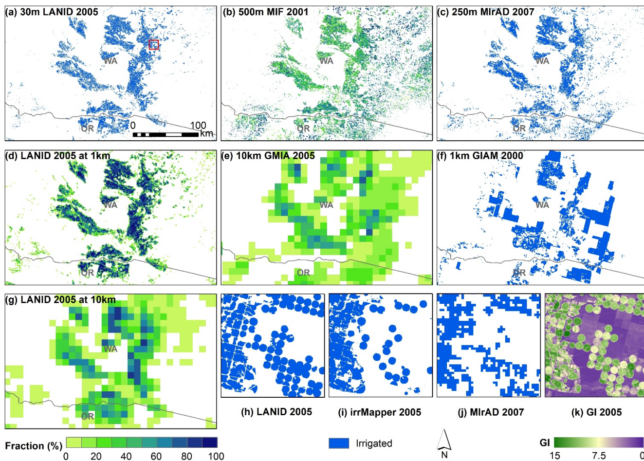
Figure 11: Product comparison at the Columbia Plateau Aquifer in northern Oregon and southern Washington. In addition to the original 30-m LANID (a), the map is aggregated to 1 km and 10 km resolution for displays (d) and (g). (h)-(i) show the location highlighted in (a) (red rectangle).
