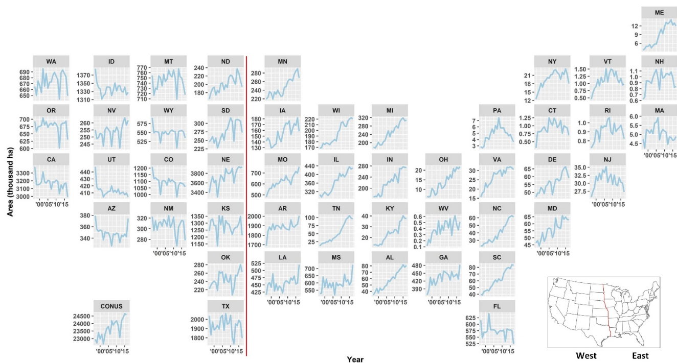
Figure 4: LANID-derived annual irrigation area by state, 1997-2017. The red line shows the East-West division in this study based on a climatic transition near the 100th meridian. Annual irrigation area per state is provided in Table A1.
