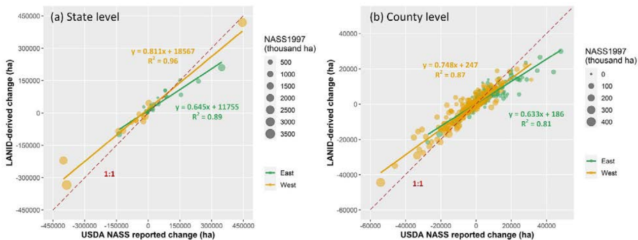
180 Figure 5: LANID-derived irrigation changes vs. USDA-NASS reported area at the state (a) and county (b) scale. Irrigation change was calculated as the difference between mean area of years 2012 and 2017 and that of 1997 and 2002 (i.e., \text{mean}(\text{irArea}_{2012} + \text{irArea}_{2017}) - \text{mean}(\text{irArea}_{1997} + \text{irArea}_{2002}) where \text{irArea}_{yr} refers to irrigation area of year yr ). The USDA-NASS reported values of 1997 is shown to represent irrigation area at the starting point of the study period.
