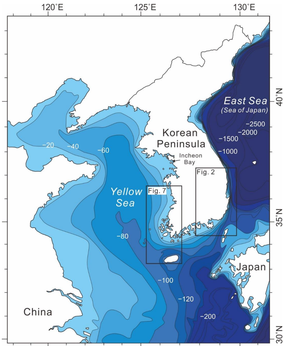
Figure 1: Bathymetry around the Korean Peninsula (modified after Chough et al., 2000; 2004; Cummings et al., 2016). Water depth contours are Bathymetric contour interval is in meters. Detailed maps with sampling areas are shown in Figs. 2, 7.
