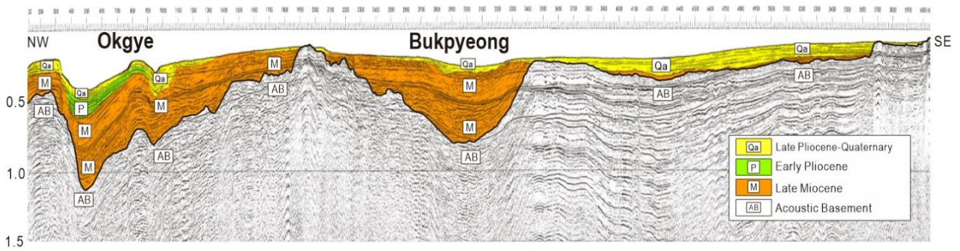
635 Figure 13: Parallel seismic Seismic section obtained parallel to the coastline and its stratigraphic interpretation (modified after Kwon, 2005; Ryang et al., 2007, 2014). For the location of the seismic track line, see Fig. 12.
