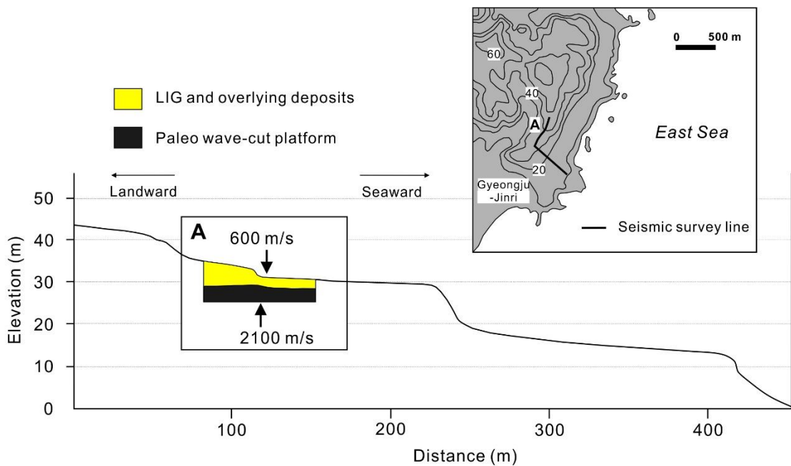
140 Figure 5: Seismic interpretation and calculated elevation of the buried LIG wave-cut platform at Subsite Jinri of the Gyeongju area, based on seismic velocities between the overlying deposits and a paleo wave-cut platform (modified after J.W. Kim et al., 2007a). The topographic contour interval is 10 meters. For location, see Fig. 2.
