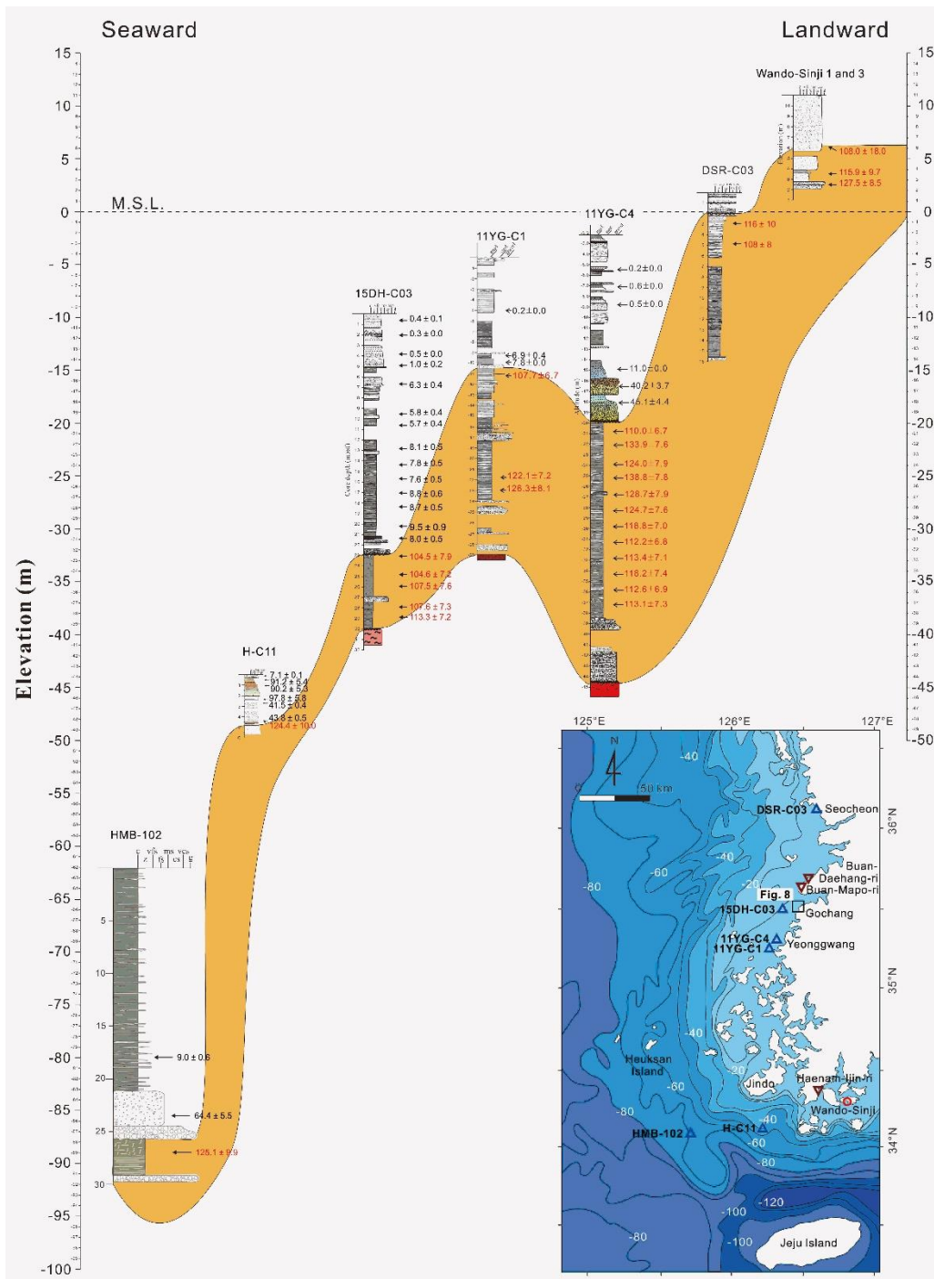
Figure 11: Arrangement of onshore sections (Wando-Sinji 1 and SJ3) and tidal-to-nearshore core sections (DSR-C03 to HMB-102) along the west coast of Korea according to the elevation of the remnant LIG deposits. Orange shading highlights the correlation of LIG deposits across the 6 coastal cores and Wando outcrop sections. Ages in red indicate LIG ages (WALIS LUM ID #470 to #491 in Table 3). For location, see Fig. 7.
