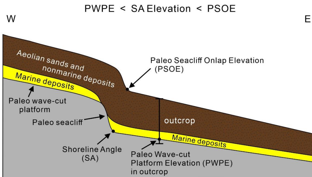
Figure 6: A schematic marine terrace commonly occurred occurring along the eastern Korean Peninsula. Note that the shoreline angle (SA) elevation is between the paleo wave-cut platform elevation (PWPE) measured in outcrop and the paleo seacliff onlap elevation (PSOE) measured in surface topography.
