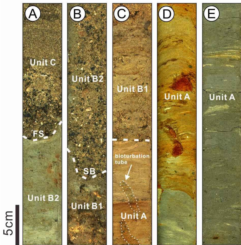
Figure 10: Selected photographs of core sediments in core DSR-C03 in Fig. 9. (a) Massive mud-free sand beds with laminated sand, pebble, shell-rich layers (Unit C). (b) Muddy coarse-grained sediments with relatively less weakly oxidized poorly sorted gravel and sand (Unit B2). (c) Completely oxidized poorly sorted gravel and sand without muddy sediments (Unit B1). (d, e) Moderately bioturbated, laminated, sandy mud and muddy sand with moderate amounts of flaser , wavy to lenticular bedding and rhythmic lamination (Unit A). The oxidized upper part of Unit A is reddish while the lower part has a gray color. TRS: Transgressive Ravinement Surface, SB: Sequence Boundary
