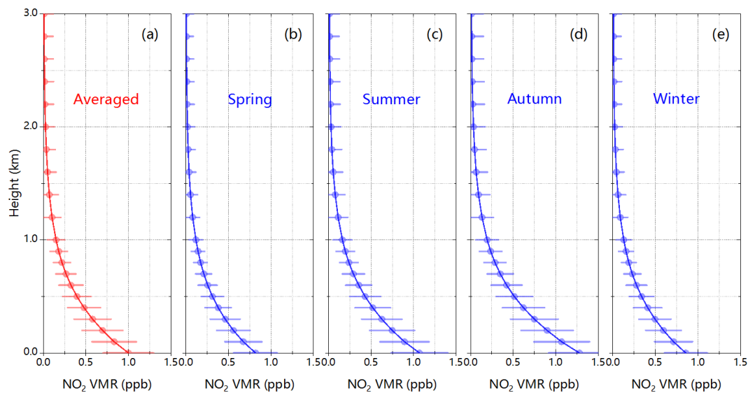
670 Figure 9. (a) total averaged, (b) spring averaged, (c) summer averaged, (d) autumn averaged, and (e) winter averaged NO 2 vertical profiles from December 2017 to February 2019 at the CAS (QOMS) station.
