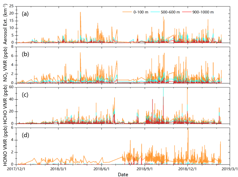
660 Figure 6. Time series of hourly averaged (a) aerosol extinction, (b) NO 2 , (c) HCHO, and (d) HONO from December 2017 to February 2019 at the CAS (QOMS) station.
