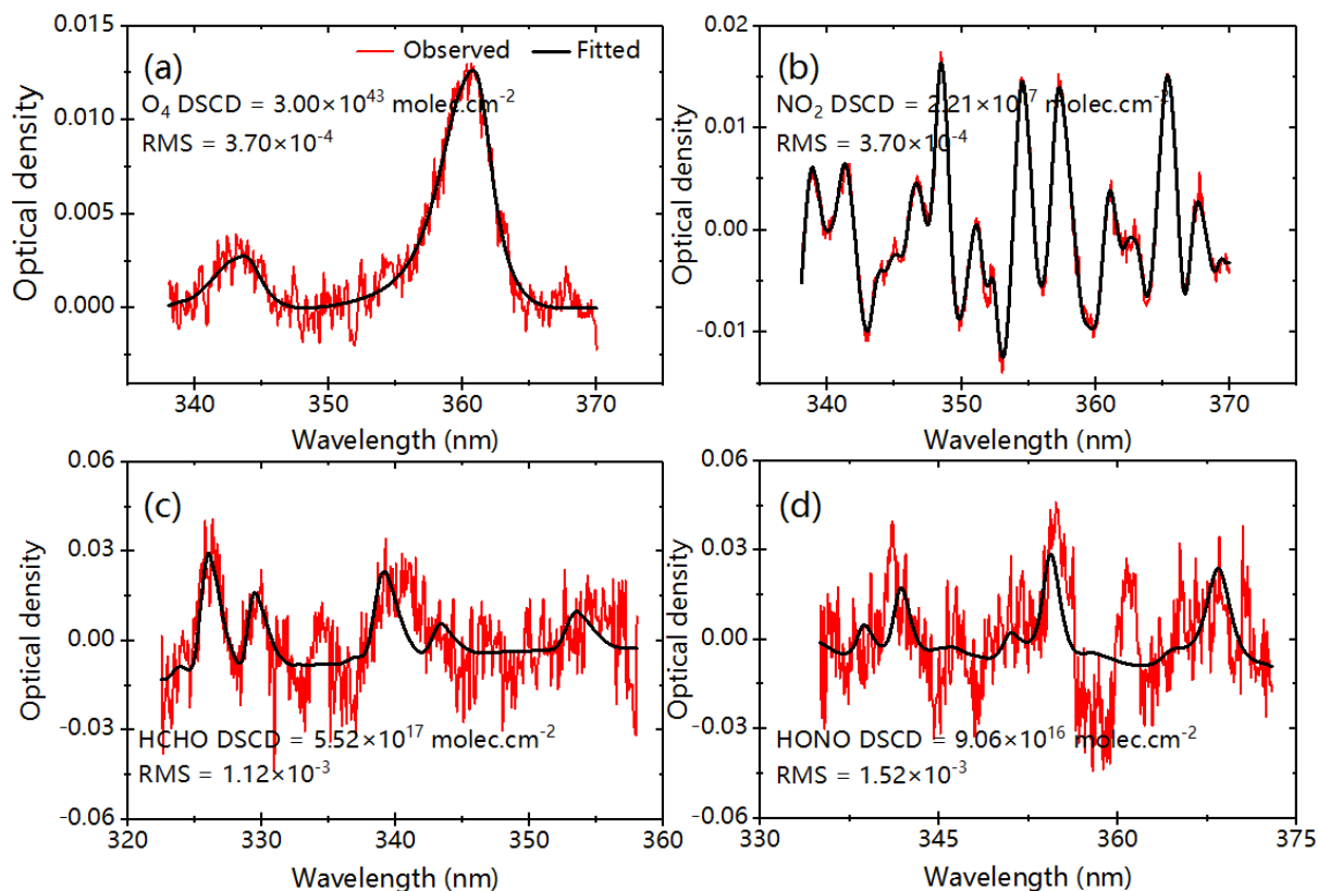
650 Figure 3. Examples of DOAS fits for O_4 , NO_2 , HCHO and HONO (~13:30 LST on May 22, 2018, SZA and EVA values were 52.53° and 15°, respectively).
