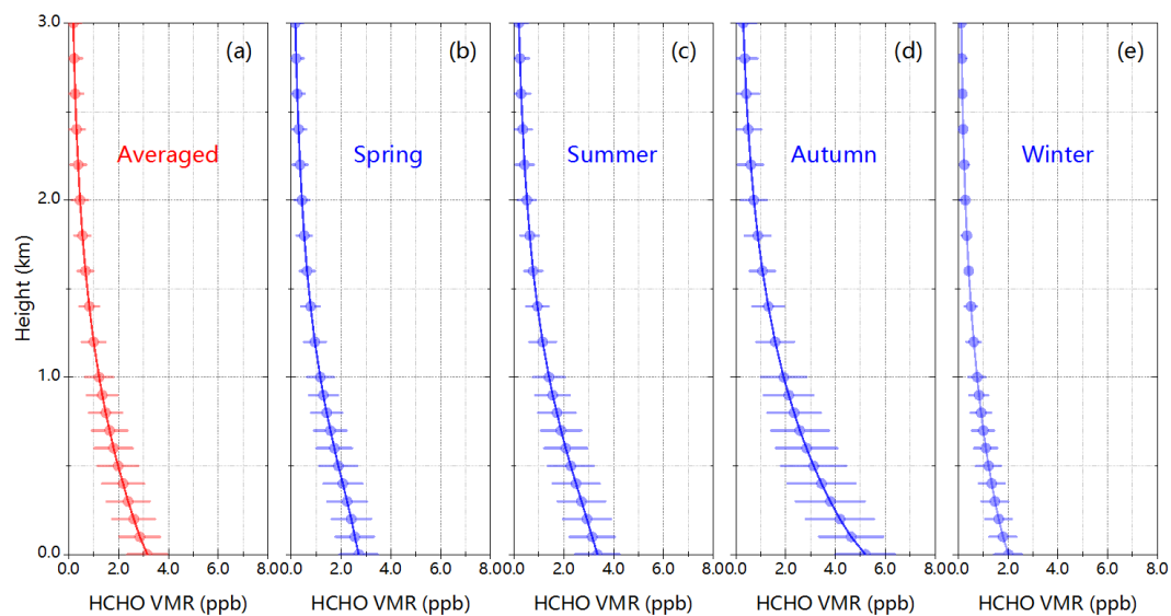
675 Figure 10. (a) total averaged, (b) spring averaged, (c) summer averaged, (d) autumn averaged, and (e) winter averaged HCHO vertical profiles from December 2017 to February 2019 at the CAS (QOMS) station.
