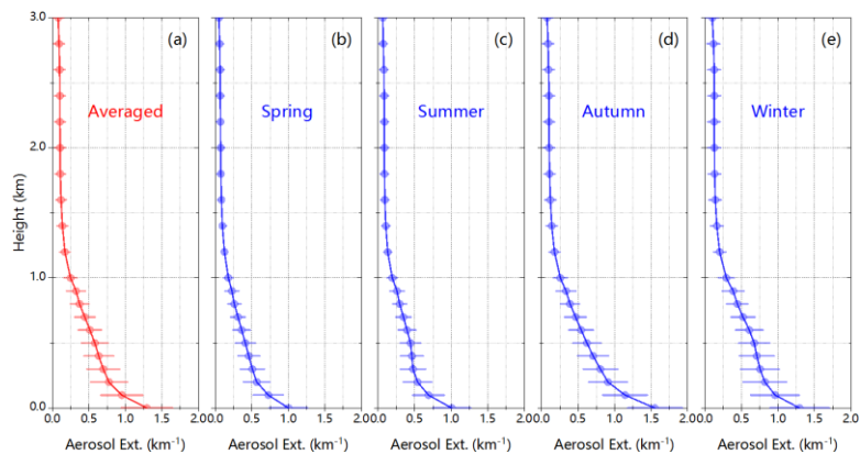
680 Figure 7. (a) total averaged, (b) spring averaged, (c) summer averaged, (d) autumn averaged, and (e) winter averaged aerosol extinction vertical profiles from December 2017 to February 2019 at the CAS (QOMS) station.
