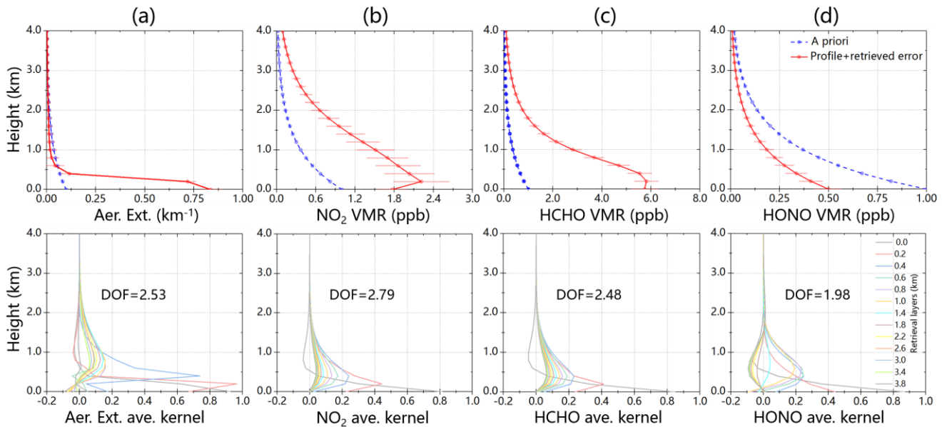
➤ Figure S2. Retrievals at 11:11:30 (LST) on 10 March at the CAS (QOMS) station. (a) aerosol extinction, (b) NO 2 , (c) HCHO and (d) HONO. The top row shows the retrieved profiles, plotted with their associated a priori profile and retrieved errors. The bottom row presents the averaging kernels and degrees of freedom for signal associated with the profile retrieval.
