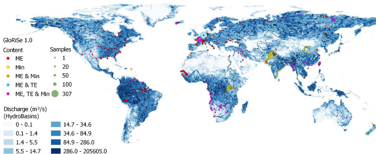
130 Figure 1 Spatial extent of the database. Dot size indicate the number of samples available per location. Dot colour indicates what 135 kind of data is available at that location (ME: Major & minor elements, TE: Trace elements, Min: Mineralogical or petrological composition). River water discharge, as indicated by blue coloration, was taken from the HydroBasins database at Pfaffstetter level 7 (Linke et al., 2019).
