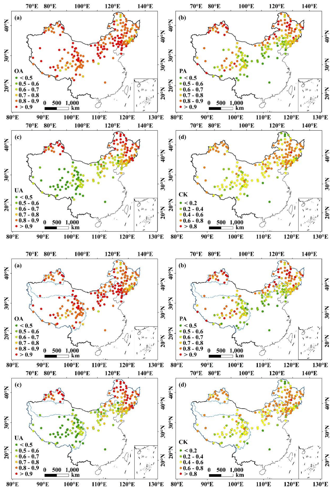
Figure 78: Point-based accuracy results of NIEER AVHRR product: (a) OA; (b) PA; (c) UA; (d) CK. The snow depth of 191 climate stations used is provided by the China Meteorological Administration (CMA). OA,
