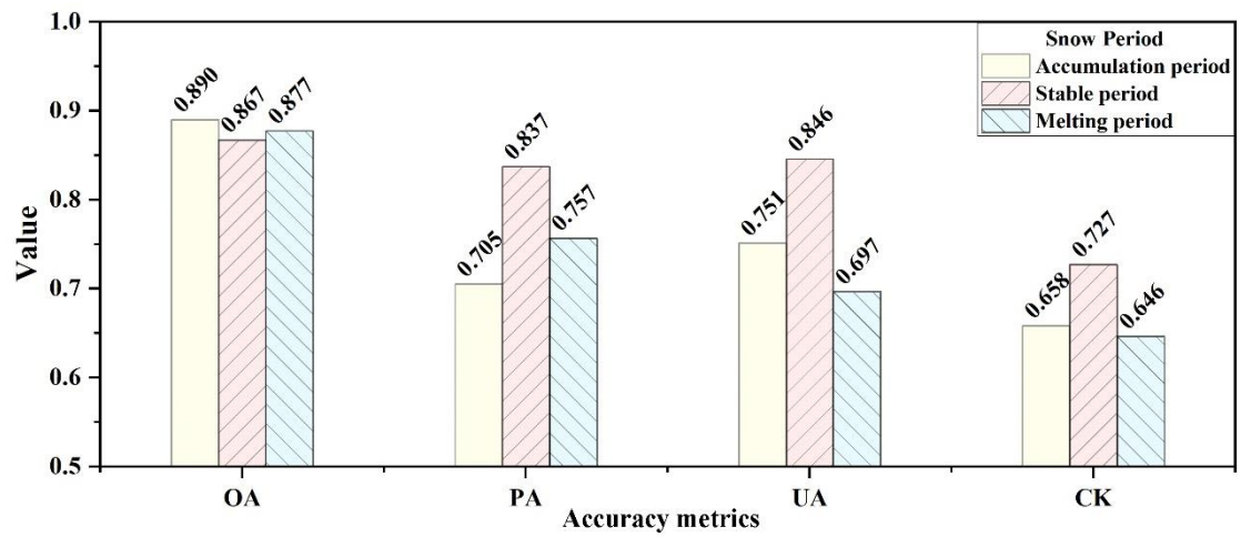
Figure 1011: Histogram of accuracy results of NIEER AVHRR SCE product in different snow periods, including accumulation period, stable period, melting period
