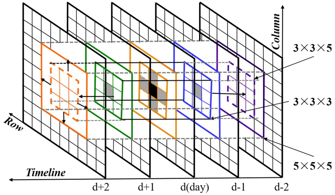
Figure 56: Diagram of the HMRF-based gap-filling process used in the study.
