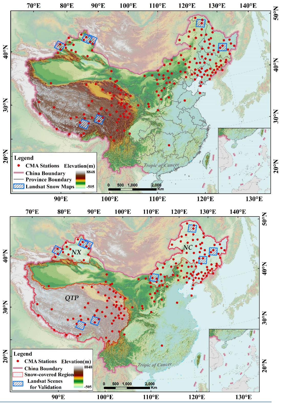
570 Figure 1: The geographic location of study area and the spatial distribution of major snow-covered regions , climate stations and Landsat-5 validation dataset. The elevation data were derived from Shuttle Radar Topography Mission (SRTM).-
