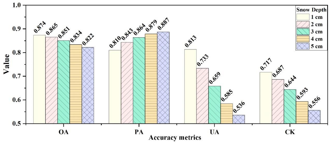
Figure 9-10: Histogram of accuracy results of NIEER AVHRR SCE product under different snow depth thresholds.
