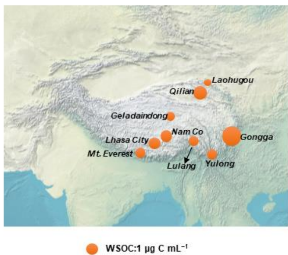
900 Figure 11. Spatial distributions of precipitation WSOC on the Tibetan Plateau and its surroundings (left), and WSOC temporal variations and flux from Qilian Station (right). Modified from Gao et al., 2021 .
