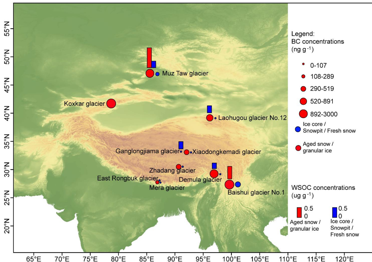
885 Figure 7. BC and WSOC concentrations from studied glaciers distributed on the Tibetan Plateau and surroundings.
