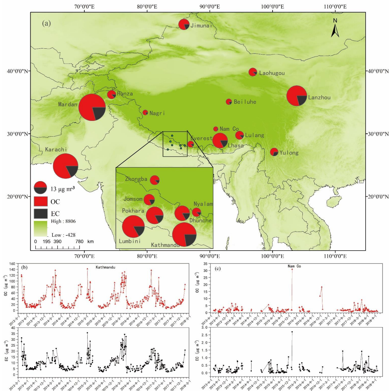
880 Figure 5. Aerosol OC and EC concentration distributions in the TP (top), and temporal variations of OC and EC concentrations at Kathmandu and Nam Co station (bottom) during the observed periods, respectively. The abbreviations can be found in Table 1.
