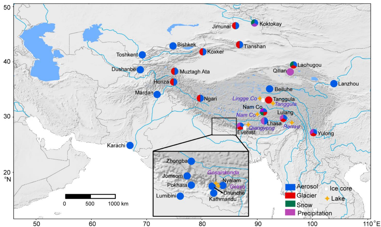
Figure 1. Schematic overview of measurements from the Atmospheric Pollution and Cryospheric Changes (APCC) network, in which coordinated carbonaceous component measurements were made on samples from the atmosphere, glaciers, snow cover, precipitation, and lake sediments. The location information for each station, glacier and lake are provided in Tables 1, 2 and 3.
