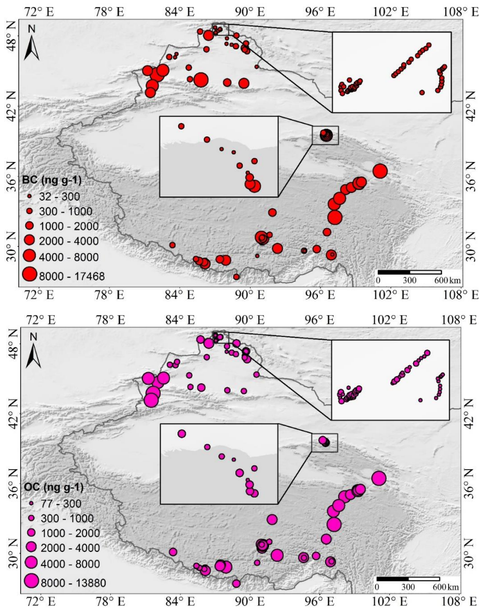
Figure 8. Spatial distributions of BC (top) and OC (bottom) concentrations in snow cover for each sampling site across the Tibetan Plateau and the Northern Xinjiang. Data cited from Zhang et al., 2018a ; Zhong et al., 2019 .
