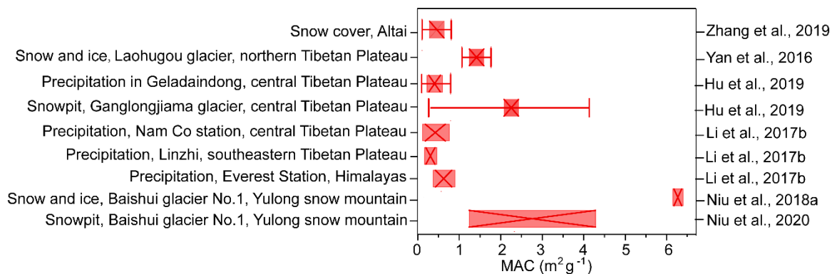
895 Figure 10. Comparison of the mass absorption cross section (MAC) of WSOC in snow and ice, and precipitation in the Tibetan Plateau and its surroundings.
