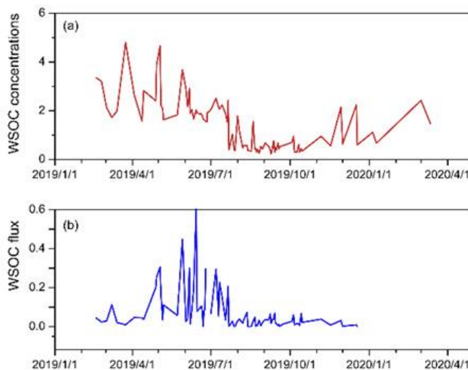
900 Figure 11. Spatial distributions of precipitation WSOC on the Tibetan Plateau and its surroundings (left), and WSOC temporal variations and flux from Qilian Station (right). Modified from Gao et al., 2021 .
