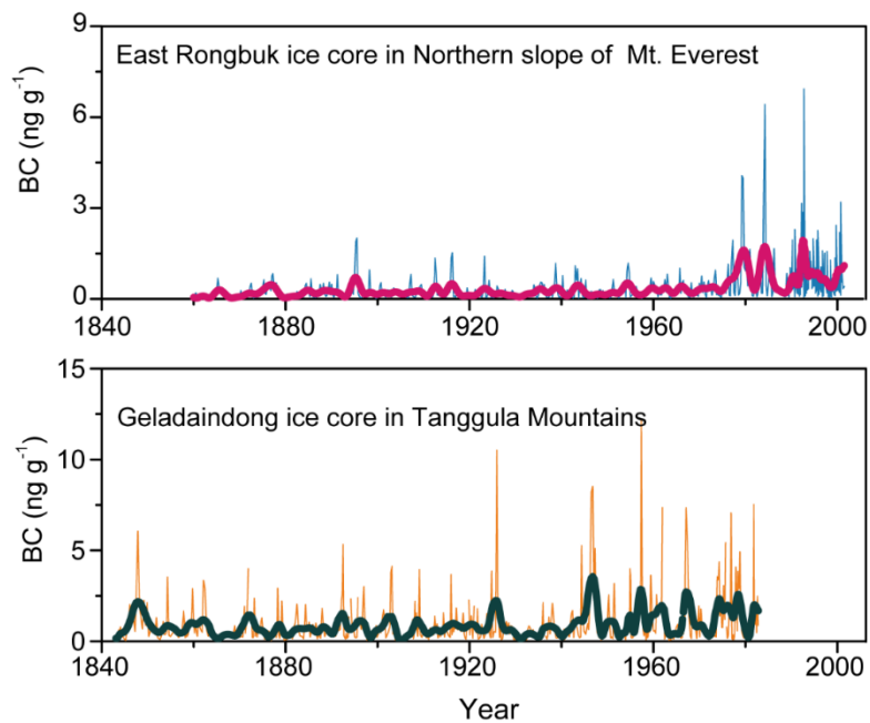
905 Figure 13. Historical BC concentration records retrieved from ice cores over the Himalayas and Tibetan Plateau. East Rongbuk ice core data from the northern slope of Mt. Everest (Kaspari et al., 2011), and Geladaindong ice core data from the Central TP (Jenkins et al., 2016).
