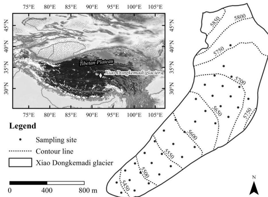
Figure 3. Surface snow and snowpit sampling sites for the Xiaodongkemadi glacier (Modified from Li X et al., 2017).
