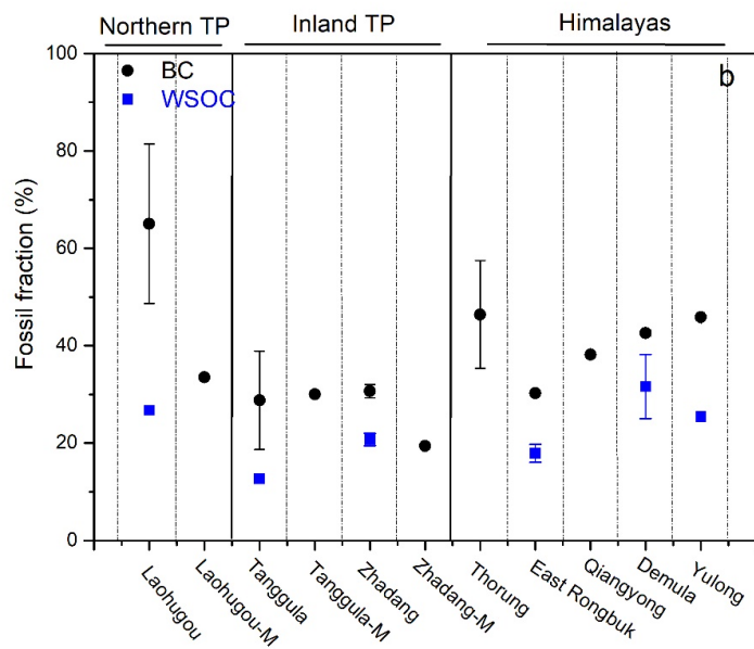
1010 Figure 12. BC carbon and WSOC isotopes from snowpit samples in the Himalayas and Tibetan Plateau. Modified from (Li et al., 2016a).
