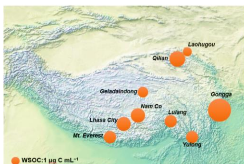
1005 Figure 11. Spatial distributions of precipitation WSOC on the Tibetan Plateau and its surroundings (left), and WSOC temporal variations of concentrations and flux from precipitation at Qilian Station in the northern Tibetan Plateau (right). (a) Precipitation WSOC concentrations and (b) Precipitation WSOC flux (Modified from Gao et al., 2021b).
