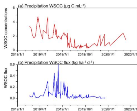
1005 Figure 11. Spatial distributions of precipitation WSOC on the Tibetan Plateau and its surroundings (left), and WSOC temporal variations of concentrations and flux from precipitation at Qilian Station in the northern Tibetan Plateau (right). (a) Precipitation WSOC concentrations and (b) Precipitation WSOC flux (Modified from Gao et al., 2021b).
