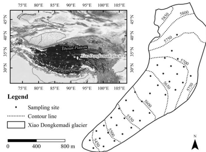
Figure 3. Black carbon and organic carbon data in surface snow and snowpit sampling sites for from the Xiaodongkemadi glacier at Tanggula Mountains in the central Tibetan Plateau. Modified from (Li et al., 2017a).
