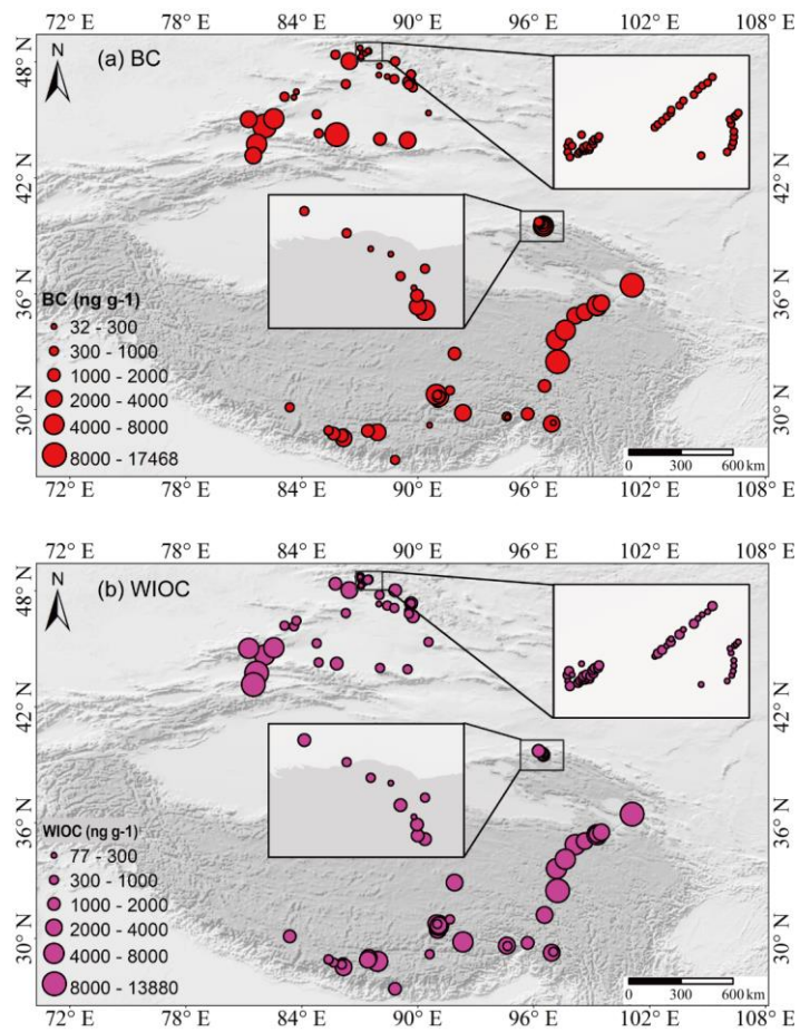
990 Figure 8. Spatial distributions of (a) BC and (b) WIOC concentrations in snow cover for each sampling site across the Tibetan Plateau and the Northern Xinjiang. Data cited from (Zhang et al., 2018a; Zhong et al., 2019).
