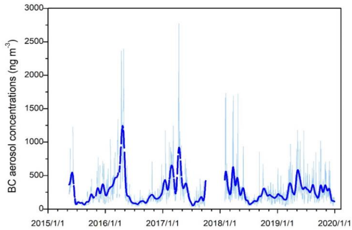
0975 Figure 4. Daily mean BC aerosol concentrations at Everest Station (Mt. Everest region) measured by AE-33 during May15, 2015 to December 29, 2019. Light blue lines refer to daily data; the thick blue lines represent the smoothing results.
