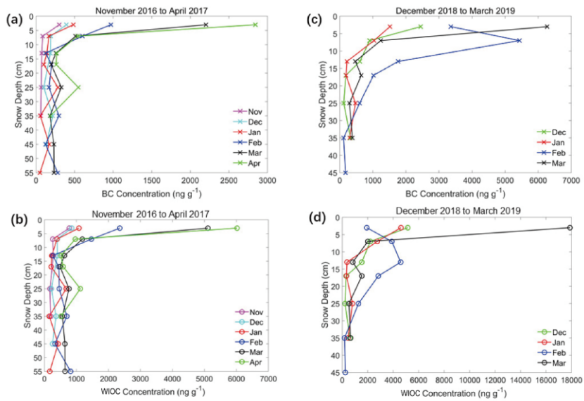
Figure 9. Vertical variations of mean BC and W IOC concentrations in snowpits at Koktokay snow station during two snow years (Zhong et al., 2019).
