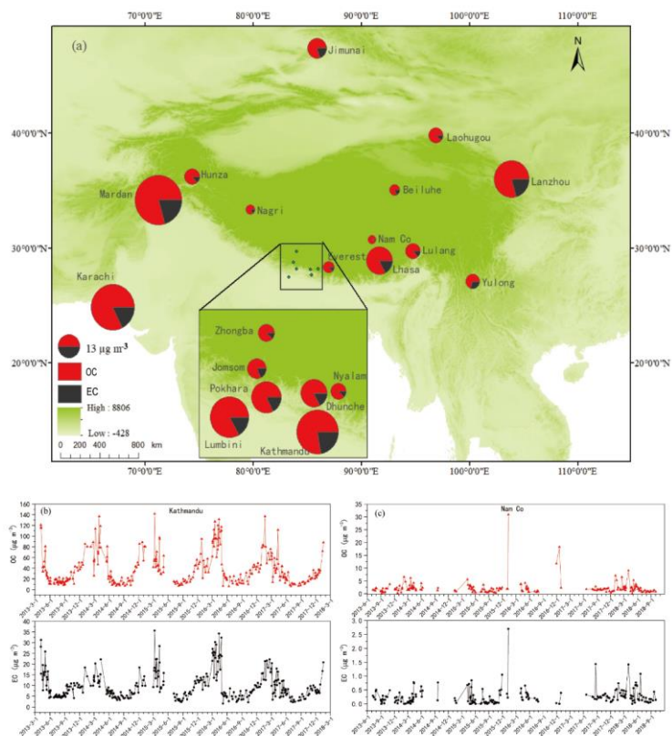
980 Figure 5. Aerosol OC and EC concentration distributions in the TP-Tibetan Plateau and its surroundings (top), and temporal variations of OC and EC concentrations at Kathmandu and Nam Co station (bottom) during the observed periods, respectively. The abbreviations can be found in Table 1.
