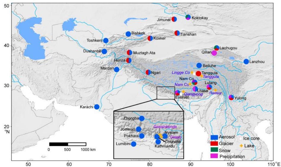
965 Figure 1. Schematic overview of measurements from the Atmospheric Pollution and Cryospheric Changes (APCC) network program over the Third Pole , in which coordinated carbonaceous component measurements were made on samples from the atmosphere, glaciers, snow cover, precipitation, and lake sediment cores . The location information for each station, glacier and lake are provided in Tables 1, 2 and 3.
