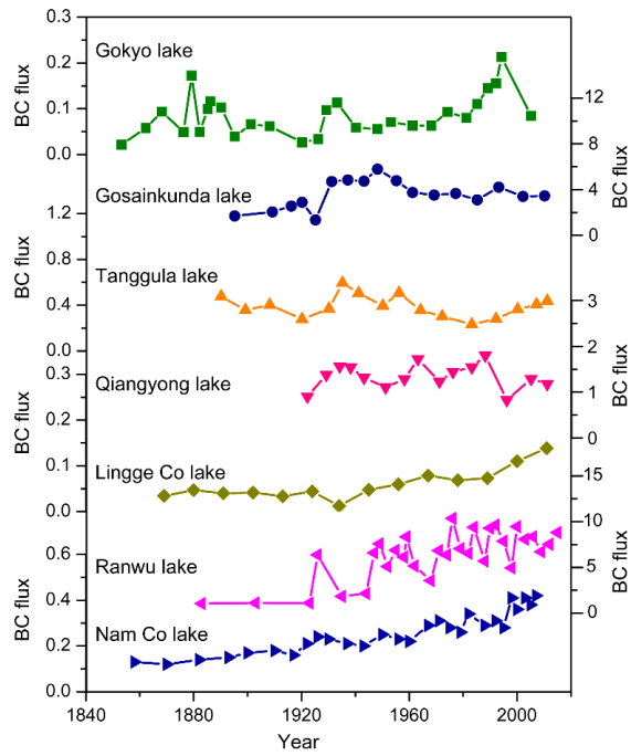
Figure 14. Historical BC flux ( \text{g m}^{-2} \text{yr}^{-1} ) retrieved from lake sediment cores across the Third Pole . Nam Co lake sediment cores data was cited from (Cong et al., 2013); other lake sediment cores data was cited from (Neupane et al., 2019).
