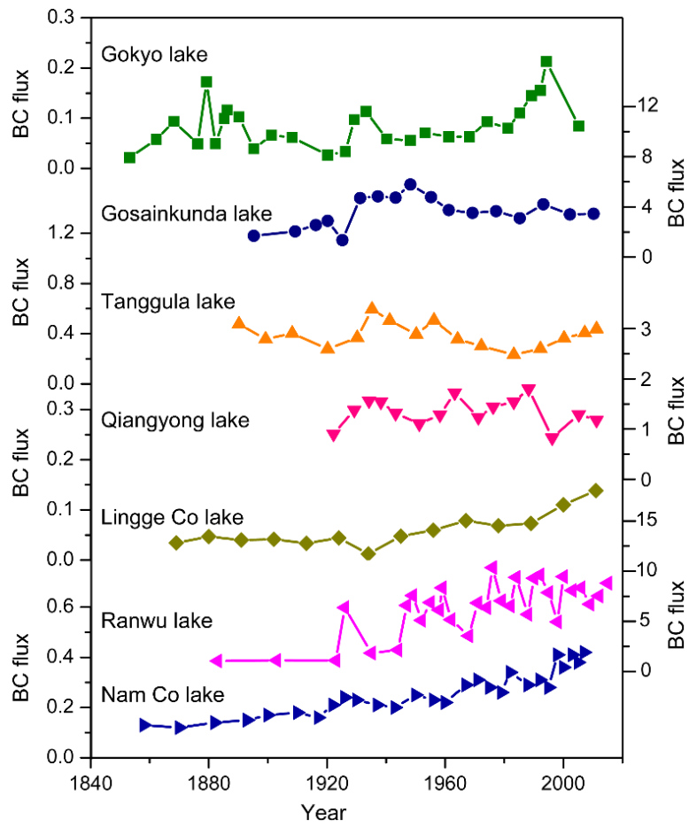
995 Figure 14. Historical BC flux ( \text{g m}^{-2} \text{yr}^{-1} ) retrieved from lake sediment cores. Nam Co lake sediment cores data was cited from Cong et al., (2013) ; other lake sediment cores data was cited from Neupane et al. (2019) .
