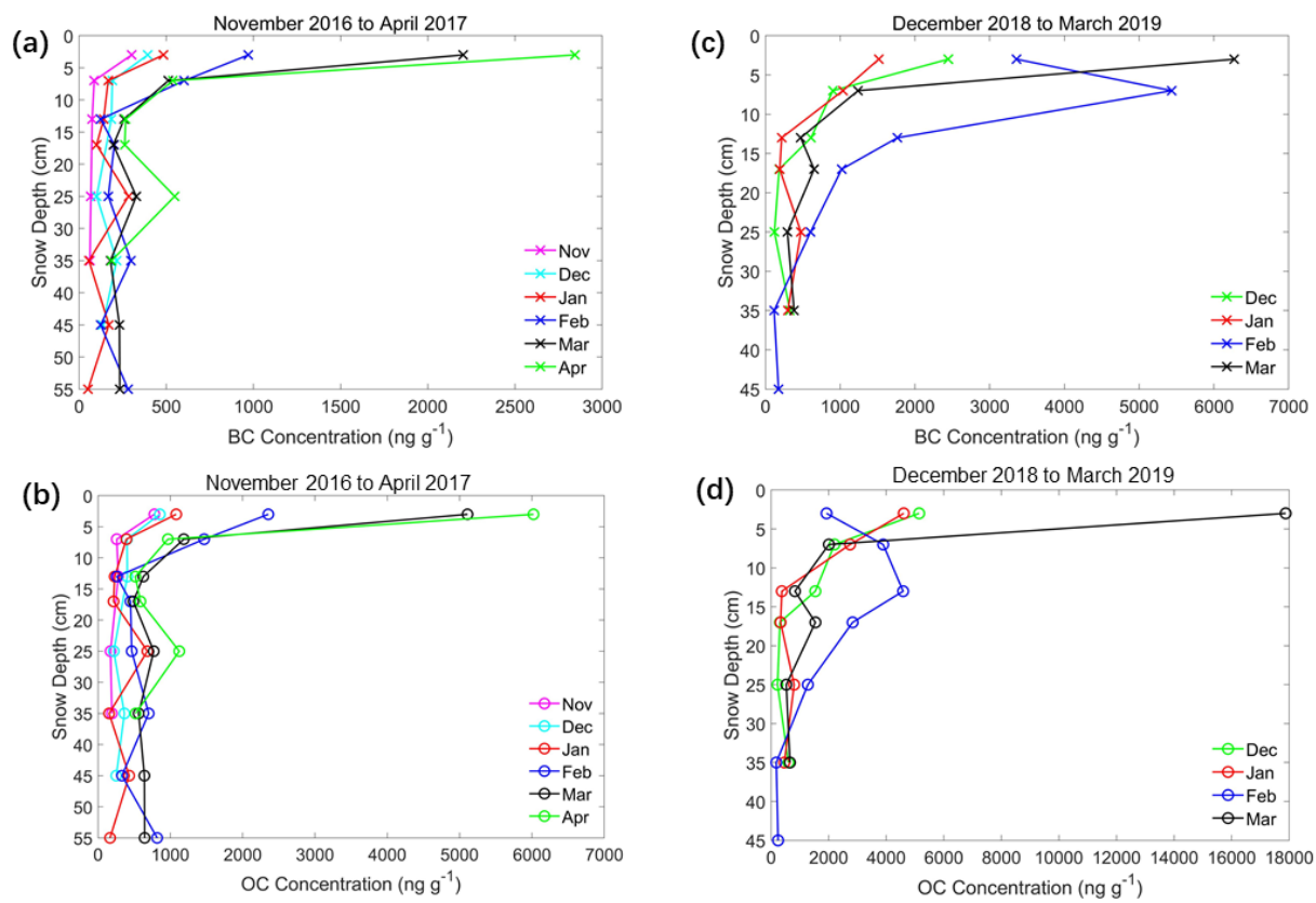
Figure 9. Vertical variations of monthly mean BC and OC concentrations in snowpits at Koktokay snow station during two snow years (Zhong et al., 2019).
