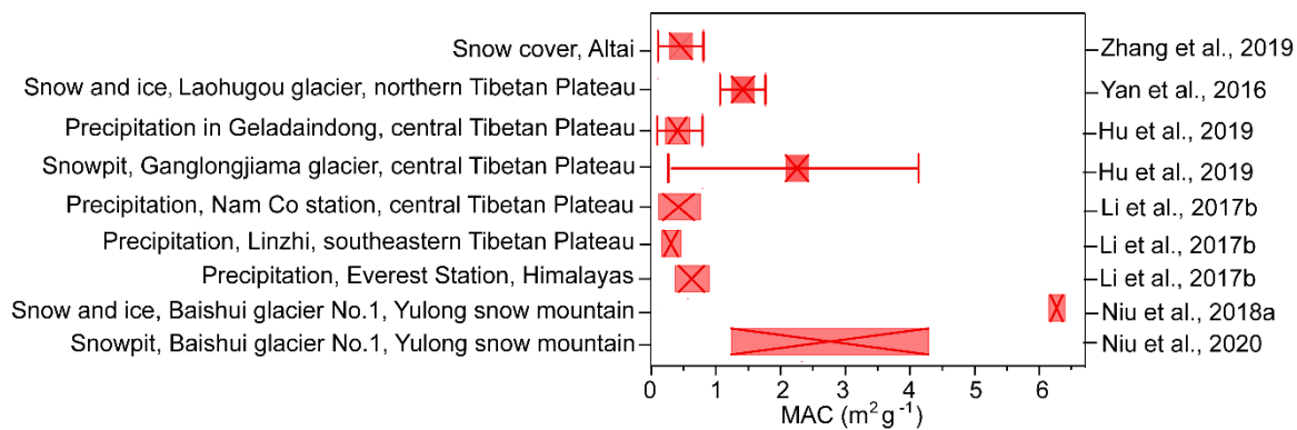
Figure 10. Comparison of the mass absorption cross section (MAC) of WSOC in snow and ice, and precipitation in the Tibetan Plateau and its surroundings.
