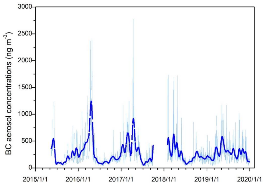
Figure 4. Daily mean BC aerosol concentrations at Everest station measured by AE-33 during May15, 2015 to December 29, 2019. Light blue lines refer to daily data; the thick blue lines represent the smoothing results.
