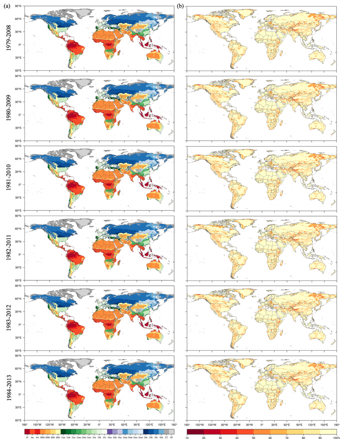
Figure 3 Global maps of the Köppen-Geiger climate classification for the historical periods (1979-2008, 1980-2009, 1981-2010, 1982-2011, 1983-2012, 1984-2013) and associated classification confidence levels. (a) Historical maps of the Köppen-Geiger climate classification and (b) confidence levels associated with the Köppen-Geiger climate classification.
