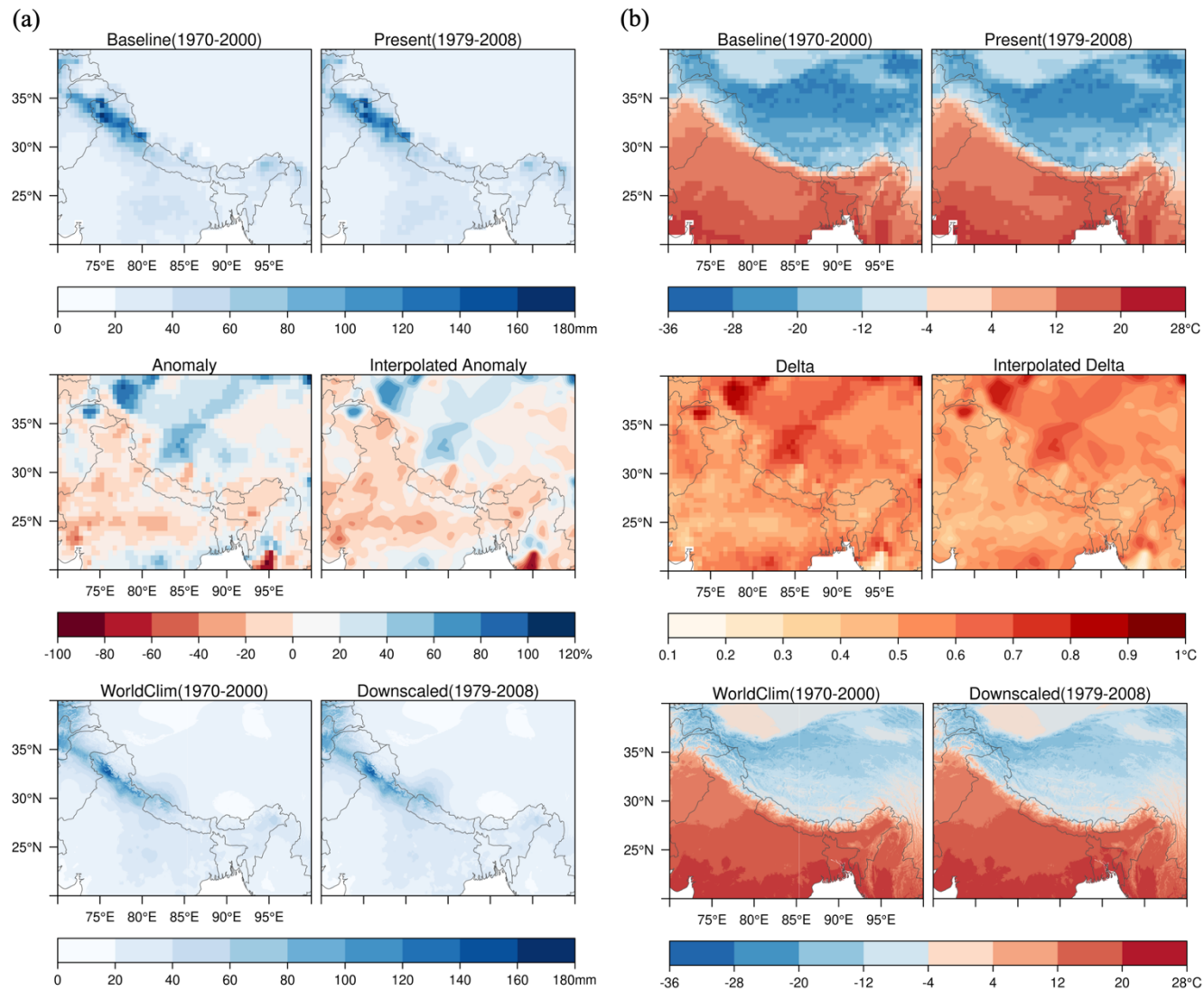
150 Figure 1. Illustration of the downscaling process. (a) Anomaly downscaling method with January total precipitation from GPCP dataset and (b) delta downscaling method with January temperature from CRU dataset. Baseline (1970-2000) and present-day climate data (e.g. 1979-2008) are from CRU, UDEL, or GPCP datasets, which have a coarse spatial resolution of 0.5°. Precipitation anomaly is change factor of monthly precipitation from baseline to present-day climates. Temperature delta is change in monthly air temperature from baseline to present-day climates. WorldClim (1970-2000) climate data is adjusted by multiplying 30 arc-second interpolated anomaly (for precipitation) or adding 30 arc-second interpolated delta (for temperature) to generate the downscaled climate surfaces with 30 arc-second resolution. 155 Precipitation values in mm/month and temperature values in °C.
