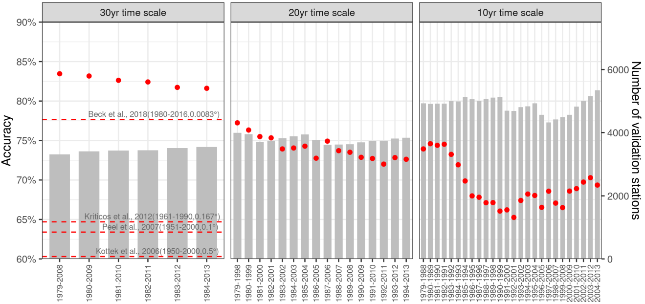
295 Figure 7. Validation of downscaled data of bioclimatic variables and the generated Köppen-Geiger climate map.
