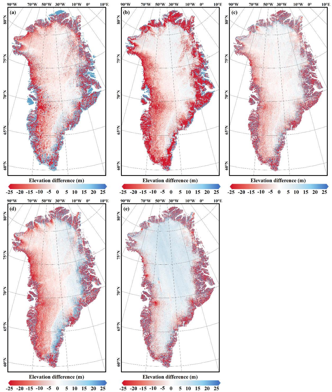
415 Figure 7: Elevation differences calculated between the new ICESat-2 DEM and the other five published available DEMs. (a) ICESat DEM, (b) CryoSat-2 DEM, (c) 500 m ArcticDEM, (d) 1 km ArcticDEM, and (e) TanDEM-X. For each picture, the previously published DEM was resampled to 500 m, and the difference was calculated as the resampled DEM subtracted from the new ICESat-2 DEM.
