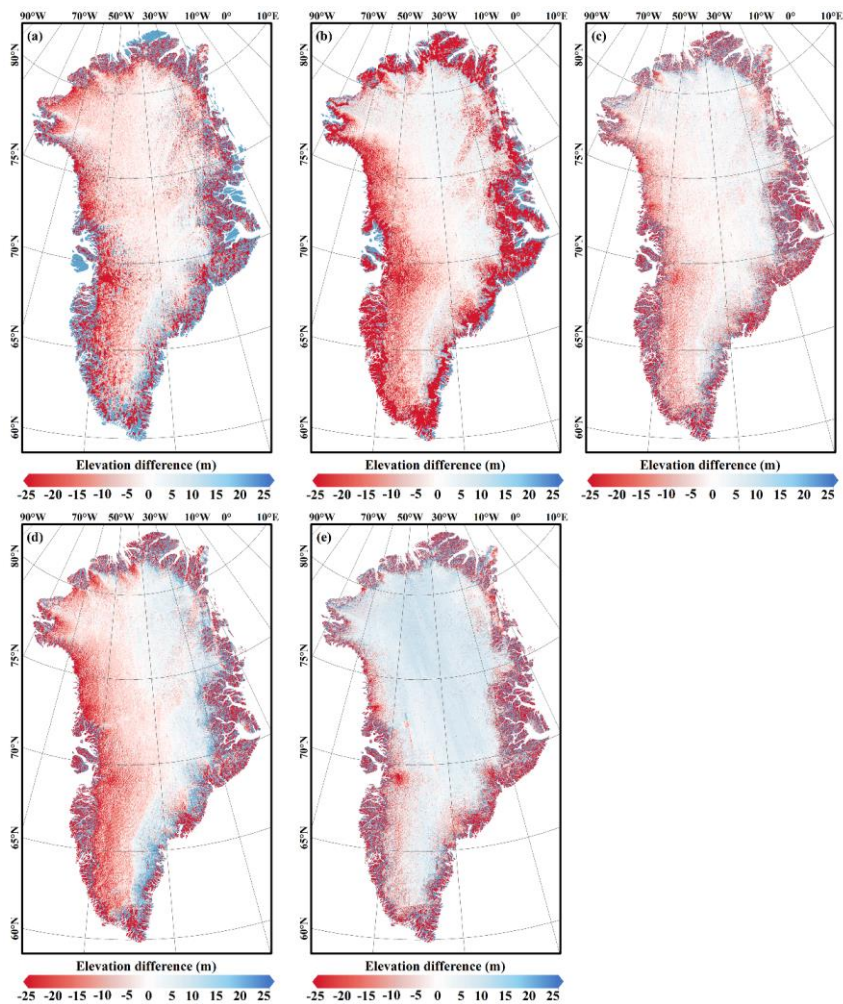
465 Figure 7: Elevation differences calculated between the new ICESat-2 DEM and the other five published available DEMs. (a) ICESat DEM, (b) CryoSat-2 DEM, (c) 500 m ArcticDEM, (d) 1 km ArcticDEM, and (e) TanDEM-X. For each picture, the previously published DEM was resampled to 500 m, and the difference was calculated as the resampled DEM subtracted from the new ICESat-2 DEM.
