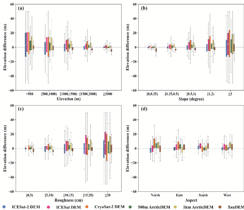
470 Figure 8: Elevation differences between different DEMs and IceBridge data under different terrain conditions. (a) Elevation, (b) slope, (c) roughness, and (d) aspect. The solid black lines near the box centres denote median values of elevation differences, the upper and lower boundaries of each box denote upper and lower quartiles (Q1 and Q3), the length means the interquartile range (IQR), and the top and bottom lines denote the range [Q1-1.5 IQR-Q3+1.5 IQR].
