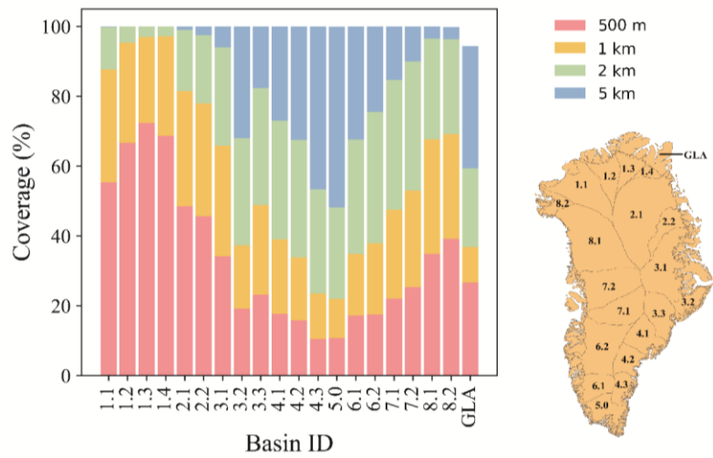
450 Figure 3: Coverage percentages of calculated elevation grids by ICESat-2 observations of 500 m, 1 km, 2 km, and 5 km. The basin boundaries are from Zwally et al. (2002), which divides Greenland into 8 main basins, covering approximately 1.72 \times 10^6 km 2 . Ice caps and glaciers that are not connected with the ice sheet are marked as GLA.
