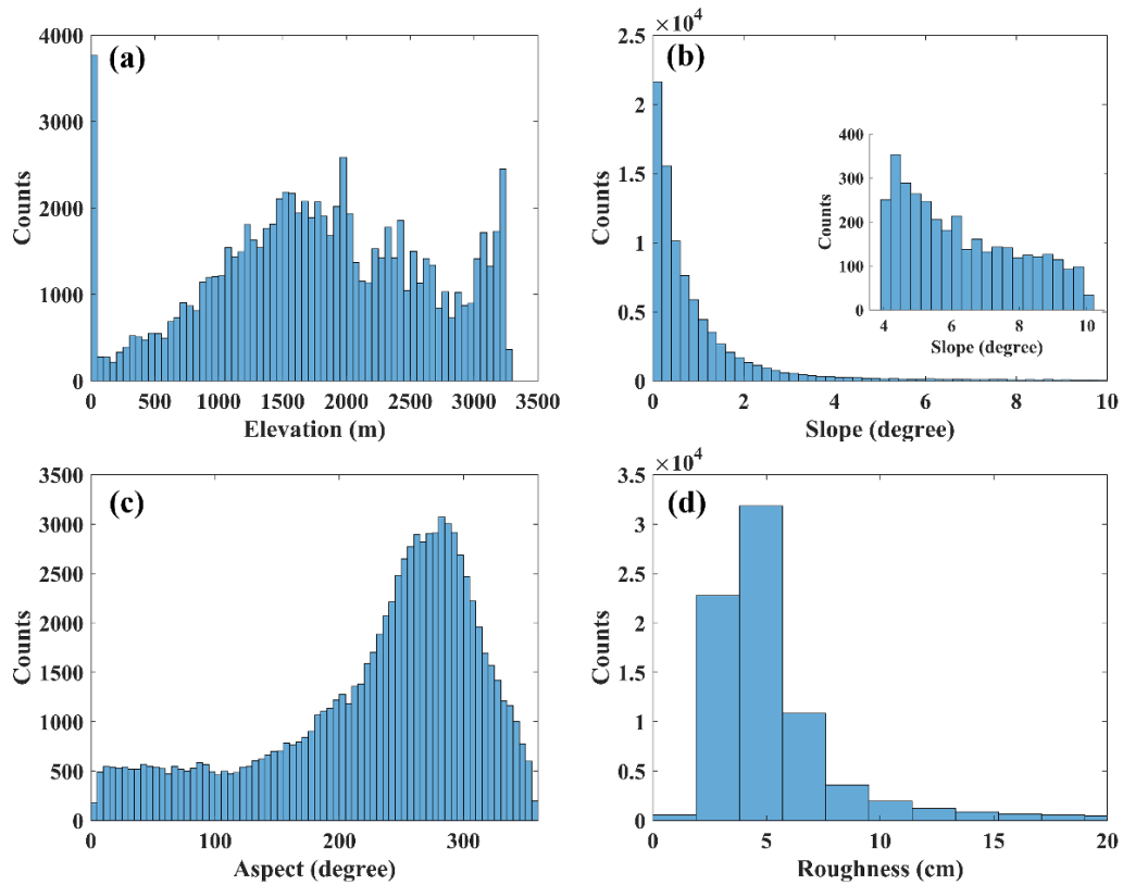
395 Figure 2: Histogram of the (a) surface height, (b) surface slope, (c) aspect, and (d) roughness derived from IceBridge data. The inset figure shows the histogram of surface slope between 4^\circ and 10^\circ .
