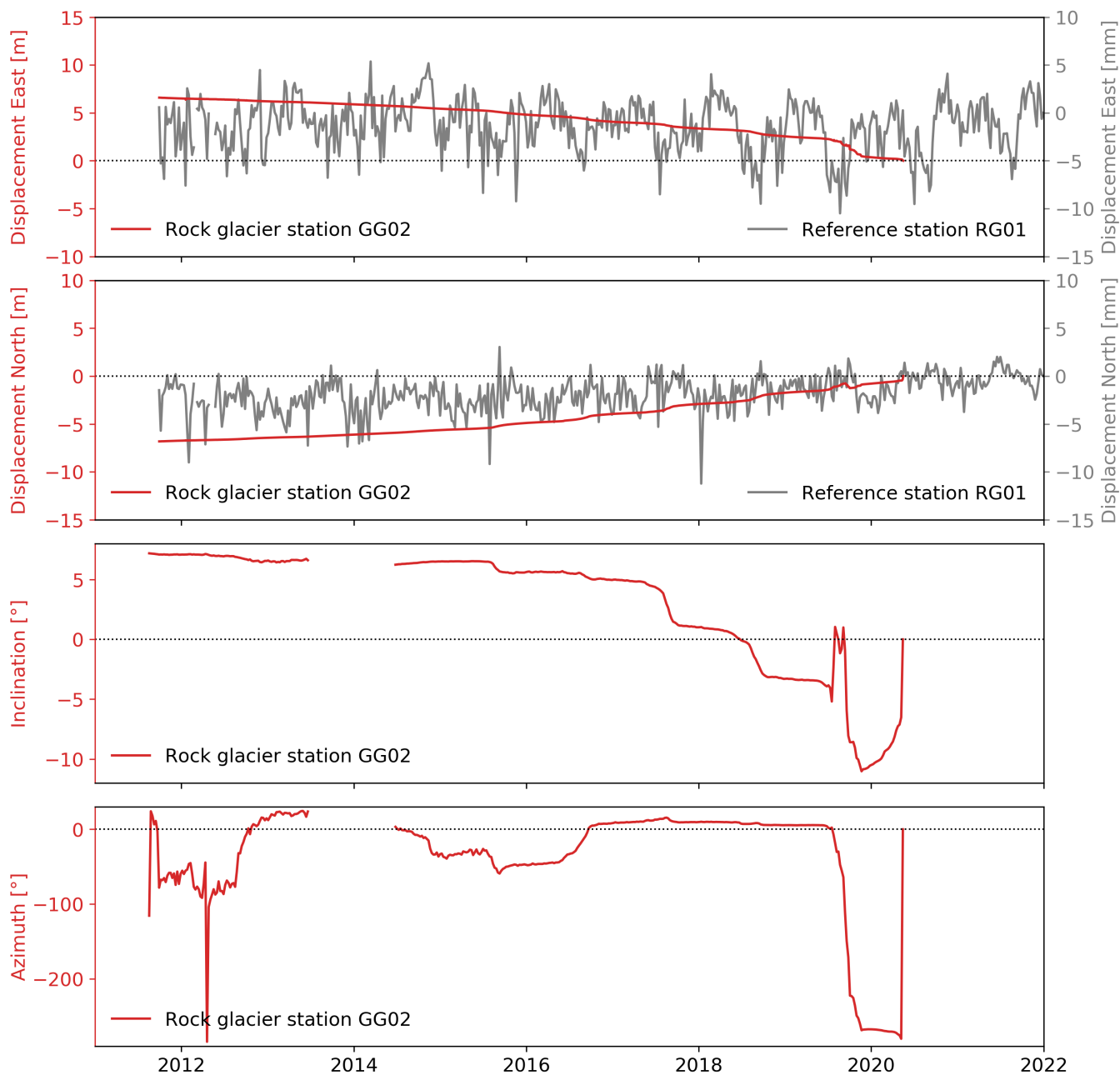
Figure B2. A decade of displacement, inclination and azimuth for the Grabengufer Rock Glacier (position GG02) In year 2020 the boulder where the GNSS station was installed showed an anomalous behaviour and strong acceleration until falling into the gully. The data show this process until the last day.
