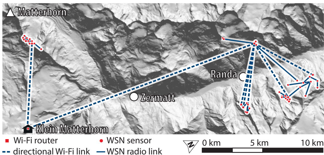
Figure A6. Wireless LAN backbone and fine distribution of wireless connectivity to all sensor locations in the Matter Valley. Base for such connection is a WLAN access point located at the cable car station of the Klein Matterhorn 3883m a.s.l. about 6.5 km away where the network is attached to a local Internet service provider using glass fiber. In a previous publication, Weber et al. (2019a) provided a more comprehensive and detailed description of the technology of the wireless sensor network.
