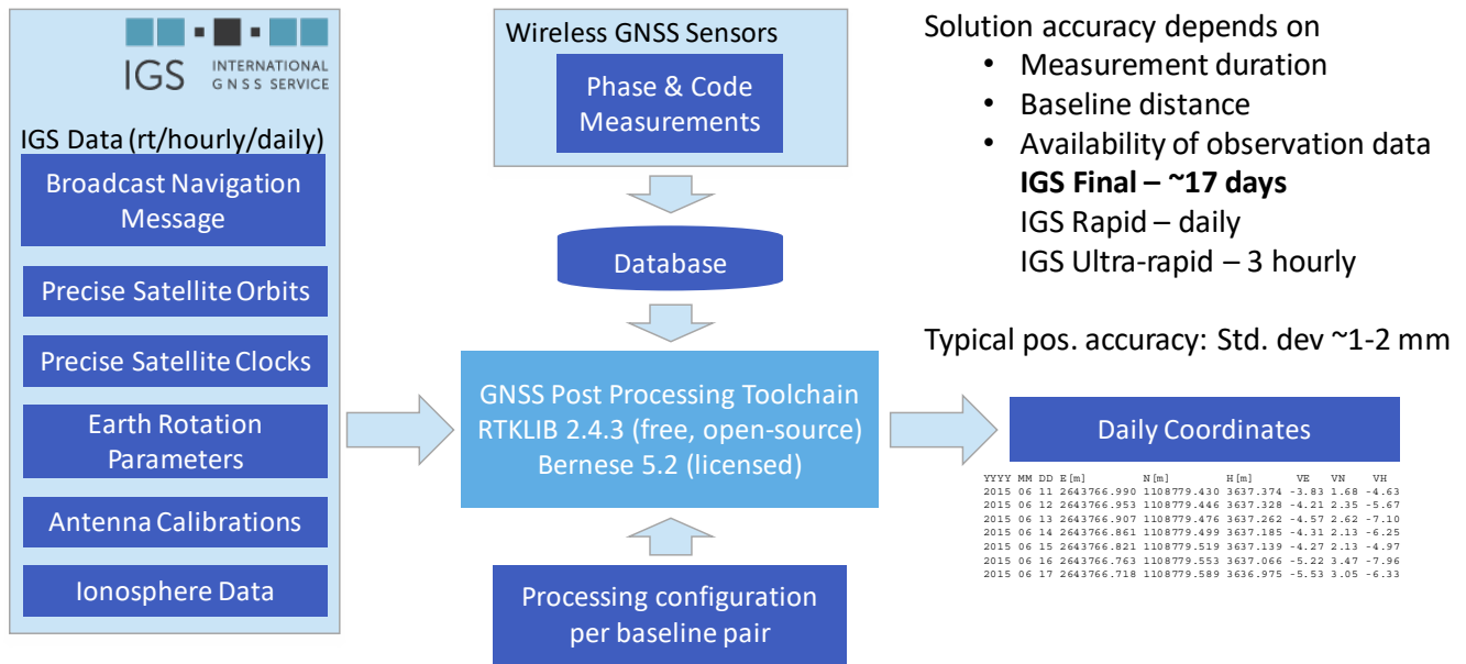
Figure 5. Typical GNSS post-processing workflow using the Bernese GNSS Software or RTKLIB.
