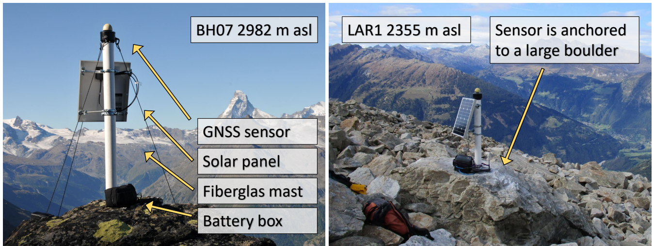
Figure 3. Two GNSS stations mounted atop large boulders on the Breithorn landslide 2982 m a.s.l., Herbruggen (left) and on the Largario Rock Glacier 2355 m a.s.l., Val di Blenio (right) illustrate how a field deployment including all sensor set-up and anchoring appears.
