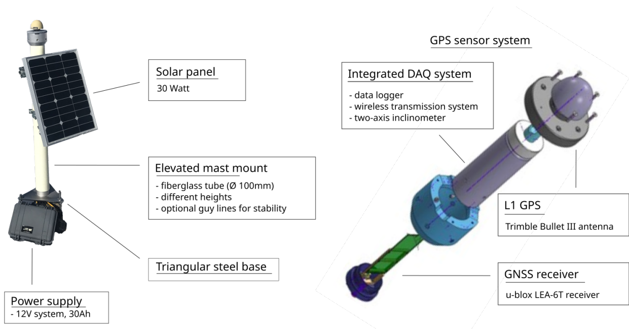
Figure 1. Structure and components of the GNSS sensor system developed in the PermaSense Project. (Left) Structure of the GNSS station. (Right) Detail of the embedded GNSS antenna, data logger, and wireless transmitter.
