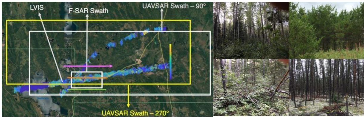
59 60 Figure 5. LEFT: Experimental design for the BERMS area TomoSAR flights in August 2018. The large White and yellow 61 boxes show the ~18 km-wide UAVSAR L-band swaths. The offset is due to the off-nadir viewing angle of the L-band SAR – 62 it is pointed to the south when flying the 270° swath and pointed north when flying the 90° swath. The small white box near 63 the center of the image marks the ~3 km-wide F-SAR swath. LVIS LiDAR data are the ~1.5 km-wide colored swaths across 64 the image; the color scaling reflects the canopy height. RIGHT: Photos from four of the 17 plots used for in situ ground truth 65 measurement at BERMS. Vegetation at BERMS was mostly Jack Pine and Aspen with many areas having dense understory 66 vegetation. Most areas have substantial detritus and ground litter left over from previous logging operations. © Google Earth
