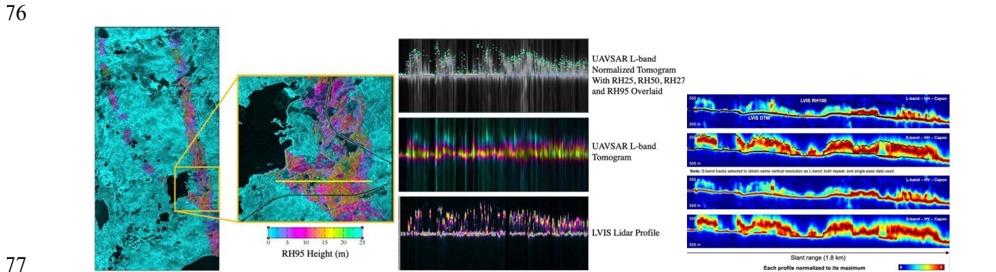
77 78 Figure 6. On the left shows location of transect as yellow line overlaid on UAVSAR imagery in grayscale and LVIS RH95 data is color 79 where UAVSAR L-band, DLR F-SAR L and S-band and LVIS LiDAR profiles are compared. Center figure shows UAVSAR L-band 80 tomographic profiles along the transect along with the corresponding LVIS LiDAR profiles. On the right are the corresponding F-SAR L 81 and S-band tomographic profiles. The L-band radar profiles exhibit power concentrated at the base of the canopy whereas the LVIS LiDAR 82 data show more return from the middle portion of the canopy. S-band obtains greater returns in the upper canopy compared to L-band and 83 show more uniform scattering within the canopy.
