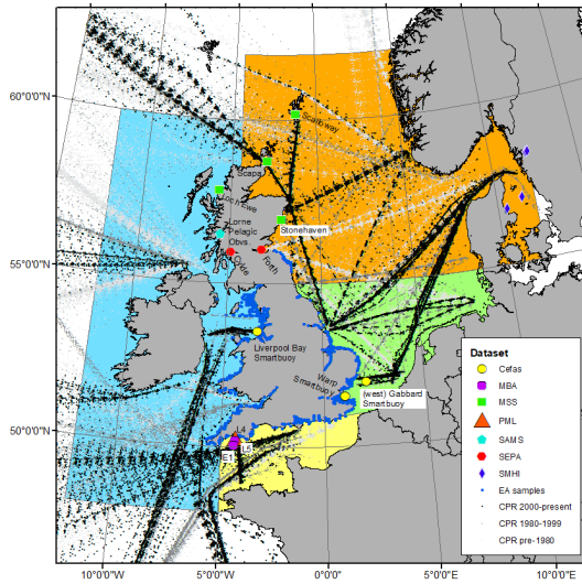
140 Figure 1. Spatial coverage of plankton measurements currently integrated with the PLET tool for lifeform extraction. See data provider and station information in Table 1 , individual station names are given next to the symbols, while symbols designate data providers as shown in the legend. The sampling transects for the CPR are coloured by date sampled, with pre-1980 in light grey, 1980-1999 in darker grey, and the most recent 2000-onwards in black. Coloured regions indicate how data are summarised for presentation of Lifeform outputs in Section 6 : blue: Celtic Seas; red: northern North Sea; green: southern North Sea; light yellow: Channel.
