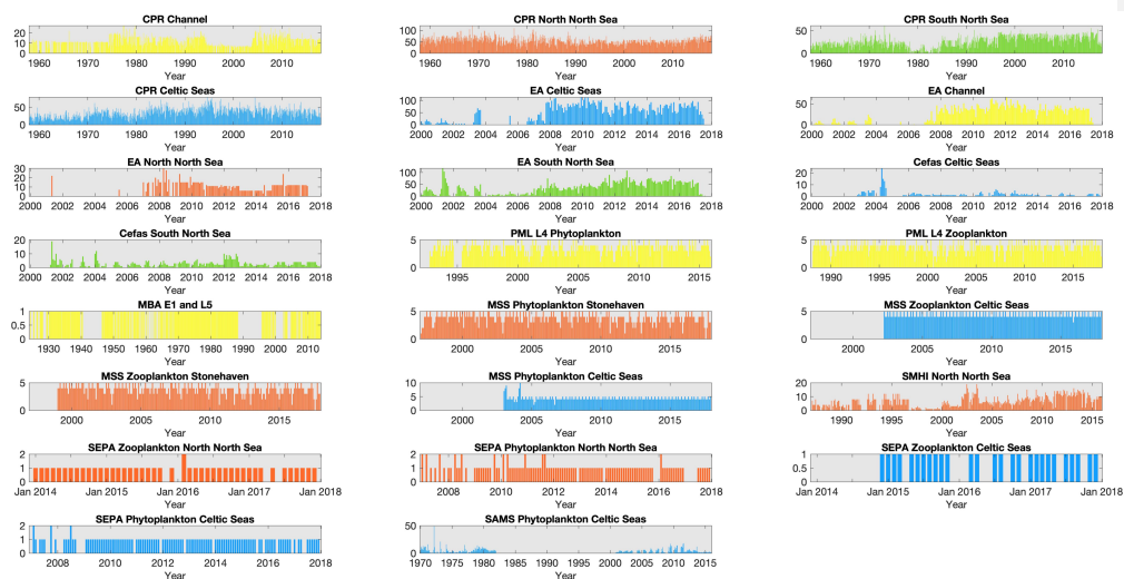
75 Figure 2. Sampling effort of each dataset within each region: number of sampling timepoints collected per month for each dataset within each of the regions defined in Figure 1 , except for MSS stations in the northern North Sea where only Stonehaven is shown as an example of the three MSS stations in that region. Note that axis limits are not fixed between panels. Bar colour indicates spatial region (see Figure 1 ); blue: Celtic Seas; red: northern North Sea; green: southern North Sea; light yellow: Channel.
