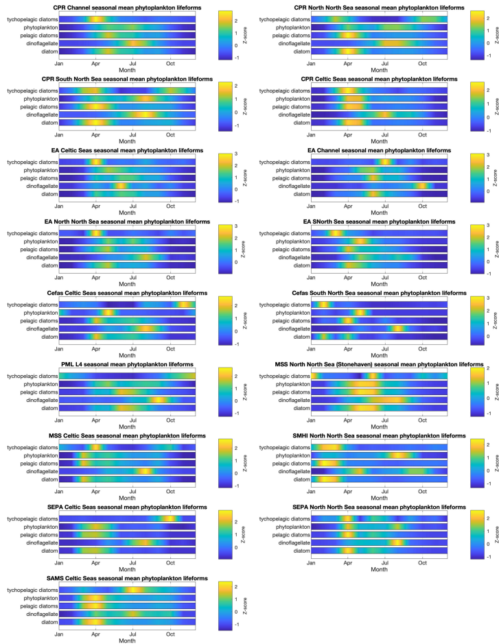
520 Figure 5. Phytoplankton lifeform monthly means, by data provider and region. Colour indicates lifeform abundance relative to the long-term mean of each lifeform within each region and dataset as standardised z-score (Glover et al., 2005); Scores of zero are equal to the long-term mean, positive scores (in green/yellow) signify values above the long-term mean and negative scores values below the long-term mean (in blue). Only those lifeforms that have been assigned a confidence level of 'high' are shown (see Table 2 and Table 3). Regions are defined in Figure 1.
