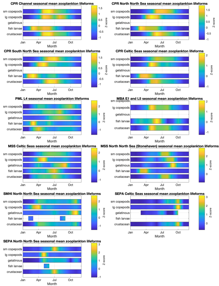
525 Figure 6. Zooplankton lifeform monthly means, by data provider and region. Colour indicates lifeform abundance relative to the long-term mean of each lifeform within each region and dataset as standardised z-score (Glover et al., 2005); Scores of zero are equal to the long-term mean, positive scores (in green/yellow) signify values above the long-term mean and negative scores values below the long-term mean (in blue). Only those lifeforms that have been assigned a confidence level of 'high' are shown (see Table 2 and Table 3 ). Regions are defined in Figure 1 .
