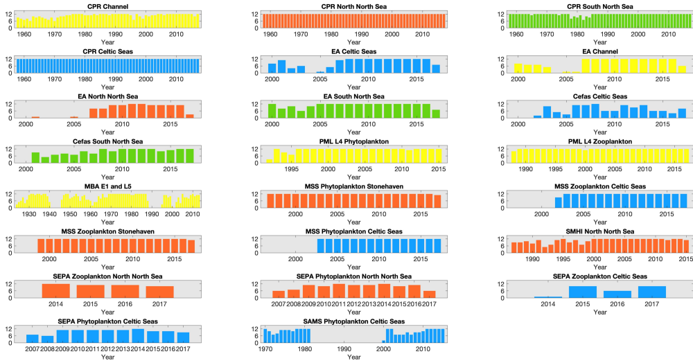
35 Figure 3. Number of months sampled per year for each dataset within each region: number of months sampled within each year, for each dataset within each of the regions defined in Figure 1 , except for MSS stations in the northern North Sea where only Stonehaven is shown as an example of the three MSS stations in that region. Widths of the bars indicate the total time-series length. Bar colour indicates spatial region (see Figure 1 ); blue: Celtic Seas; red: northern North Sea; green: southern North Sea; light yellow: Channel.
