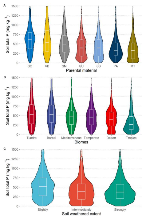
220 Fig. 2 Soil total P concentration in relation to parent material, biome, and soil weathering extent. For visualization, we chose to limit the y-axis to 1500 mg kg -1 ; and in panel A, only parent material types with more than 100 measurements in our database were shown; the abbreviations in figure (A) represent the following: SC: Carbonate sedimentary; VB: Basic volcanic; SM: Mixed sedimentary; SU: Unconsolidated sediments; SS: Siliciclastic sedimentary; PA: Acid plutonic; MT: Metamorphics.
