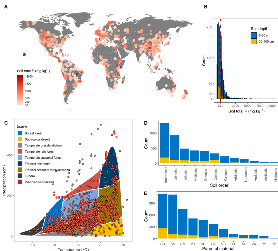
130 Fig. 1 The distribution of our site-level training data. The database contains 5,275 observations (A & B) covering all major terrestrial biomes (C), 12 soil orders (D), and 12 parent materials (E). Red dashed line in figure (B) indicates the arithmetic mean of the soil total P concentration ( 570 \text{ mg kg}^{-1} ). The abbreviations in figure (E) represent the following: SS: Siliciclastic sedimentary; SU: Unconsolidated sediments; SM: Mixed sedimentary; MT: Metamorphics; SC: Carbonate sedimentary; PA: Acid plutonic; VB: Basic volcanic; VI: Intermediate volcanic; PI: Intermediate plutonic; VA: Acid volcanic; PY: Pyroclastics; PB: Basic plutonic.
