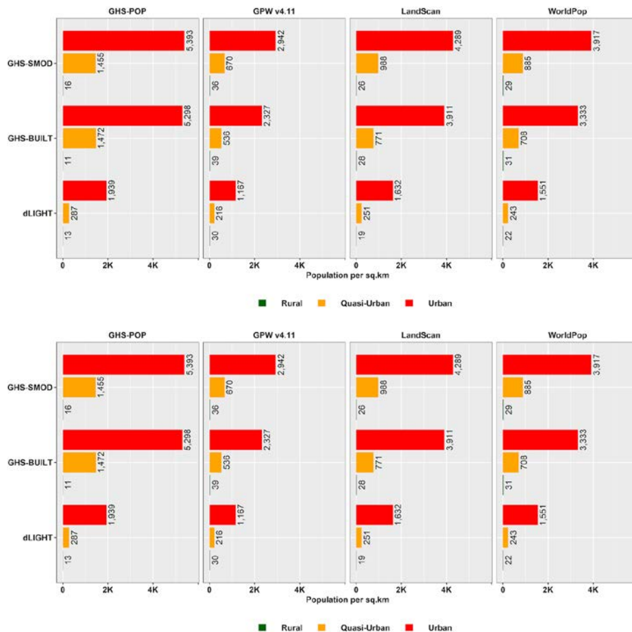
Figure 13b. Population density of urban, quasi-urban and rural areas by urban proxy data sets (y-axis) and population data (x-axis).
