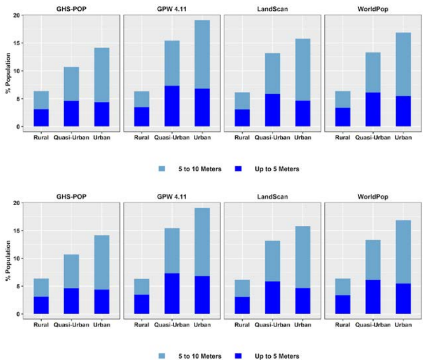
Figure 12b. ProportionPercentage of population in each urban class (urban, quasi-urban and rural) in the \leq 5\text{m} and 5-10m LECZ, by each respective urban-rural class, according to different Population and Urban Proxy data sets, 2015. (GHS-SMOD is used for the urban proxy and MERIT is used for LECZ delineation.)
