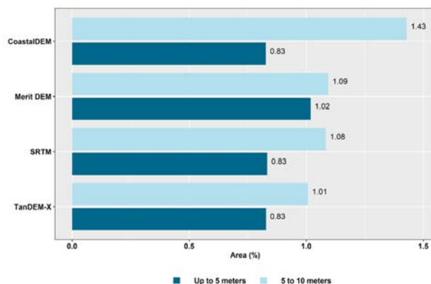
Figure 8. Proportion Percentage of total land area in the ≤5m and 5-10m LECZ, by different elevation sources.
