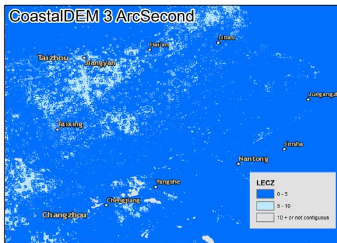
Figure B2. Raw TanDEM-X captures roadways, whereas CoastalDEM seems to capture agricultural land uses.
