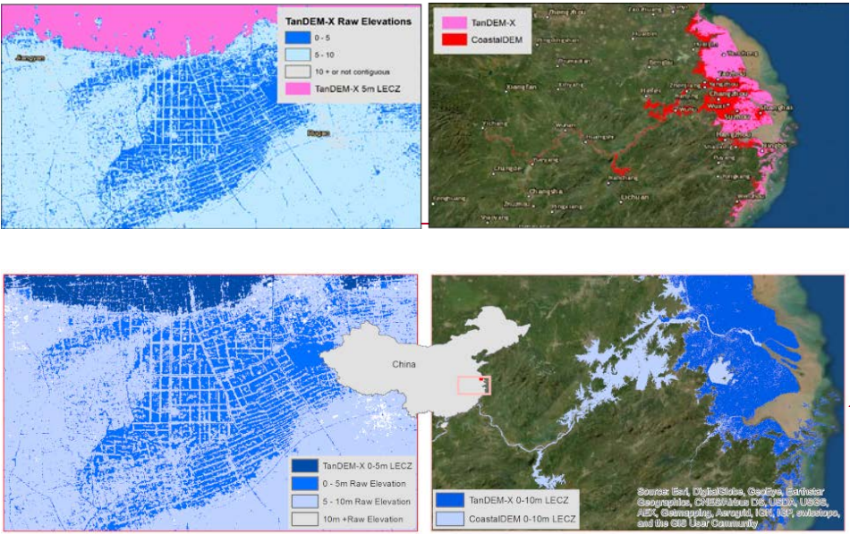
Figure 10. Comparison of coastal-contiguity in LECZ data sources along the Yangtze River, China for CoastalDEM and TanDEM-X elevation sources. Basemap from Esri, DigitalGlobe, GeoEye, Earthstar Geographics, CNES/Airbus DS, USDA, USGS, AEX, Getmapping, Aerogrid, IGN, IGP, swisstopo, and the GIS User Community.
