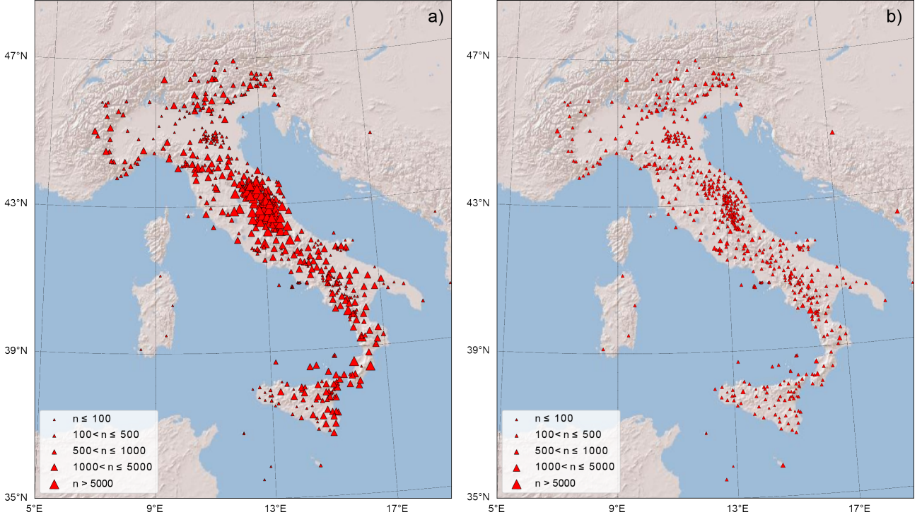
Figure (2). Map of the stations used to assemble the events (a) and noise (b) datasets. The symbol size in (a) is proportional to the number of P-phases and corresponding waveform traces available for each station. In (b) the symbol size is proportional to the number of traces. A total of 620 stations are included.
