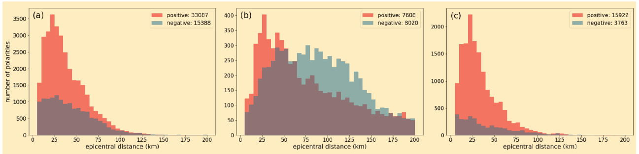
Figure (C1). Distribution of the positive and negative P-wave polarities for earthquakes with M > 2.5 in the Apennines region ( 41^\circ\text{N} - 44^\circ\text{N} and 9^\circ\text{E} - 15^\circ\text{E} ) (a); (b) as in (a) but for earthquakes outside the Apennines; (c) as in (a) but filtered by backazimuth along the NE-SW directions, corresponding to the intervals 15^\circ - 105^\circ and 195^\circ - 285^\circ .
