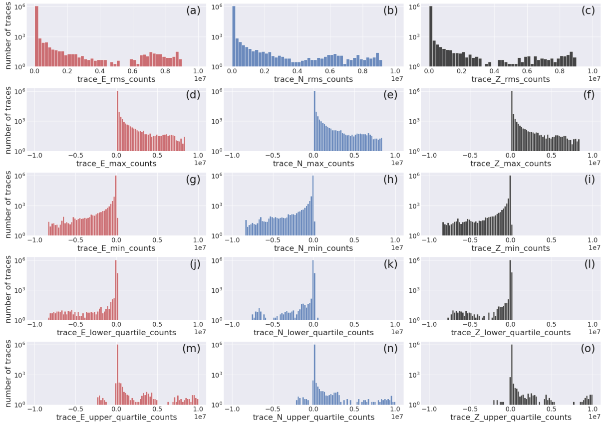
Figure (D3). Histogram of the full -distribution of quality control metadata of the event-waveforms full earthquake dataset with the horizontal axis inclusive of the complete range of values : rms, min, max, first and third quartile. The width of the bins is 2 \times 10^5 ; axes are labelled according to the metadata listed in Table 2.
