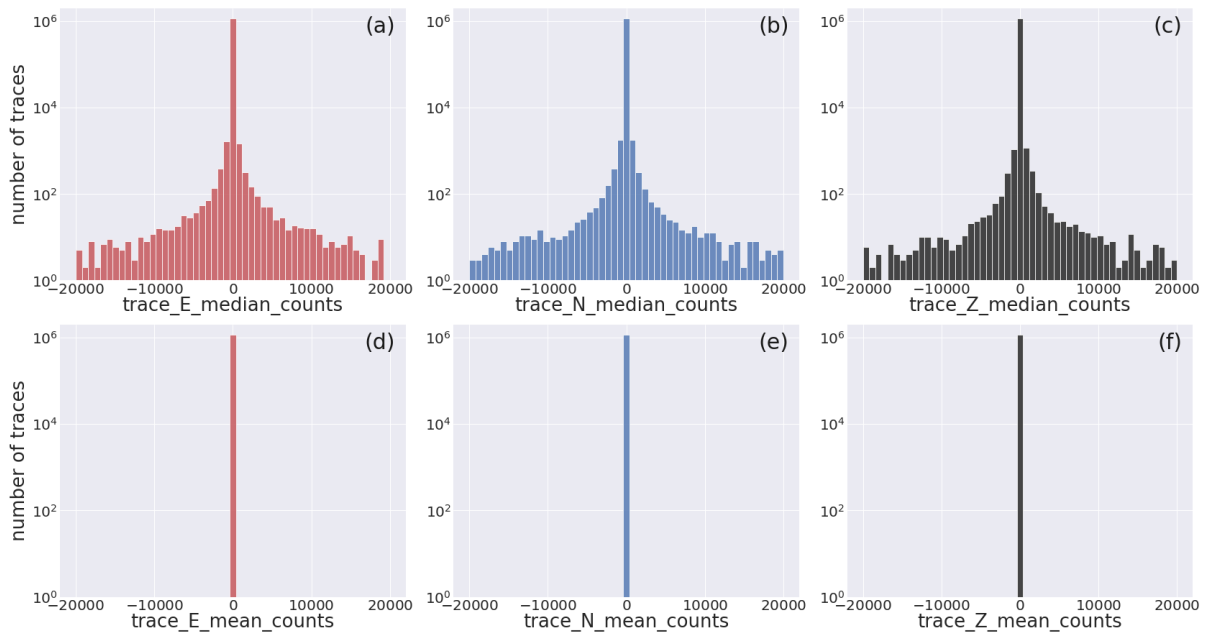
Figure (D2). Histogram of the distribution of the quality control metadata of the eventsfull earthquake dataset with the horizontal axis inclusive of the complete range of values ; median (a-c) and mean (d-f). The width of the bins is 2 \times 10^3 ; axes are labelled according to the metadata listed in Table 2 .
