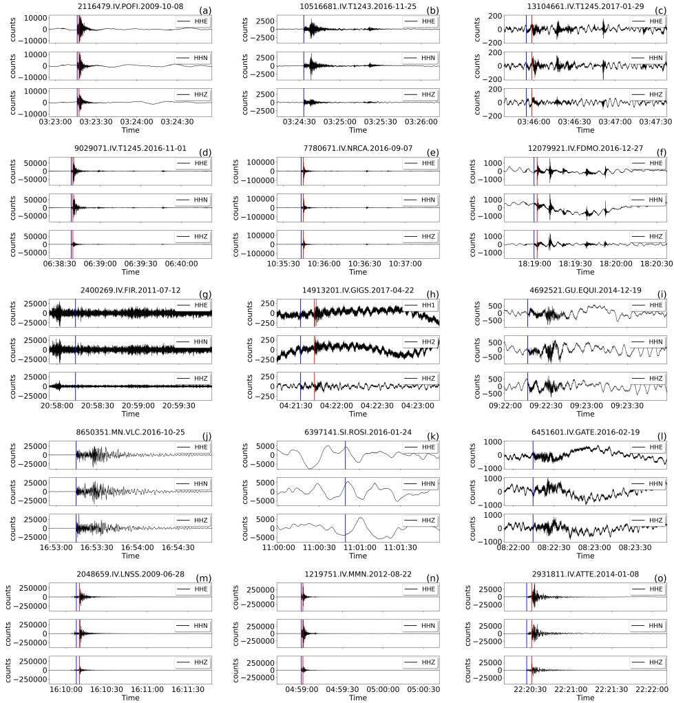
Figure (15). Example of randomly selected “problematic” earthquake waveforms of the broadband HH channels. Each row contains three randomly selected 3C traces drawn according to the following criteria based on the metadata listed in Table 2: (a-c) traces with \text{trace\_GPD}_{[P, S]}_{\text{number}} > 3 (7.96 % of the total of the HH channels); (d-f) traces with \text{trace\_EQT\_number\_detections} > 3 (0.38 % of the total of the HH channels); (g-i) traces \text{trace}_{[ENZ]}_{\text{snr\_db}} with at least one component in the 10 % quantile (18.10 % of the total of the HH channels); (j-l) traces with all \text{trace}_{[ENZ]}_{\text{median\_counts}} either in the first 10 % or the last 10 % quantiles (5.90 % of the total of the HH channels); (m-o) traces with \text{trace}_{[ENZ]}_{\text{median\_counts}} either in the first 10 % or the last 10 % quantiles and corresponding \text{trace}_{[ENZ]}_{\text{snr\_db}} excluded from the first quartile (5.06 % HH dataset). The arrival times of P- and S-wave onsets (i.e. \text{trace}_{[P, S]}_{\text{arrival\_time}} ) are shown by blue and red vertical lines, respectively.
