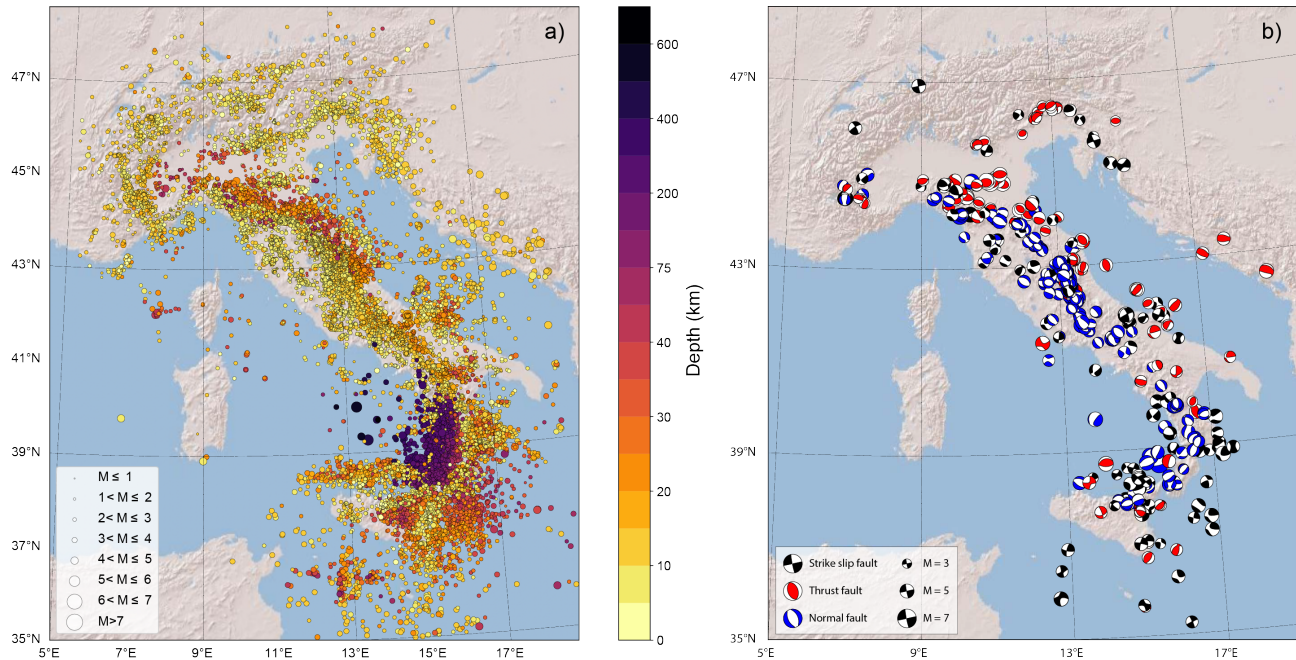
Figure (1). Earthquakes-Map of the earthquakes included in the dataset shown as solid circles with colors selected according to depth (a), and map of the available moment tensors with colors assigned depending on the focal mechanism (b) of the dataset. Symbol size, in both maps, is proportional to earthquake magnitude.
