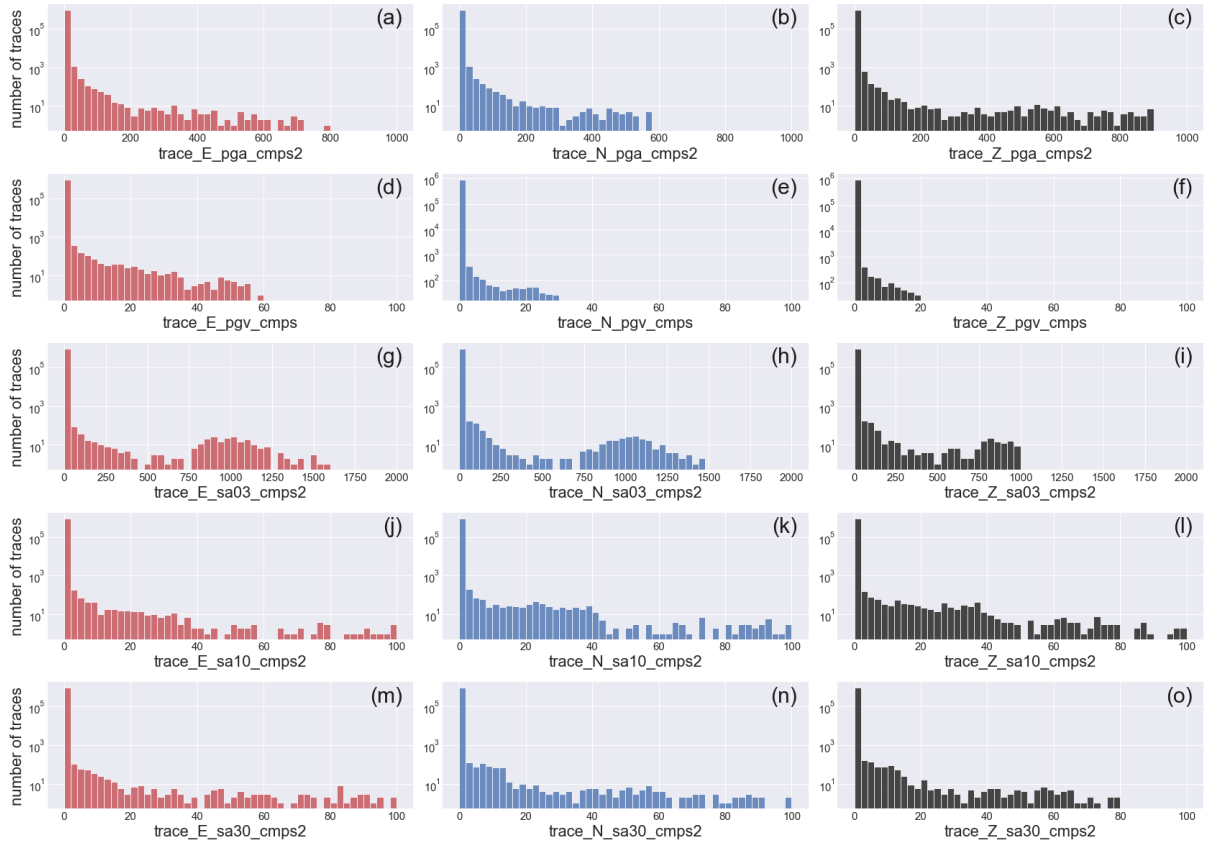
Figure (D4). Histograms of the distribution of the intensity measures (IMs) of the event waveforms earthquake dataset for M \geq 2 earthquakes with the horizontal axis inclusive of the complete range of values . Axes are labelled according to the metadata listed in Table 2 .
