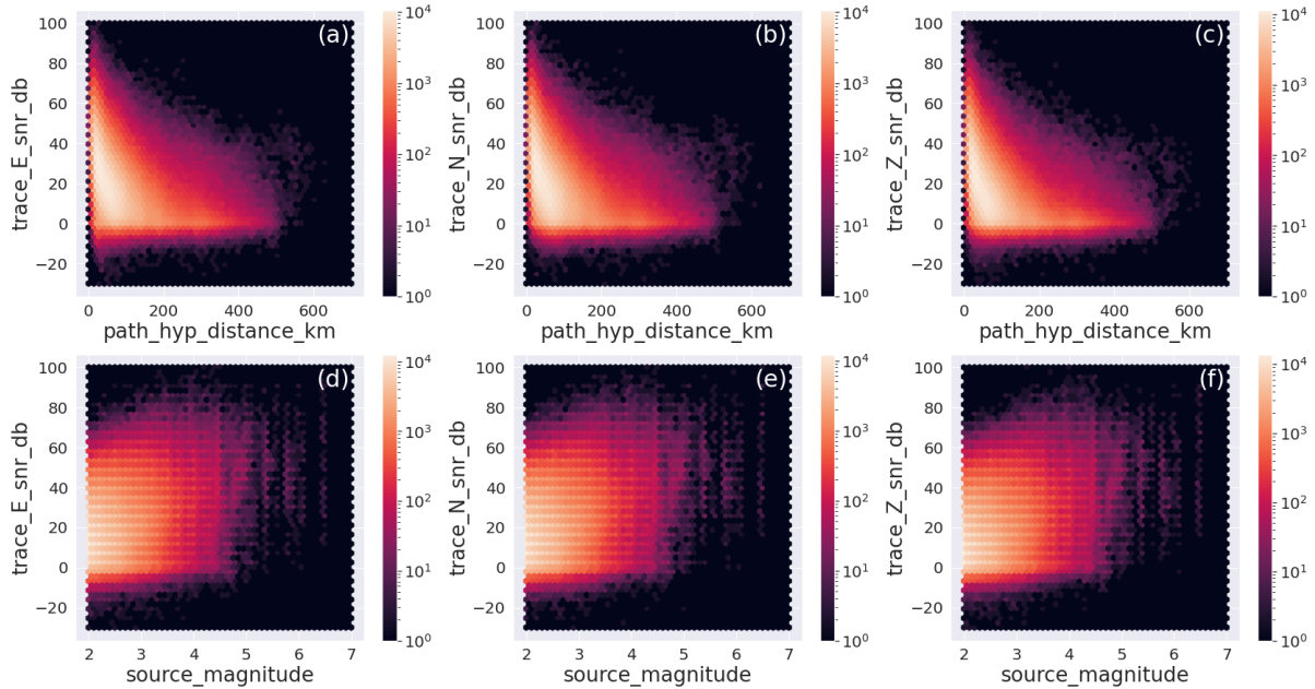
Figure (11). Hexbin representation of the distribution of the signal-to-noise ratio with for the E, N and Z components of the earthquake dataset as function of hypocentral distance distance and magnitude. The metadata names listed in Table 2 are used as labels for the specific metadata being represented.
