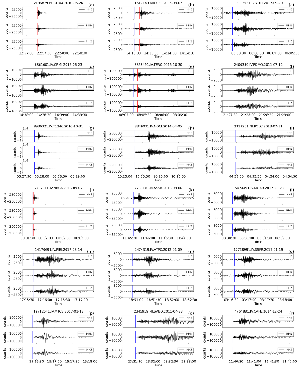
Figure (14). Example of randomly selected earthquake waveforms of the broadband HH channels contained in INSTANCE randomly drawn according to different criteria based on the metadata provided in Table 2 . Each row contains three randomly selected, 3C traces drawn according to based on the following criteria: (a-c) earthquakes 2 \leq M < 3 (66.8 % of the total of the HH channels); (d-f) earthquakes 3 \leq M < 4 (13.5 %); (g-i) earthquakes M \geq 4 (2.0 %); (j-l) earthquakes \text{trace\_E\_snr\_db} \geq 10 and \text{path\_ep\_distance} < 100 km (55.0 %); (m-o) earthquakes \text{trace\_E\_snr\_db} \geq 10 and \text{path\_ep\_distance} \geq 100 km (10.8 %); (p-r) earthquakes M \geq 4 and \text{trace\_E\_snr\_db} \geq 10 (1.7 %). The arrival times of P- and S-wave onsets ( e.g. , \text{trace\_}[P,S]\_arrival\_time ) are shown by blue and red vertical lines, respectively.
