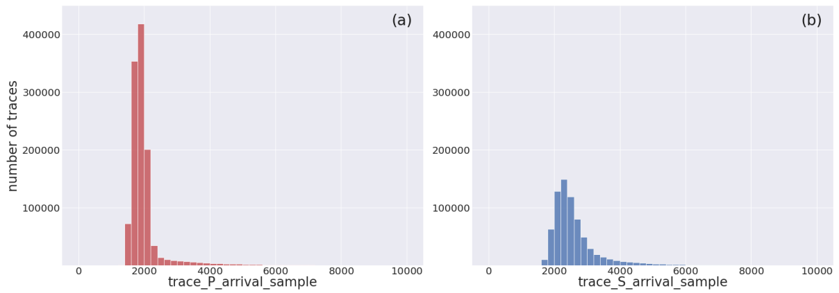
Figure (D1). Distribution of P- (left) and S-arrival (right) samples of the extracted waveform traces belonging to the earthquake dataset .
