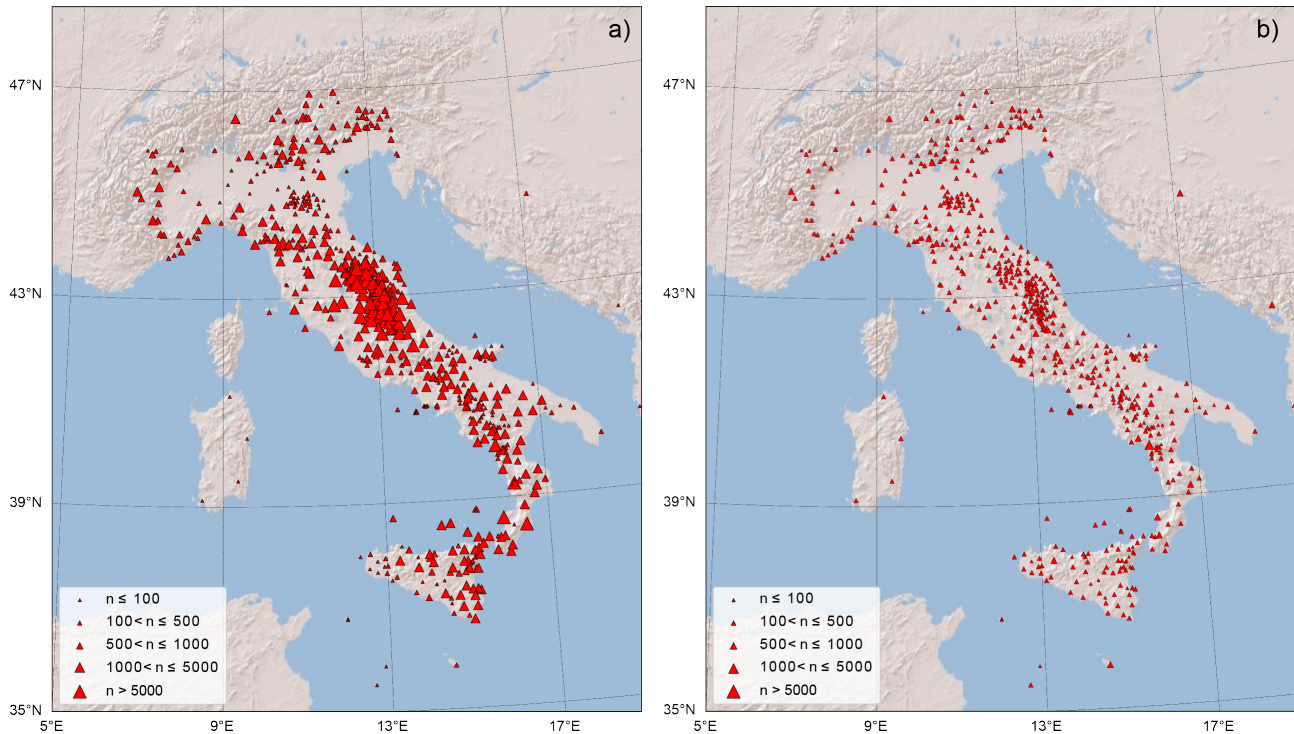
Figure (2). Stations included in Map of the stations used to assemble the events (a) and noise (b) datasets. The symbol size in (a) is proportional to the number of the number of P-phases and corresponding waveform traces available for each station. In (b) the symbol size is proportional to the number of traces. A total of 620 stations are included.
