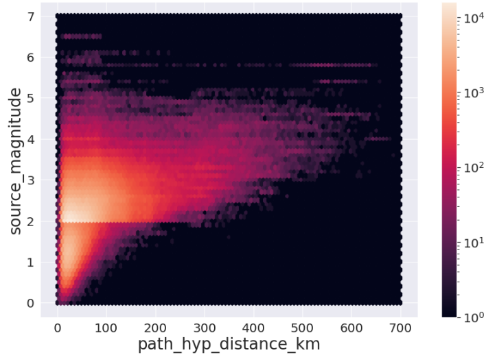
Figure (4). Diagrams Diagram of the earthquake magnitude distribution of the dataset versus receiver distance represented as hexbin plot. The labels are assigned using the metadata names listed in Table 2.
