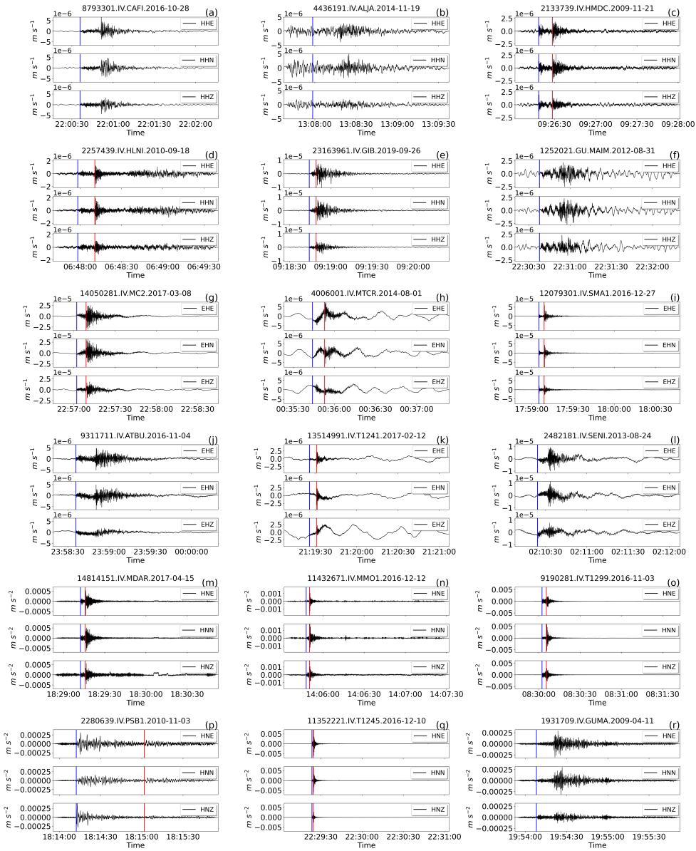
Figure (16). Example of randomly selected event waveforms in ground motion physical units of the HH, EH and HN channels in IN-STANCE. The traces are representative of 75 % of the data and belonging-belong to the second, third and fourth quartiles of each channel. Each row contains three, randomly selected, 3C traces drawn as-follows according to the following criteria based on the metadata listed in Table 2 and the quantile values provided in Table 4 : (a-f) HH traces with trace\_pga\_perc > 5.1e-4 % g; (g-l) EH traces with trace\_pga\_perc > 9.3e-4 % g; (m-r) HN traces with trace\_pga\_perc > 8.7e-4 % g; The arrival times of P- and S-wave onsets ( i.e. , trace_[P,S]_arrival_time ) are shown by blue and red vertical lines, respectively.
