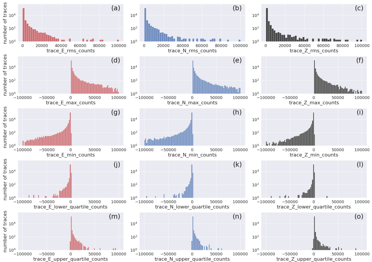
Figure (19). Histogram of the distribution of the noise-quality control metadata of the noise E, N, Z component waveform traces : rms, min, max, first and third quartile. The width of the bins is 2 \times 10^3 . The complete-full distribution of values is provided in Fig. D6. The horizontal axis labels correspond to the metadata being represented which are listed in Table 2.
