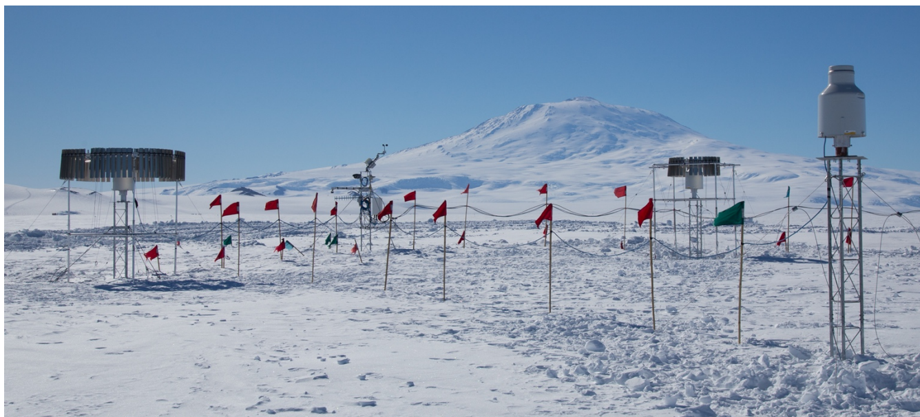
Figure 4: The modified experimental setup at the Willie Field site for the second year, at the completion of the modifications in November 2018. The three precipitation gauges are installed in a double-Alter wind shield, single- 310 Alter wind shield, and unshielded from left to right in the photo.
