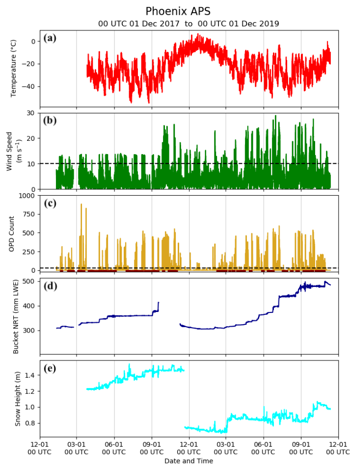
Figure 5: Time series plots of the quality-controlled data from Phoenix Airfield APS site spanning from December 2017 to November 2019. Plotted data include temperature (a), wind speed (b), particle count (c), Bucket NRT (d; see text for a description), and snow height (e). The dashed line in (b) indicates a wind speed of 10 \text{ m s}^{-1} , which is the approximate speed when there is blowing snow at the surface. The dashed line in (c) indicates a particle count of 30, which when sustained is classified as an “event” and triggers additional observations.
