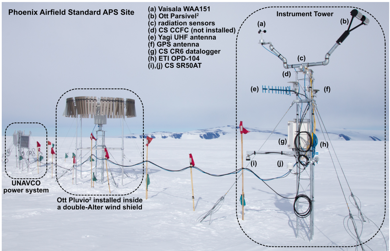
Figure 2: A complete APS standard site installation at the Phoenix Airfield site at the completion of the installation in November 2017. The UNAVCO power system is at the far left, the weighing precipitation gauge installed inside the wind shield at the center, and the instrument tower is on the right.
