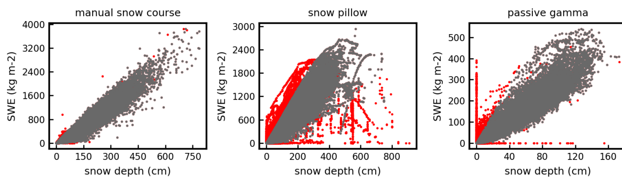
Figure 3: CanSWE data by measurement type before (red) and after (grey) quality control described in Section 2.3 and Table 5. Snow pillows are deployed in British Columbia and Alberta; passive gamma radiation sensors are used by Hydro Quebec and the Government of Newfoundland and Labrador (Sect. 2.2).
