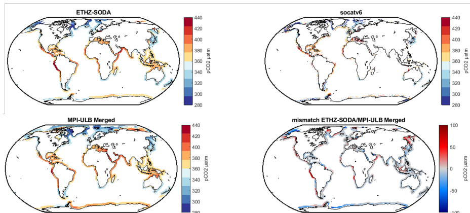
Figure A3: Spatial distributions of the annual mean p\text{CO}_2 ( \mu\text{atm} ) generated by (a) ETHZ-OceanSODA, (b) extracted from the SOCATv6 database and (c) from the MPI-ULB Merged product. (d) bias between panels (a) and (c) in \mu\text{atm} (red colors correspond to regions in which the p\text{CO}_2 from ETHZ-OceanSODA is higher than MPI-ULB Merged product). There is good agreement between the products on a regional scale.
