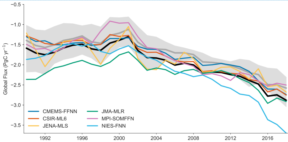
Figure 5: Global flux time series from six observation-based products. Color lines show fluxes calculated from the standardized approach presented here (spatial filling with flux calculated from three wind products and the average flux is then plotted here); the black line shows the mean of six products. The shaded region shows the spread of original flux calculations from product creators with the mean in gray.
