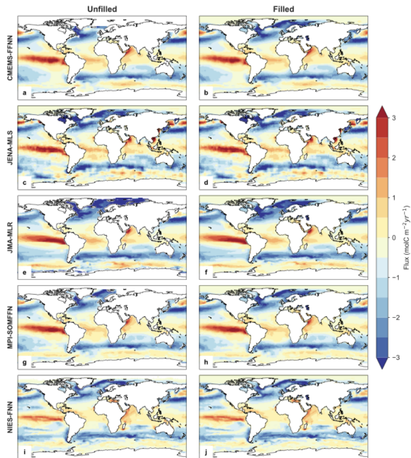
Figure A5: Mean flux ( \text{mol m}^{-2} \text{yr}^{-1} ) 1990-2019. Left-hand column: map of mean calculated flux using the unfilled \text{pCO}_2 product and 3 scaled wind products. Right-hand column: map of mean calculated flux using the filled \text{pCO}_2 product and 3 scaled wind products.
