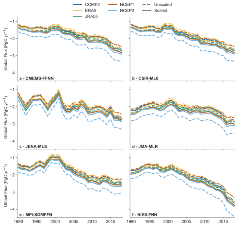
Figure A4: Air-sea CO 2 flux time series (PgC yr -1 ) calculated using five wind speed products (CCMPv2, ERA5, JRA55, NCEP1, NCEP2); scaled (solid) and unscaled (dashed).
