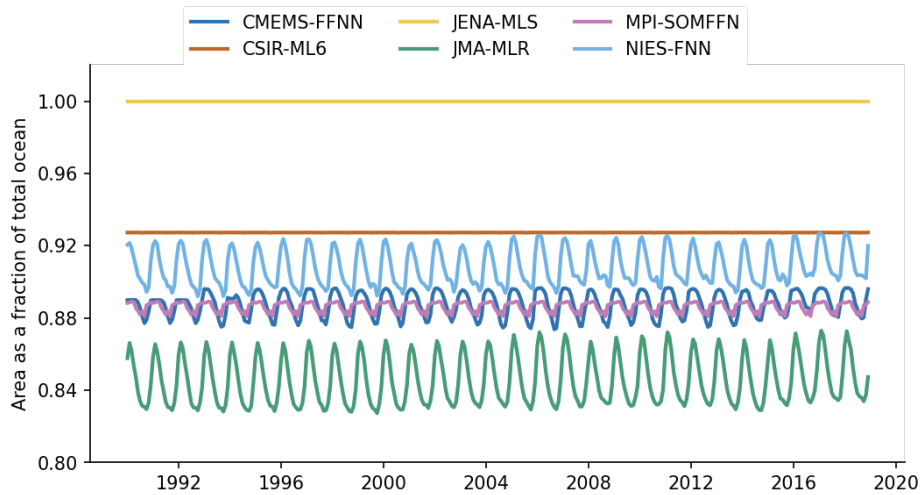
Figure A1: Time series showing the fraction of area covered by observations as a function of time (monthly) for the six pCO 2 data products used in this study.
