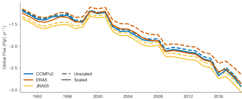
Figure 4: CSIR-ML6 product calculated air-sea CO 2 flux time series for various wind speed products; scaled (solid) and unscaled (dashed; \alpha = 0.251 ). Time series plots for all pCO 2 products and including 2 additional wind products (NCEP1 and NCEP2) are included in Figure A4.
