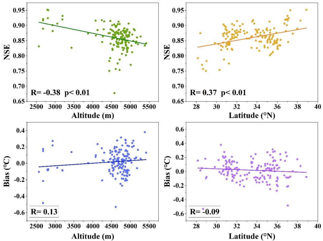
Figure S2: The NSE and bias in relation to the altitude and latitude of the lake
