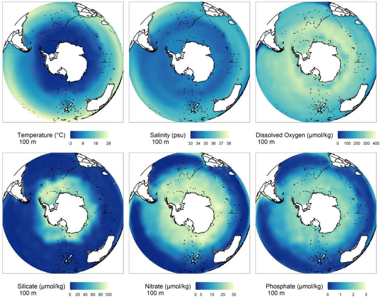
185 Figure 2: Locations of sites (black dots) and the six environmental variables at 100 m water depth used to demonstrate the environmental coverage of the SO-RAD dataset (Data source: Locarnini et al., 2018; Garcia et al., 2019a, 2019b; Zweng et al., 2019).
