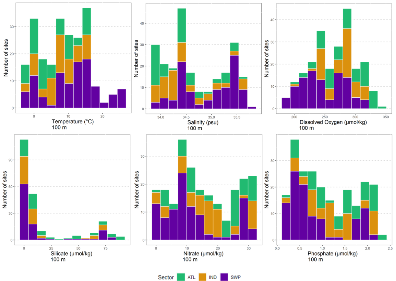
195 Figure 3: Distribution of sites across observed environmental variables at 100 m water depth (Locarnini et al., 2018; Garcia et al., 2019a, 2019b; Zweng et al., 2019) identified by sector – Atlantic Ocean sector (ATL; green), Indian Ocean sector (IND; orange), southwest Pacific sector (SWP; purple).
