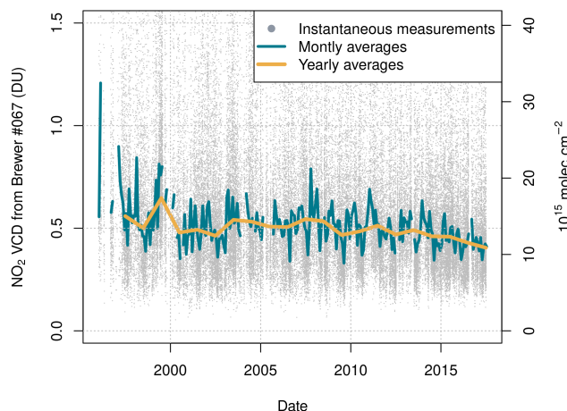
Figure 3. VCDs retrieved using BNALG2 from Brewer #067: instantaneous measurements (grey dots), monthly and yearly averages (lines).
