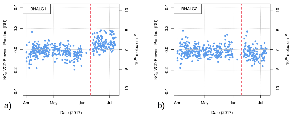
Figure 9. Difference between \text{NO}_2 retrievals from Brewer #067 - using BNALG1 (a) and BNALG2 (b) - and Pandora #117, on a portion of the data set. The vertical line shows the moment when the internal mercury lamp of Brewer #067, representing its wavelength reference, was replaced. This is sufficient to trigger a change with BNALG1, which is very sensitive to slight wavelength misalignments.
