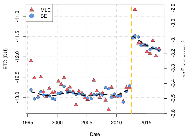
Figure 2. Extraterrestrial coefficients of Brewer #067 determined with the Minimum-Amoung Langley-Extrapolation (MLE, triangles) and Bootstrap-Estimation (BE, circles). The yellow vertical line indicates the discontinuity occurring in correspondence of the Arosa campaign in July 2012 (Sect. 2.2.1). The black dashed line represents a LOESS interpolation through the ETCs estimated by the BE method.
