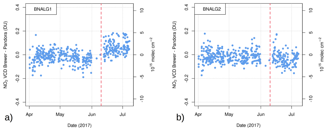
Figure 11. Difference between \text{NO}_2 retrievals from Brewer #067 – using BNALG1 (a) and BNALG2 (b) – and Pandora #117, on a portion of the data set. The vertical line shows the moment when the internal mercury lamp of Brewer #067, representing its wavelength reference, was replaced. This is sufficient to trigger a change with BNALG1, which is very sensitive to slight wavelength misalignments.
