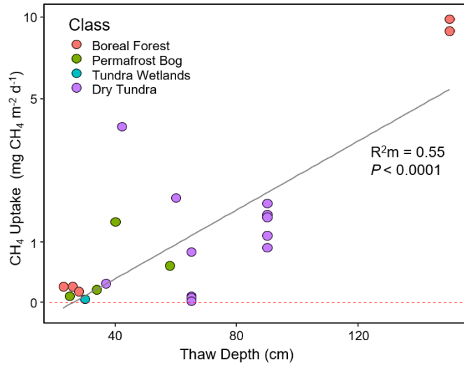
SI Figure 1. Correlation between thaw depth and methane uptake. Positive numbers represent net uptake from the atmosphere. Colors represented different ecosystem class. Neutral (i.e. zero) fluxes were not included in the regression analyses.
