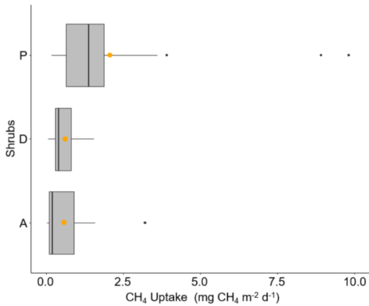
SI Figure 2. Boxplots of CH 4 uptake as a factor of shrub cover. Positive numbers represent net uptake from the atmosphere. Orange dots represent mean uptake within a given category. P = Present; D = Dominant; A = Absent. Neutral fluxes were not included in the boxplots.
