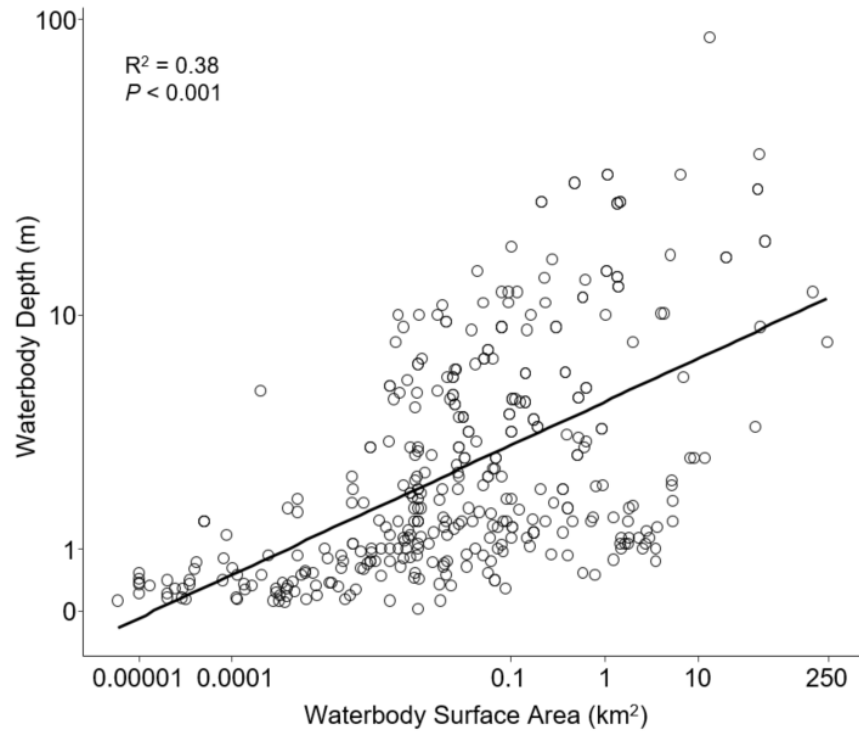
SI Figure 5. Relationship between waterbody surface area and water column depth.
