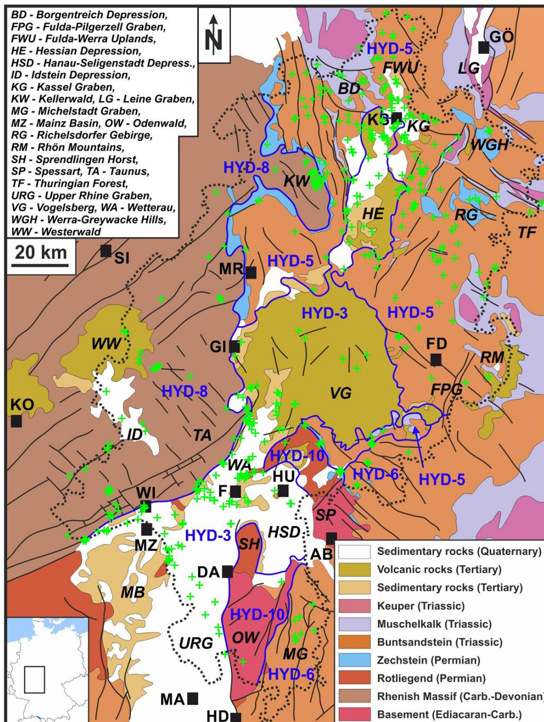
Figure 1: Hydrochemical sampling points and hydrochemical regions in the federal state of Hesse. Abbreviation of cities: AB – Aschaffenburg, DA – Darmstadt, F – Frankfurt, FD – Fulda, GI – Gießen, GÖ – Göttingen, HD – Heidelberg, HU – Hanau, KL – Kaiserslautern, KO – Koblenz, KS – Kassel, MA – Mannheim, MR – Marburg, MZ – Mainz, SI – Siegen, WI – Wiesbaden. Generalized geological map after Schäffer et al. (2018).
