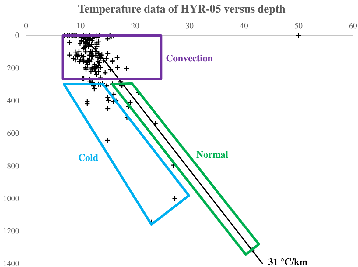
5 Figure 4: Temperature data of HYR-05 plotted against depth. Similar to HYR-03 (Figure 3) the majority of data from HYR-05 are also characterized by “convection” and/or follow the typical Hessian geothermal gradient. However, as opposed to HYR-03, neither “hot”, nor “very hot” groundwater clusters are apparent. Instead, HYR-05 shows a data cluster of “cold” groundwaters with temperatures below the typical Hessian geothermal gradient. Note that the field “convection” has been constrained rather arbitrary and not based on firm scientific evidence.
