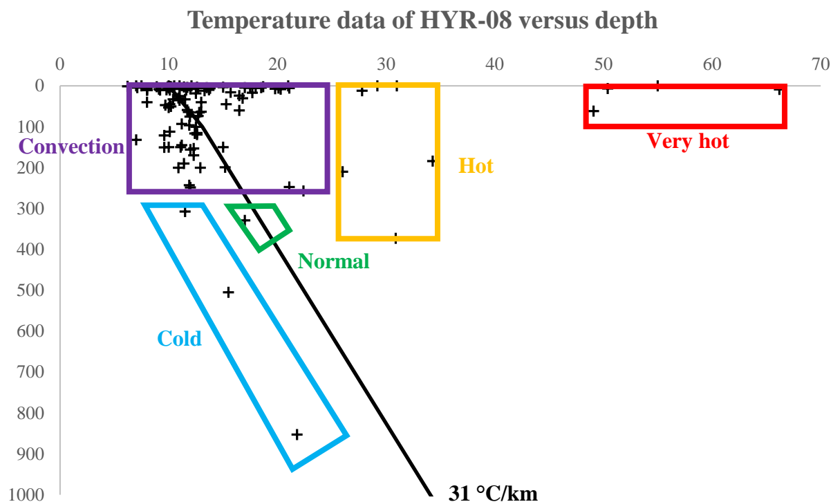
5 Figure 5: Temperature data of HYR-08 plotted against depth. Next to the clusters “hot” and “very hot” HYR-08 also shows the cluster “cold”. Only one groundwater (below 250 m bsl) shows a “normal” temperature in accordance with the typical Hessian geothermal gradient. Note that the field “convection” has been constrained rather arbitrary and not based on firm scientific evidence.
