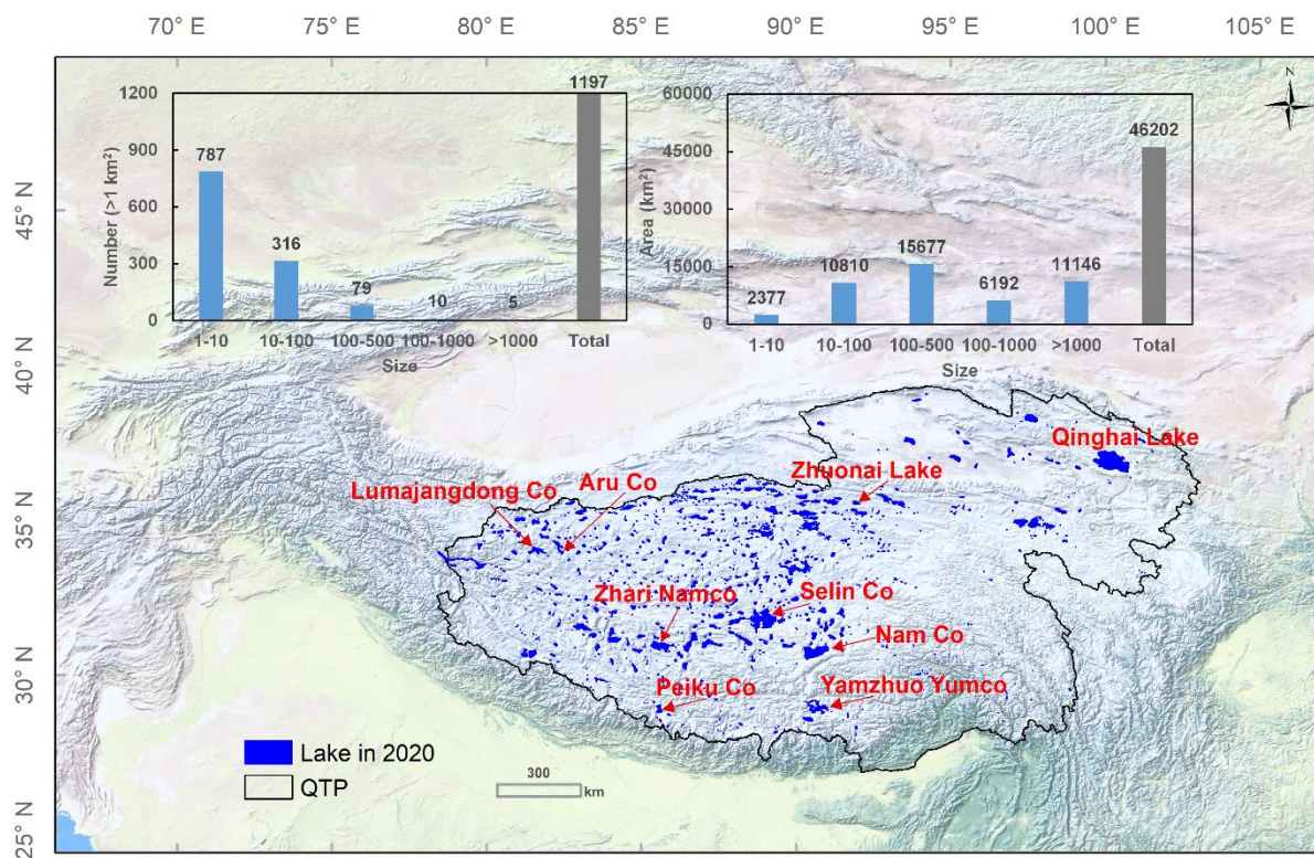
Figure 1. Distribution of lakes over the QTP. Insets show, for lakes larger than 1 km 2 , the number and area of lakes in different size ranges and the total number and area (status: 2020). The names refer to the lakes presented as examples in Figure 7. The background of this figure is from Natural Earth at https://www.naturalearthdata.com .
