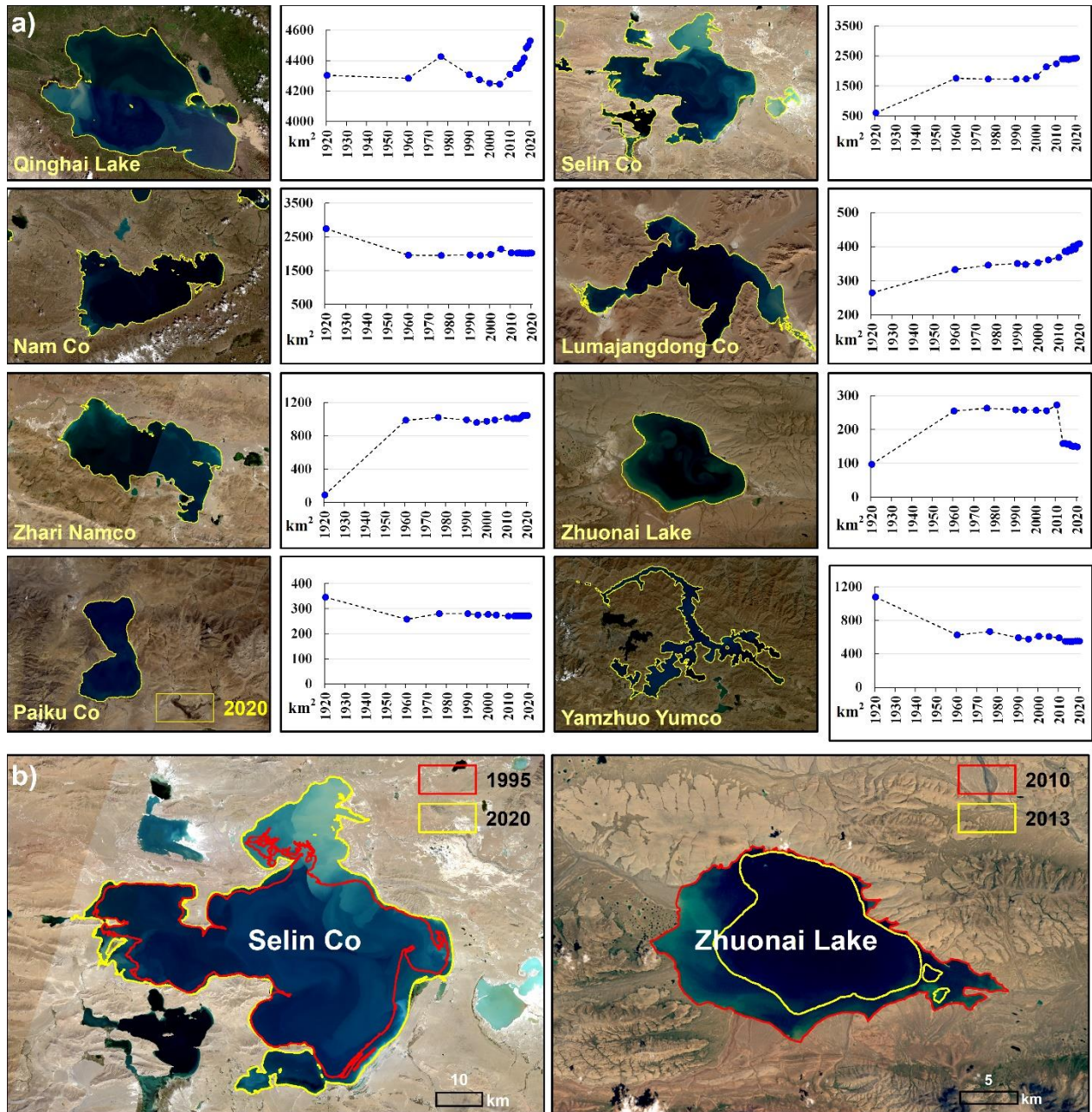
Figure 7. Examples showing the evolution of eight selected lakes from 1920 to 2020, with background of Landsat 285 images (Bands 3, 2, 1 composite). a) Time series of eight selected lake area from 1920 to 2020. b) Images for Selin Co and Zhuonai Lake as examples of rapid lake expansion and rapid shrinkage, respectively. The locations of these lakes are shown in Figure 1.
