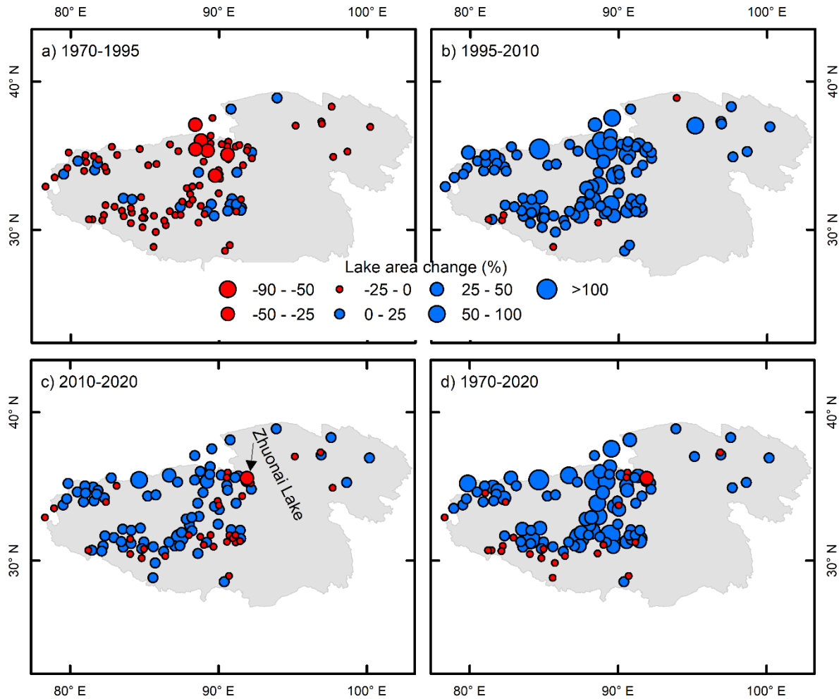
Figure 109. Spatial patterns of lake area changes during the Landsat era. a) 1970–1995. b) 1995–2010. c)
