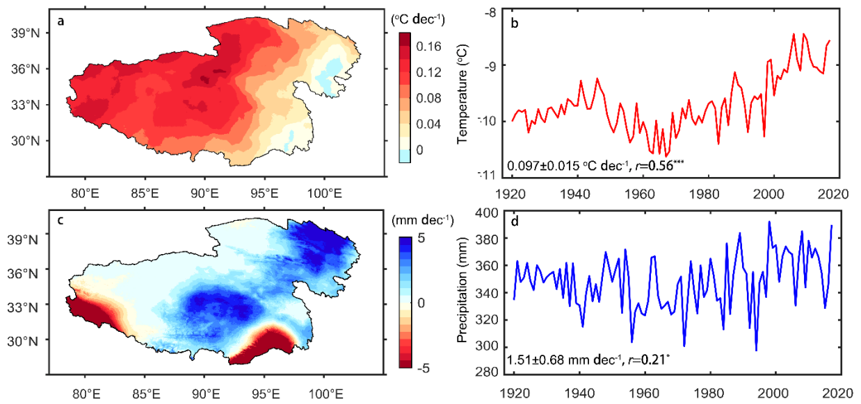
Figure 110. Spatial-temporal variations of temperature and precipitation from 1920 to 2017. a) Spatial pattern of temperature change. b) Time series of temperature change. c) Spatial pattern of precipitation variation. d) Time series of precipitation change.
