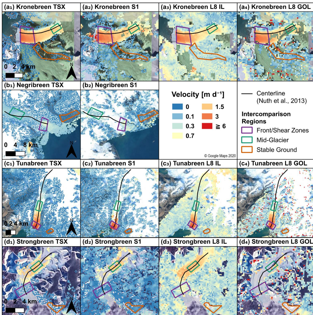
Figure 6: Comparison of scene-pair velocity fields from Sentinel-1, Landsat-8 ITS_LIVE and Landsat-8 GoLIVE with TerraSAR-X over 4 different glaciers in Svalbard. TSX: TerraSAR-X, S1: Sentinel-1, L8 IL: Landsat-8 ITS_LIVE, L8 GOL: Landsat-8 GoLIVE. The dates of acquisition are listed in Table 1. Background: © Google Maps 2020
