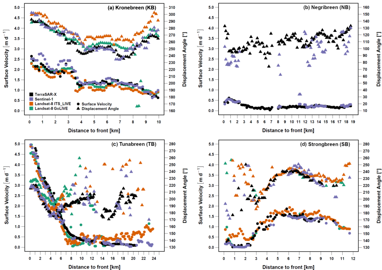
Figure 7: Comparison of velocity and displacement angle profiles from TerraSAR-X, Sentinel-1, Landsat-8 ITS_LIVE and Landsat-8 GoLIVE data sets, extracted along the centerlines of 4 different glaciers in Svalbard. Centerlines are displayed in Fig. 6 and the dates of acquisition are listed in Table 1.
