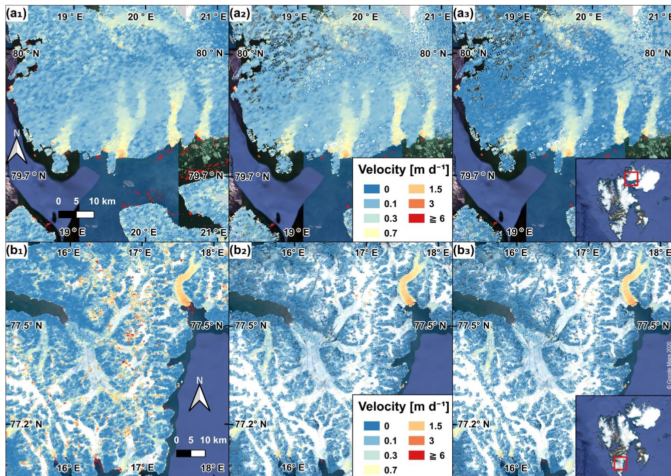
Figure 2: Examples of raw, filtered and corrected single velocity fields. Raw velocity (magnitude) fields from 15 January 2019 (6-day repeat pair, a1 ) and 11 August 2019 (12-day repeat pair, b1 ). Filtered products using the approach of Lüttig et al. (2017) are shown in panels a2 and b2 . The products that were corrected for coregistration errors are displayed in panels a3 and b3 . The short 6-day temporal baseline of the 15 January 2019 velocity field and the absence of surface melt during winter allowed for tracking radar speckle on the almost featureless surface of Vestfonna ice cap. Filtering effectively removed existing blunders while keeping reliable measurements in both examples. While coregistration error correction significantly improved the velocity field on Vestfonna ( a3 ), it had only minor effects on the velocities from 11 August 2019 ( b3 ) due to abundant ice free area in this scene. The coregistration error correction values applied to both velocity fields are shown in Fig. 3. Background: © Google Maps 2020.
