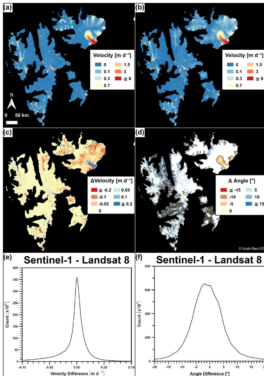
Figure 9: Comparison of a Sentinel-1 surface velocity mosaic with a Landsat-8 ITS_LIVE velocity mosaic from 2018. a) Sentinel-1 weighted mean of the velocity magnitude, b) Landsat-8 weighted mean of the velocity magnitude, c) velocity magnitude difference (Sentinel-1 minus Landsat-8) d) displacement angle difference in regions with surface velocities of > 0.3 \text{ m d}^{-1} (Sentinel-1 minus Landsat-8) e) distribution of the velocity differences, f) distribution of the displacement angle differences. Background: © Google Maps 2020, overlain by an OpenStreetMap-based ocean polygon data set in black ( https://osmdata.openstreetmap.de/data/water-polygons.html ), © OpenStreetMap contributors 2019. Distributed under the Open Data Commons Open Database License (ODbL) v1.0).
