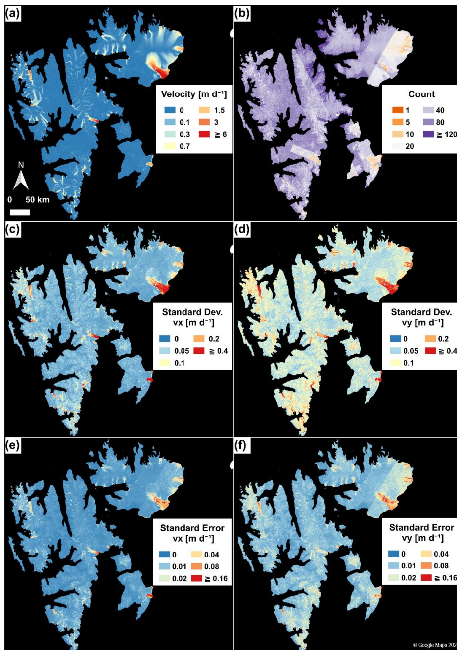
Figure 8: Sentinel-1 surface velocity mosaic generated from 557 scene-pair velocity fields with a 2019 time stamp. a) velocity magnitude, b) measurement count per pixel, c) weighted standard deviation of the x velocity component, d) weighted standard deviation of the y velocity component, e) weighted standard error of the x velocity component, f) weighted standard error of the y velocity component. Background: © Google Maps 2020, overlain by an OpenStreetMap-based ocean polygon data set in black
