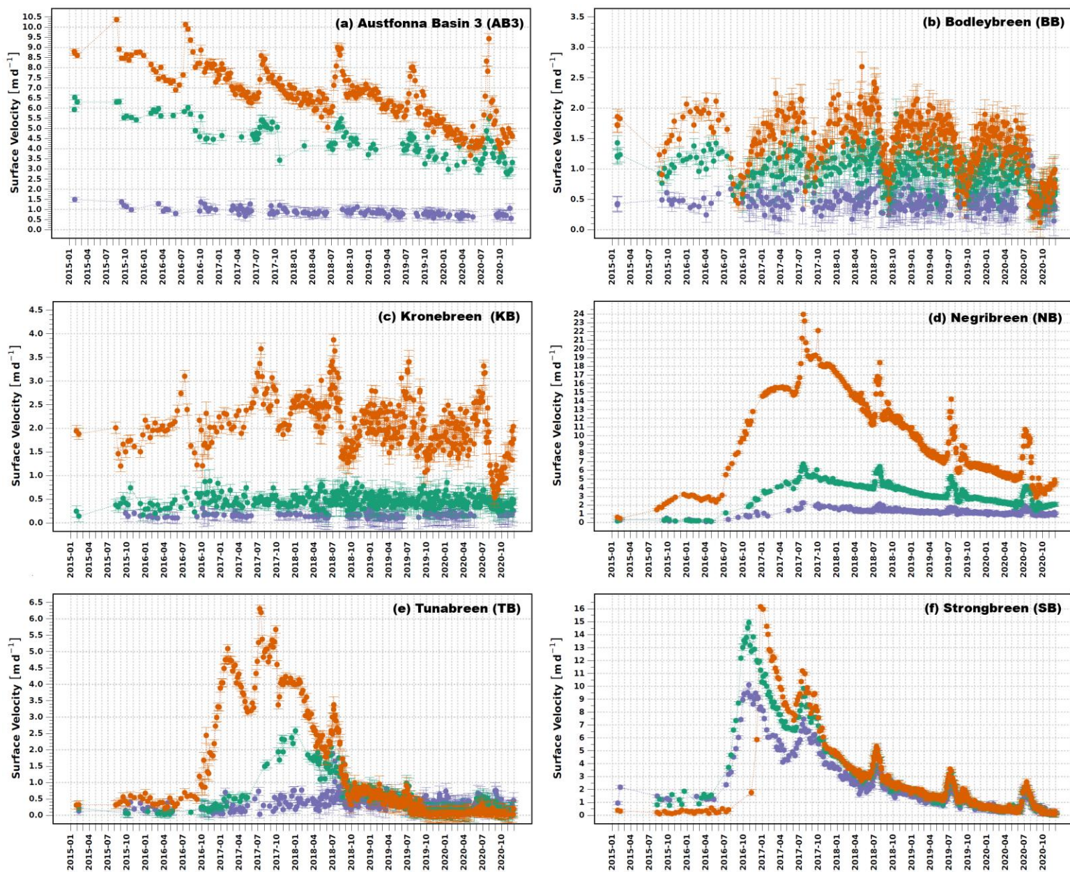
Figure 5: Velocity time series from Sentinel-1 (1 January 2015–30 November 2020) for 6 different glaciers in Svalbard. The color coding is the same as for the corresponding extraction points in Fig. 4.
