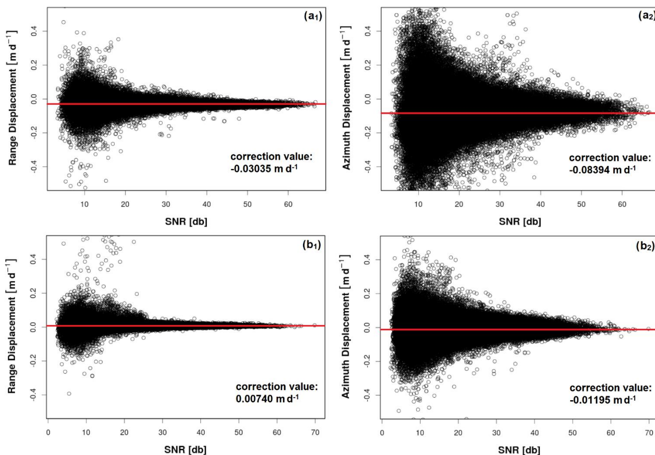
Figure 3: Determination of coregistration error correction values. Coregistration error correction values in az and r direction are shown for the velocity fields from 15 January 2019 ((a 1 ) and (a 2 )) and 11 August 2019 ((b 1 ) and (b 2 )) displayed in Fig. 2. Black circles represent displacement values extracted over stable ground, plotted against their corresponding SNR (Signal to Noise Ratio) values, computed as SNR = CCP/CCS . The median displacement values (red lines) coincide well with the displacement values that have the highest SNR values (i.e. the most reliable measurements, assumed to be primarily affected by coregistration inaccuracy). After correction, median displacement values are 0 for both directions.
