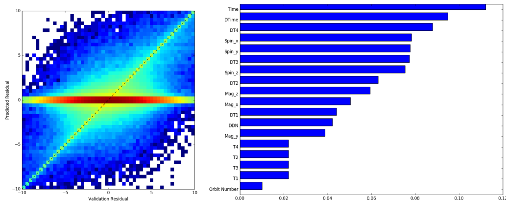
Figure C1. (left) Heatmap of the predicted C_{sp} residuals (vertical axis) against the observed ones (horizontal axis), colored in log-scale. (right) Rank of importance of different parameters.
