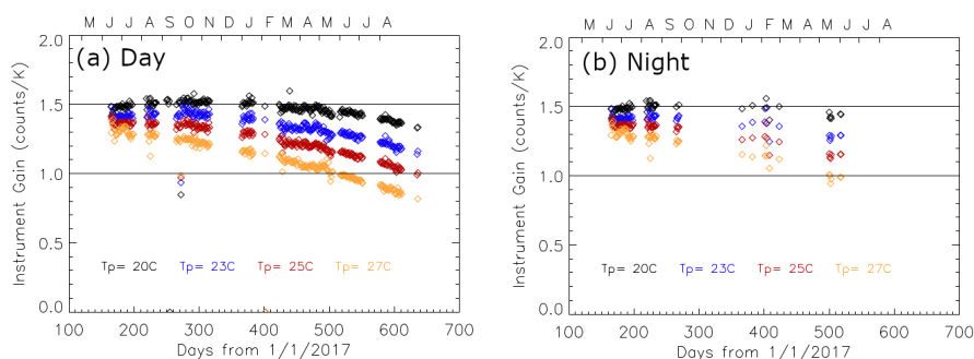
Figure 5. Time series of daily gain for (a) daytime and (b) nighttime when T_{p4} value equals to 20^\circ\text{C} (black), 23^\circ\text{C} (blue), 25^\circ\text{C} (red), and 27^\circ\text{C} (orange). The gain declines consistently with increasing of instrument temperature.
