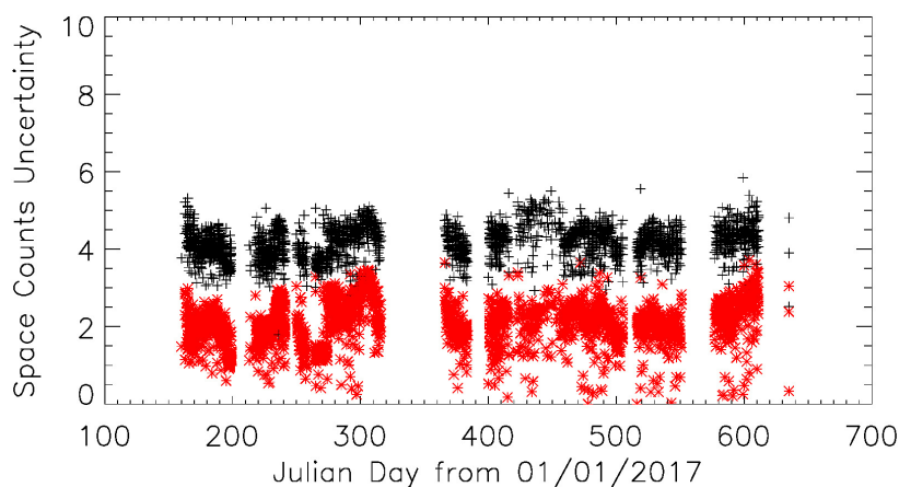
Figure 4. Time series of \sigma_{sp} before the ML/AI model fitting (black crosses) and after the fitting (red crosses). Each cross represent one orbit.
