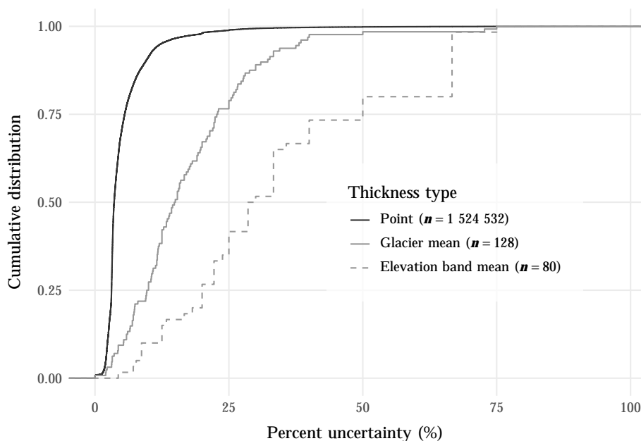
Figure 11. Cumulative distribution of percent ice thickness uncertainties ( 100\% \times \text{uncertainty}/\text{thickness} ) by thickness type: point (solid black line), glacier mean (grey solid line), and elevation band mean (dashed grey line). For example, about three quarters of glacier mean thicknesses report uncertainties of 25 % of the thickness or better.
