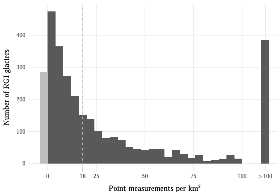
Figure 7. Number of RGI glaciers with point measurements in GlaThiDa by the average number of point measurements per km 2 . The median (18 points per km 2 ) is marked with a grey dashed line. Glaciers with a mean or maximum thickness but no point measurements are shown in the grey bar to the left of 0 per km 2 .
