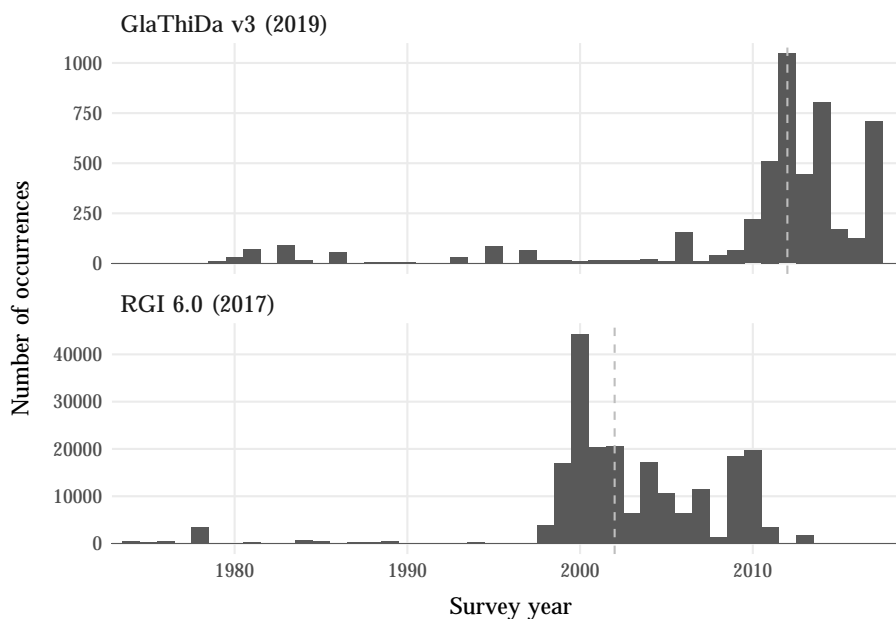
Figure 10. Comparison of the distribution of survey years between GlaThiDa (top) and RGI (bottom). Medians are marked with grey dashed lines. Only survey years since 1975 are shown.
